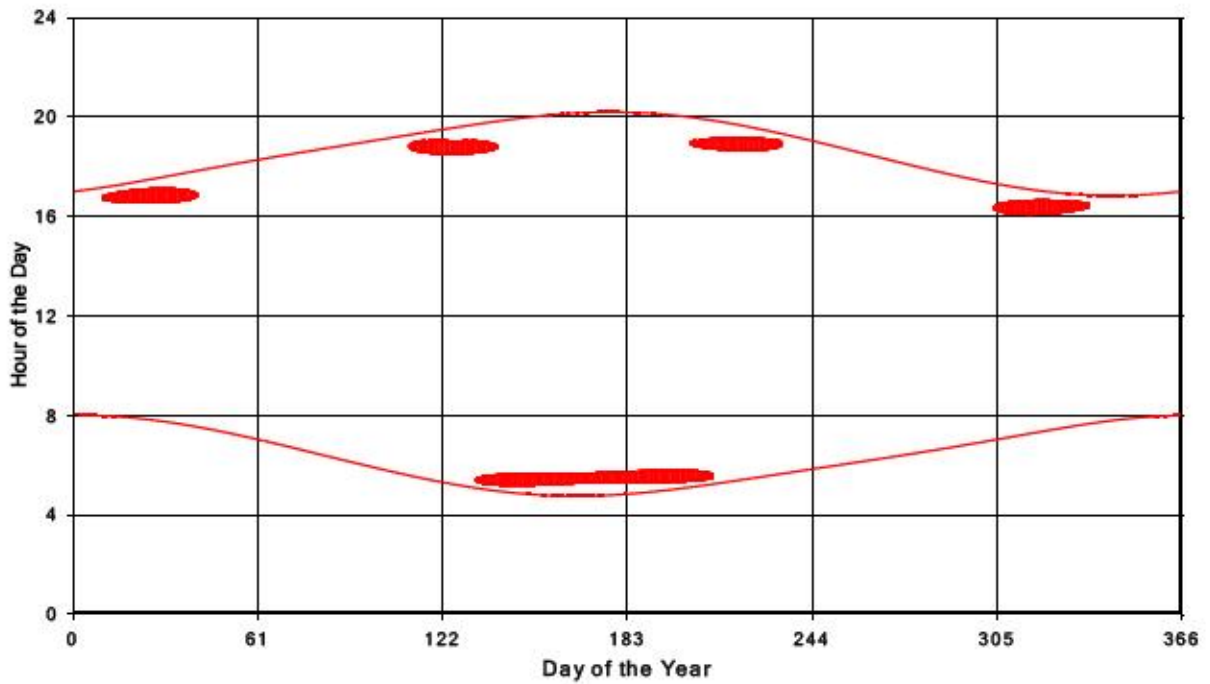
Bluewater Wind Energy Centre Shadow Times on Receptor 381, All Windows from All Turbine
