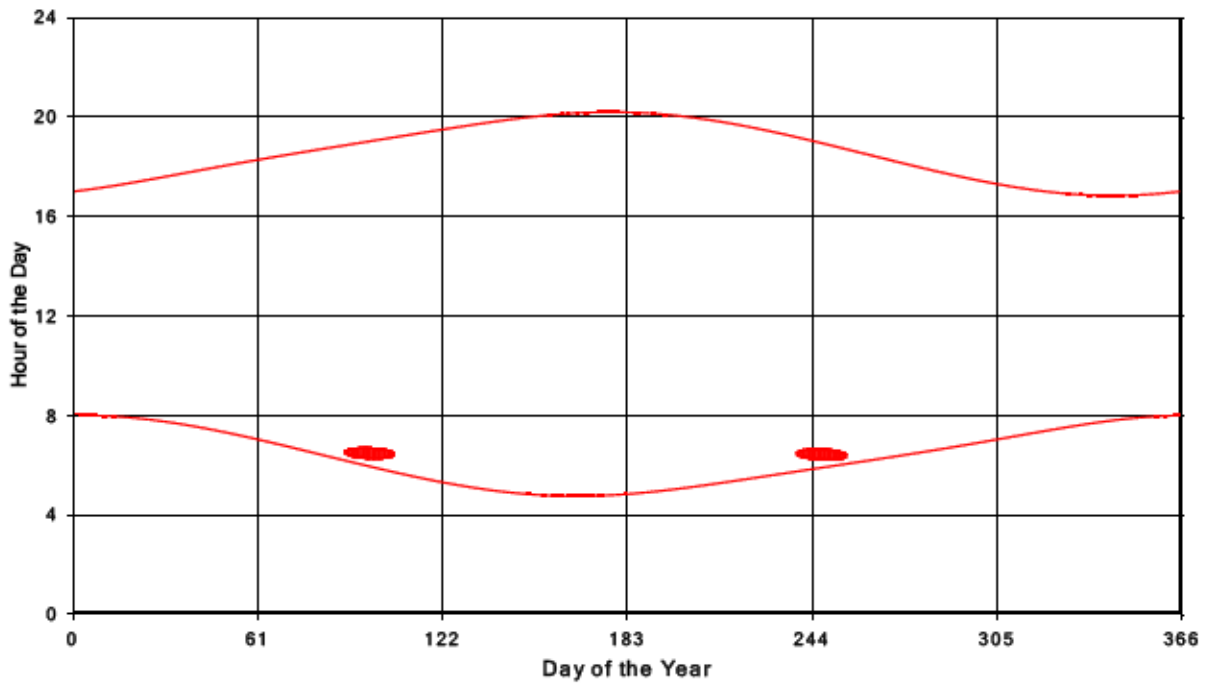
Bluewater Wind Energy Centre Shadow Times on Receptor 332, All Windows from All Turbine
