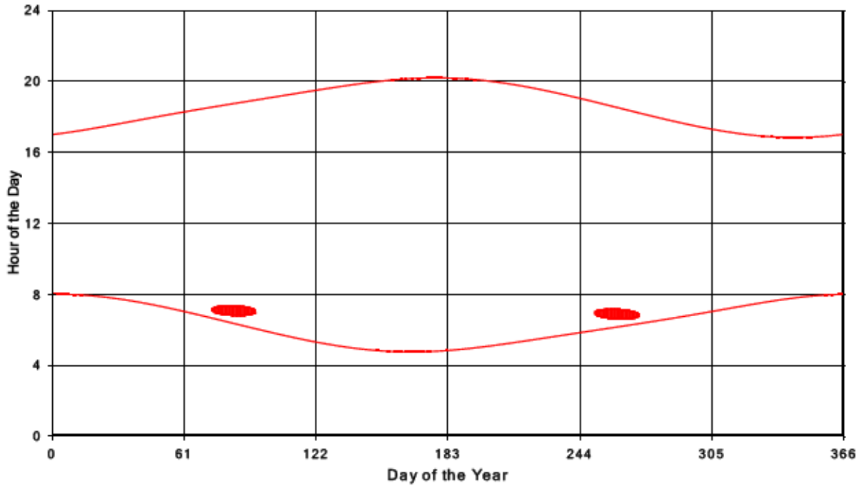
Bluewater Wind Energy Centre Shadow Times on Receptor 195, All Windows from All Turbine
