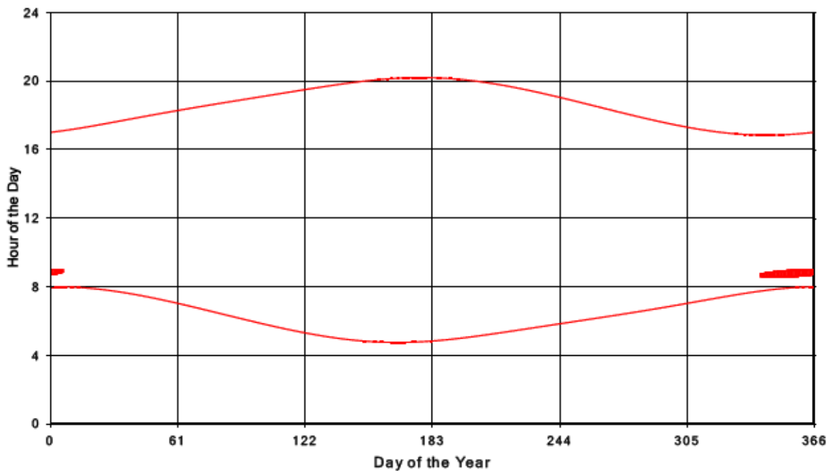
Bluewater Wind Energy Centre Shadow Times on Receptor 124, All Windows from All Turbine
