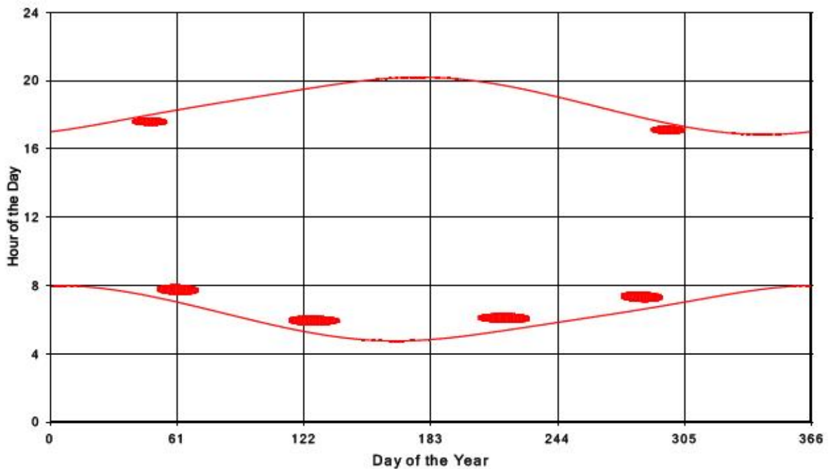
Bluewater Wind Energy Centre Shadow Times on Receptor 259, All Windows from All Turbine
