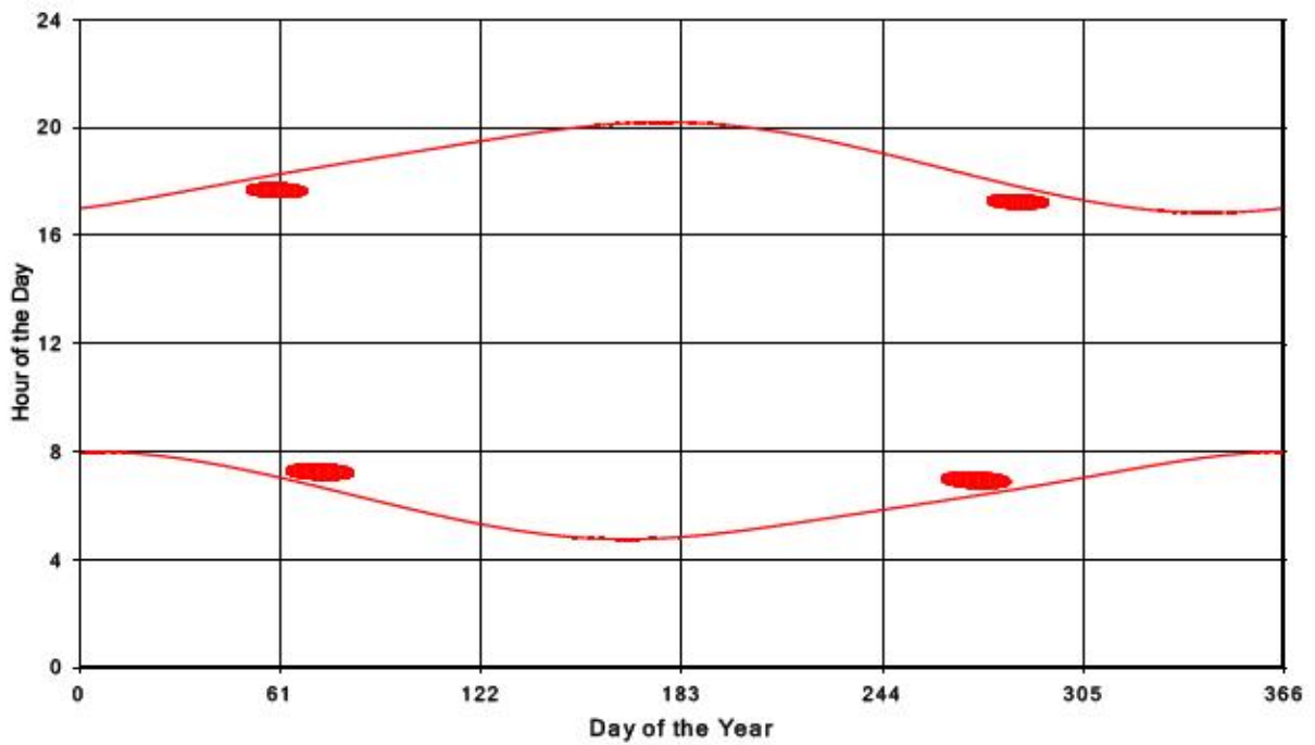
Bluewater Wind Energy Centre Shadow Times on Receptor 138, All Windows from All Turbine
