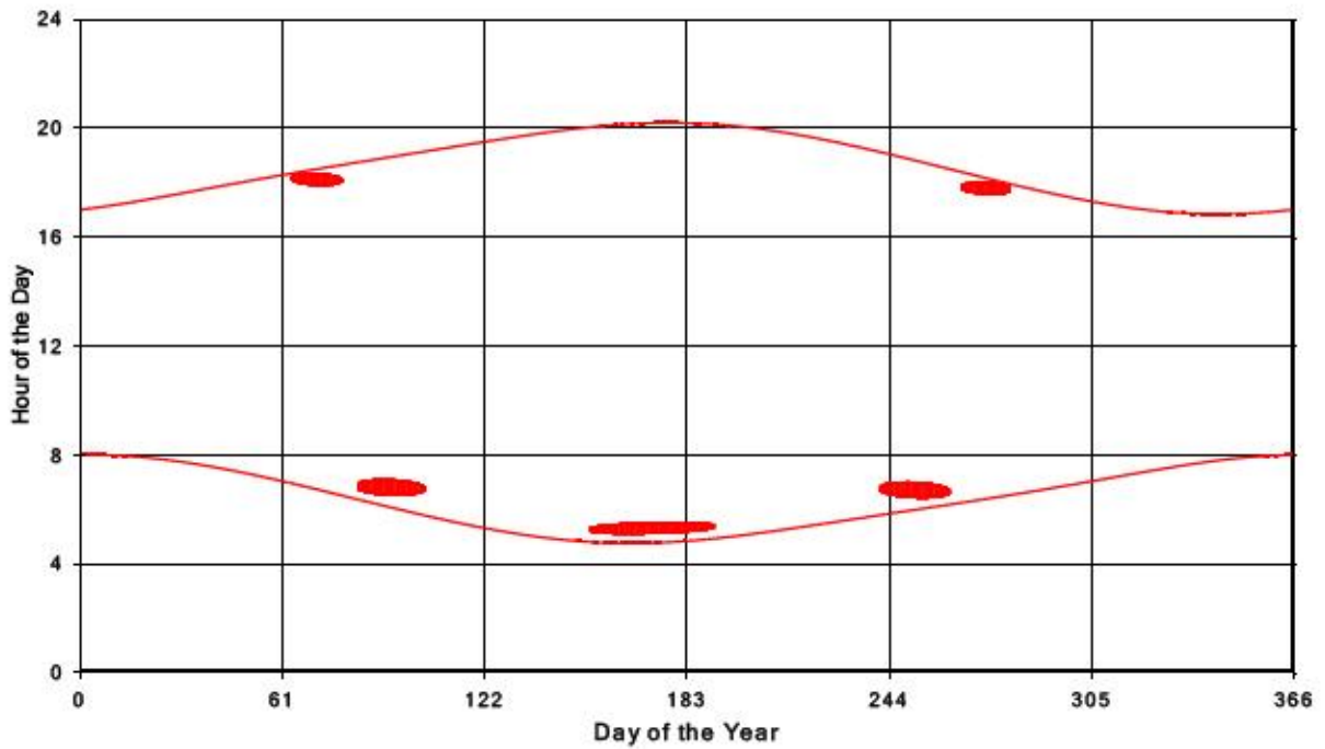
Bluewater Wind Energy Centre Shadow Times on Receptor 260, All Windows from All Turbine
