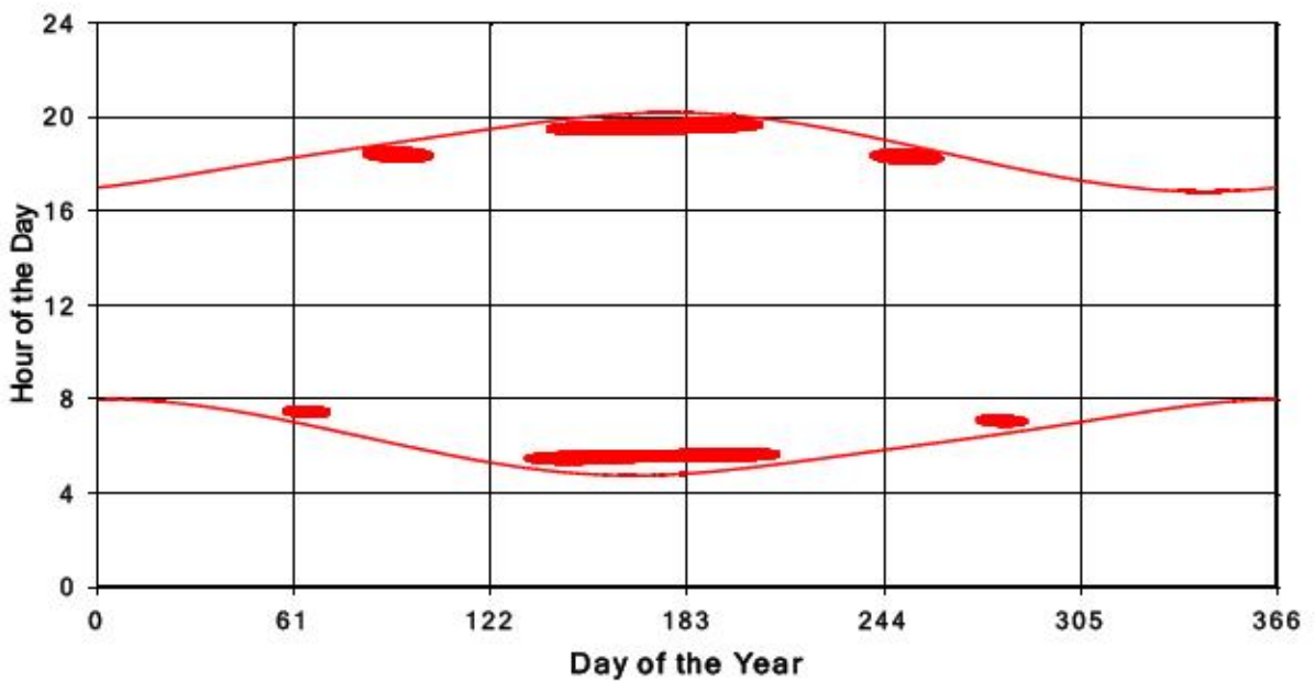
Bluewater Wind Energy Centre Shadow Times on Receptor 410, All Windows from All Turbine
