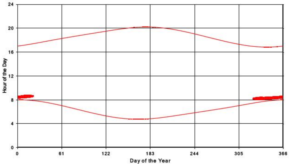
Bluewater Wind Energy Centre Shadow Times on Receptor 119, All Windows from All Turbine
