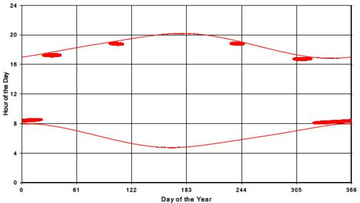
Bluewater Wind Energy Centre Shadow Times on Receptor 214, All Windows from All Turbine
