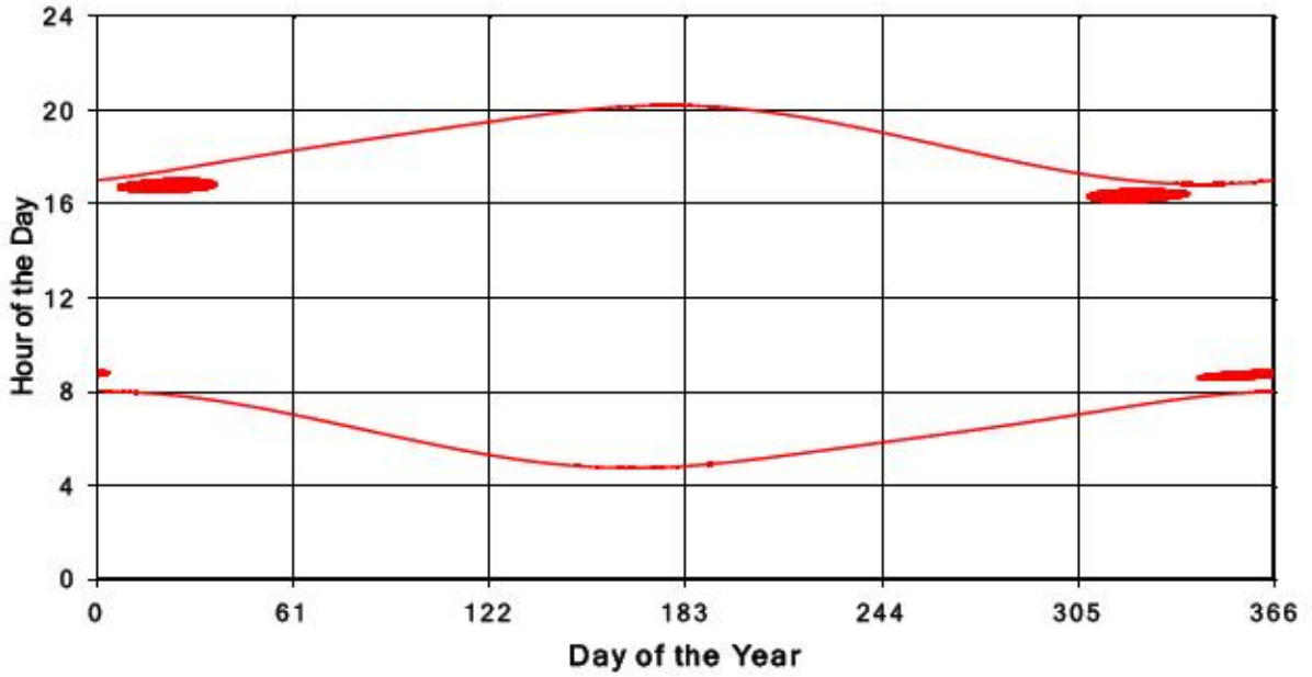
Bluewater Wind Energy Centre Shadow Times on Receptor 232, All Windows from All Turbine
