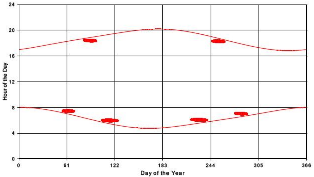
Bluewater Wind Energy Centre Shadow Times on Receptor 367, All Windows from All Turbine
