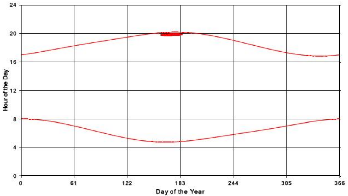
Bluewater Wind Energy Centre Shadow Times on Receptor 77, All Windows from All Turbine:
