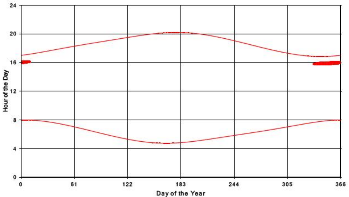
Bluewater Wind Energy Centre Shadow Times on Receptor 136, All Windows from All Turbine
