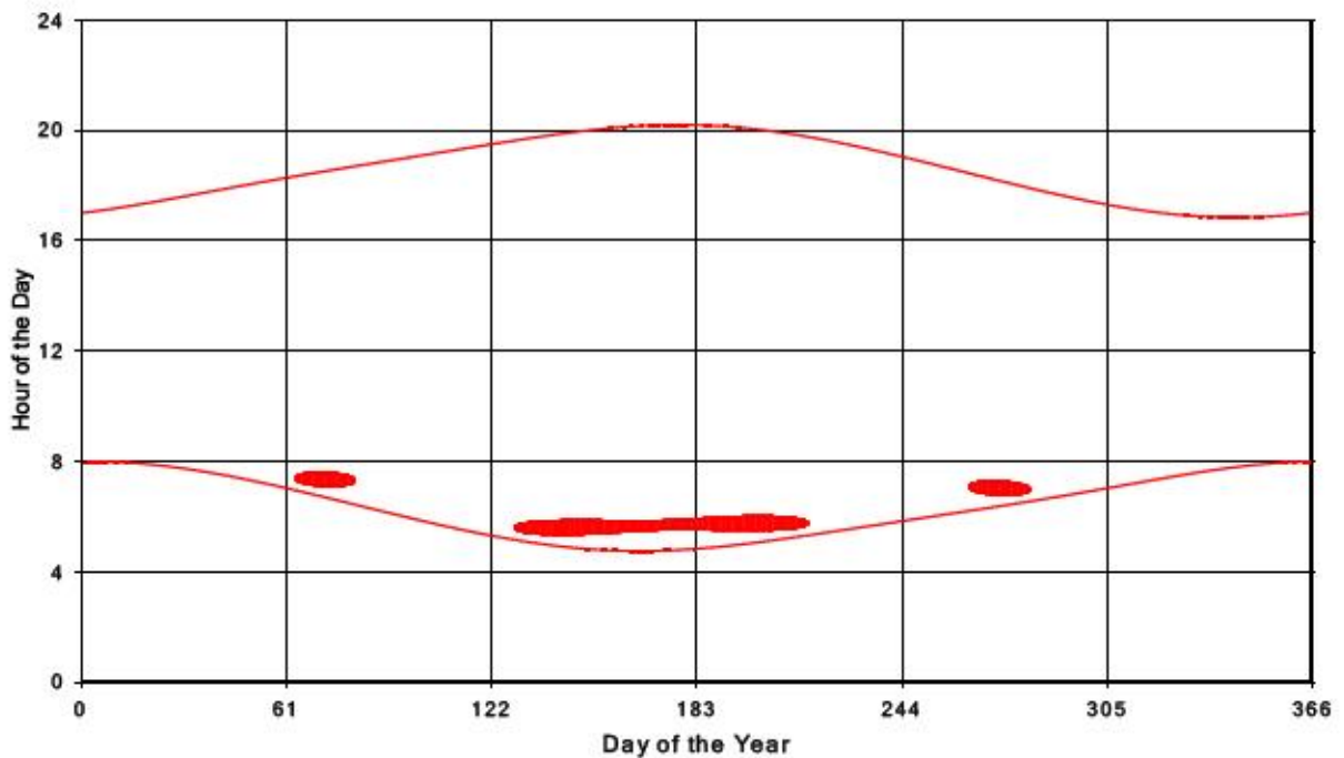
Bluewater Wind Energy Centre Shadow Times on Receptor 340, All Windows from All Turbine
