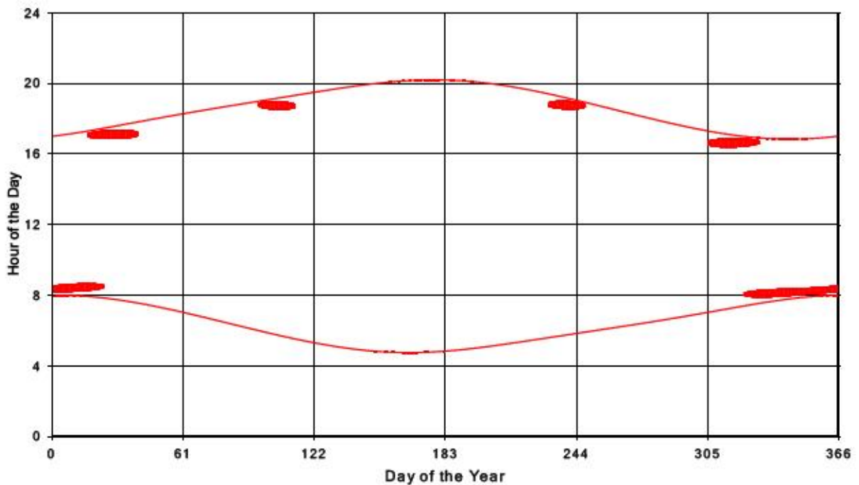
Bluewater Wind Energy Centre Shadow Times on Receptor 212, All Windows from All Turbine
