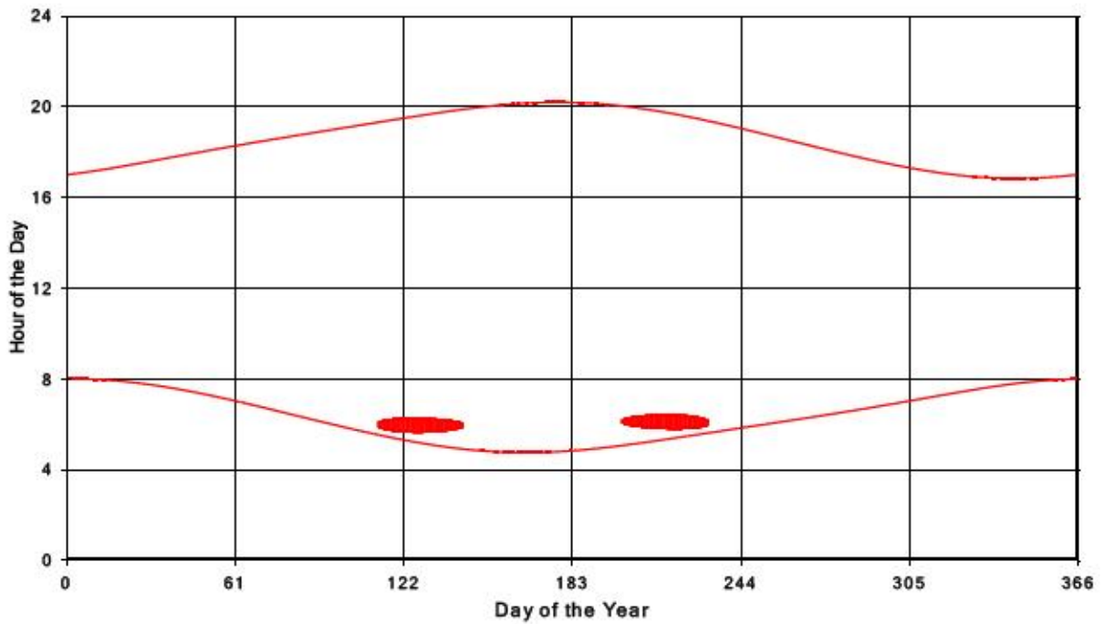
Bluewater Wind Energy Centre Shadow Times on Receptor 358, All Windows from All Turbine
