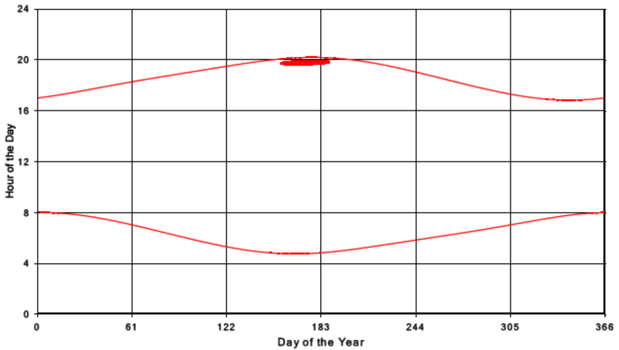
Bluewater Wind Energy Centre Shadow Times on Receptor 185, All Windows from All Turbine
