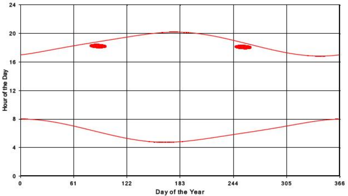
Bluewater Wind Energy Centre Shadow Times on Receptor 240, All Windows from All Turbine
