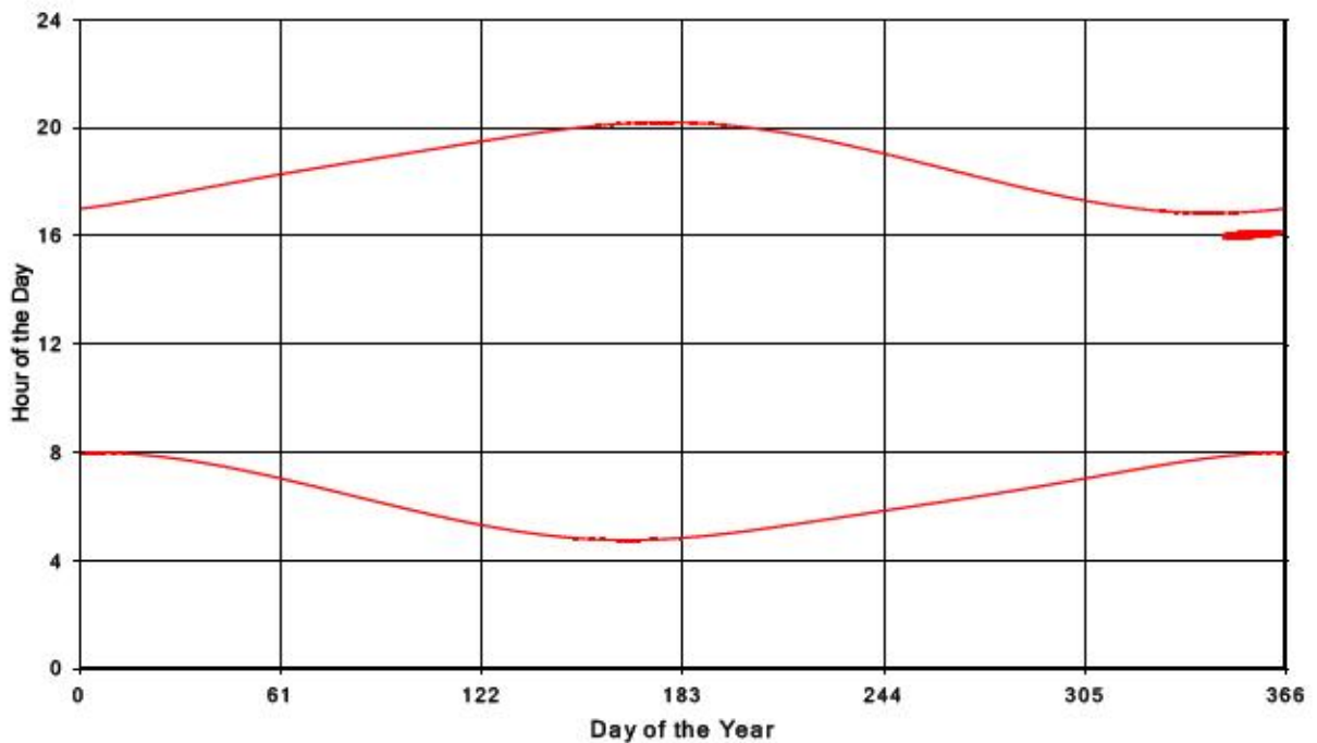
Bluewater Wind Energy Centre Shadow Times on Receptor 198, All Windows from All Turbine
