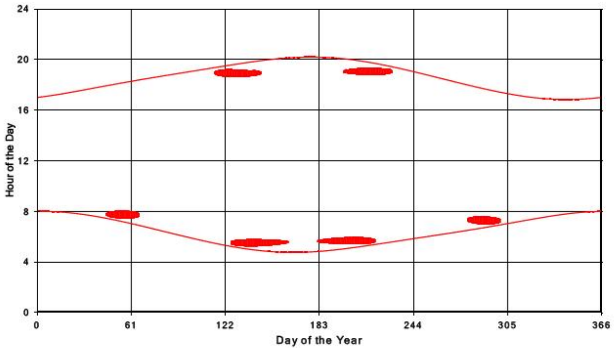
Bluewater Wind Energy Centre Shadow Times on Receptor 243, All Windows from All Turbine
