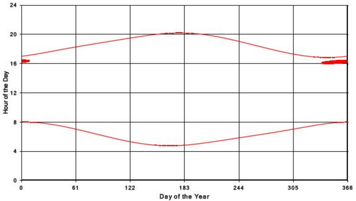
Bluewater Wind Energy Centre Shadow Times on Receptor 49, All Windows from All Turbine:
