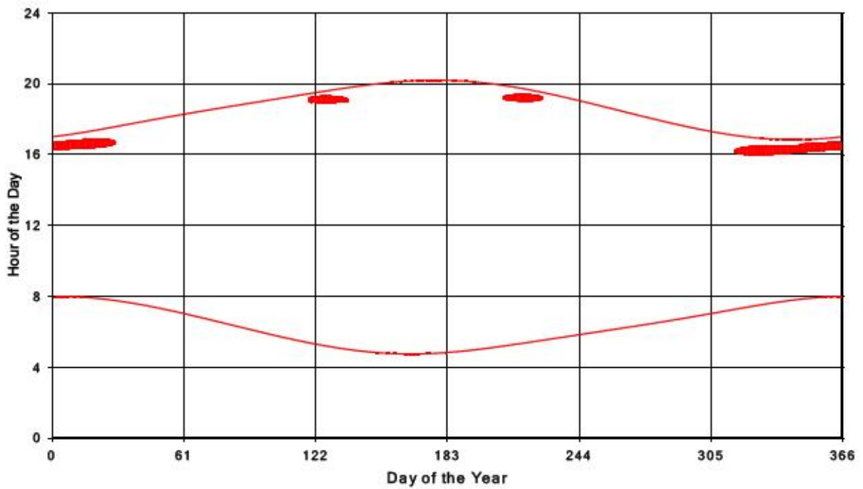
Bluewater Wind Energy Centre Shadow Times on Receptor 390, All Windows from All Turbine
