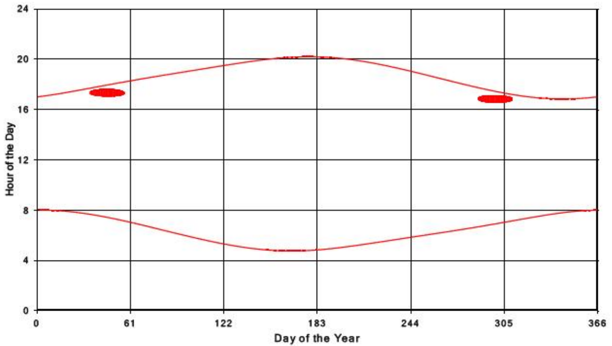
Bluewater Wind Energy Centre Shadow Times on Receptor 391, All Windows from All Turbine
