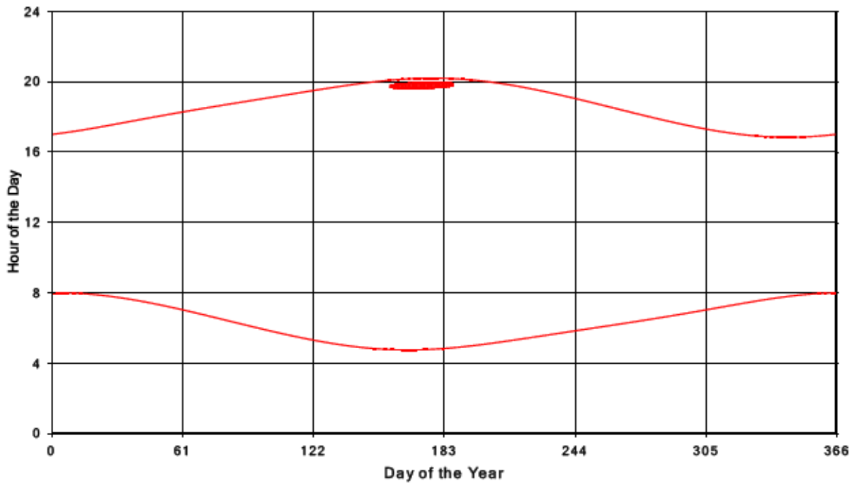
Bluewater Wind Energy Centre Shadow Times on Receptor 184, All Windows from All Turbine
