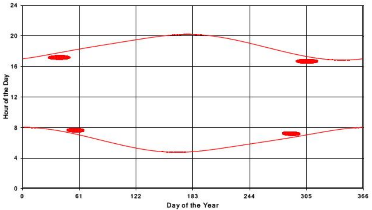
Bluewater Wind Energy Centre Shadow Times on Receptor 137, All Windows from All Turbine
