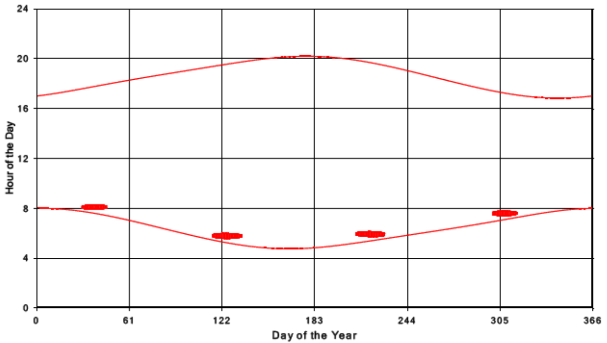
Bluewater Wind Energy Centre Shadow Times on Receptor 326, All Windows from All Turbine
