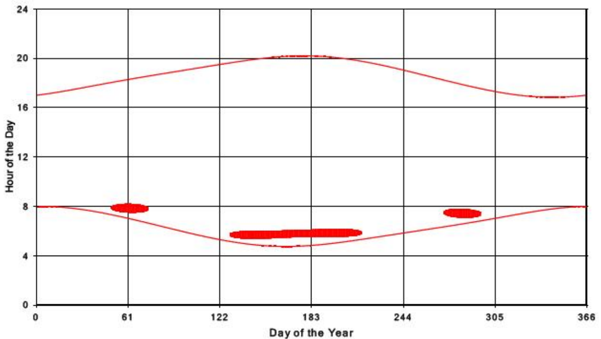
Bluewater Wind Energy Centre Shadow Times on Receptor 201, All Windows from All Turbine
