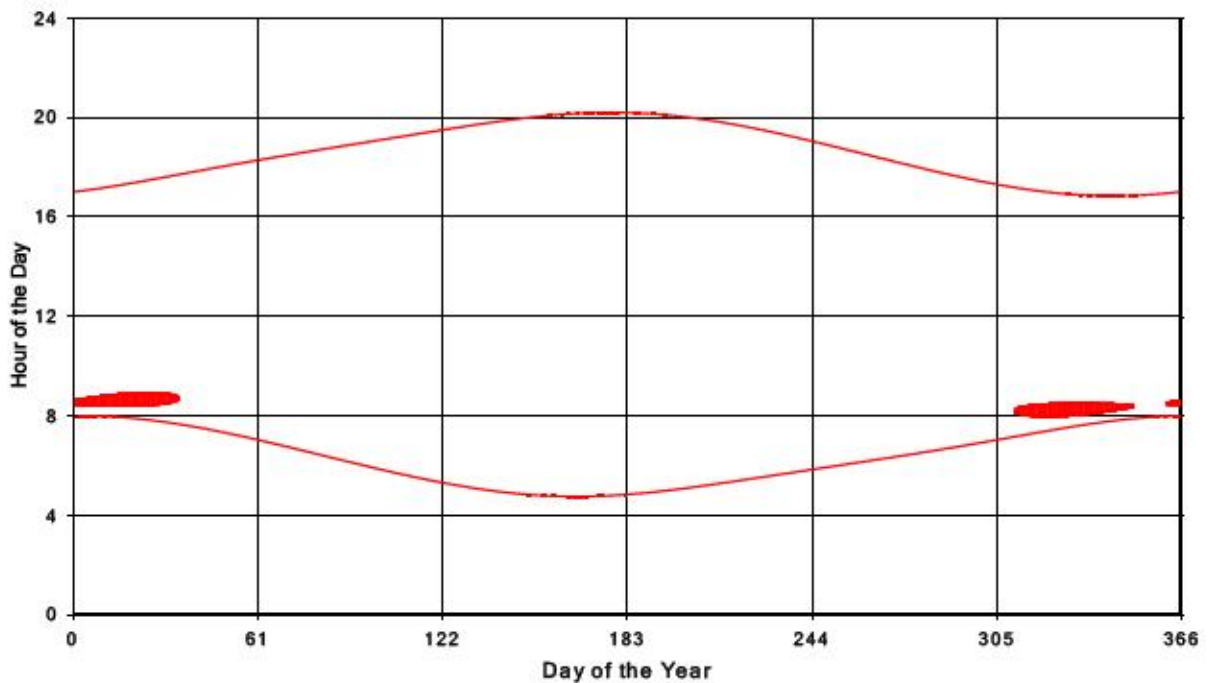
Bluewater Wind Energy Centre Shadow Times on Receptor 219, All Windows from All Turbine
