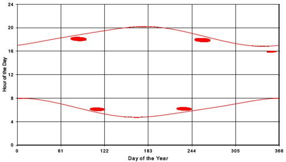
Bluewater Wind Energy Centre Shadow Times on Receptor 380, All Windows from All Turbine
