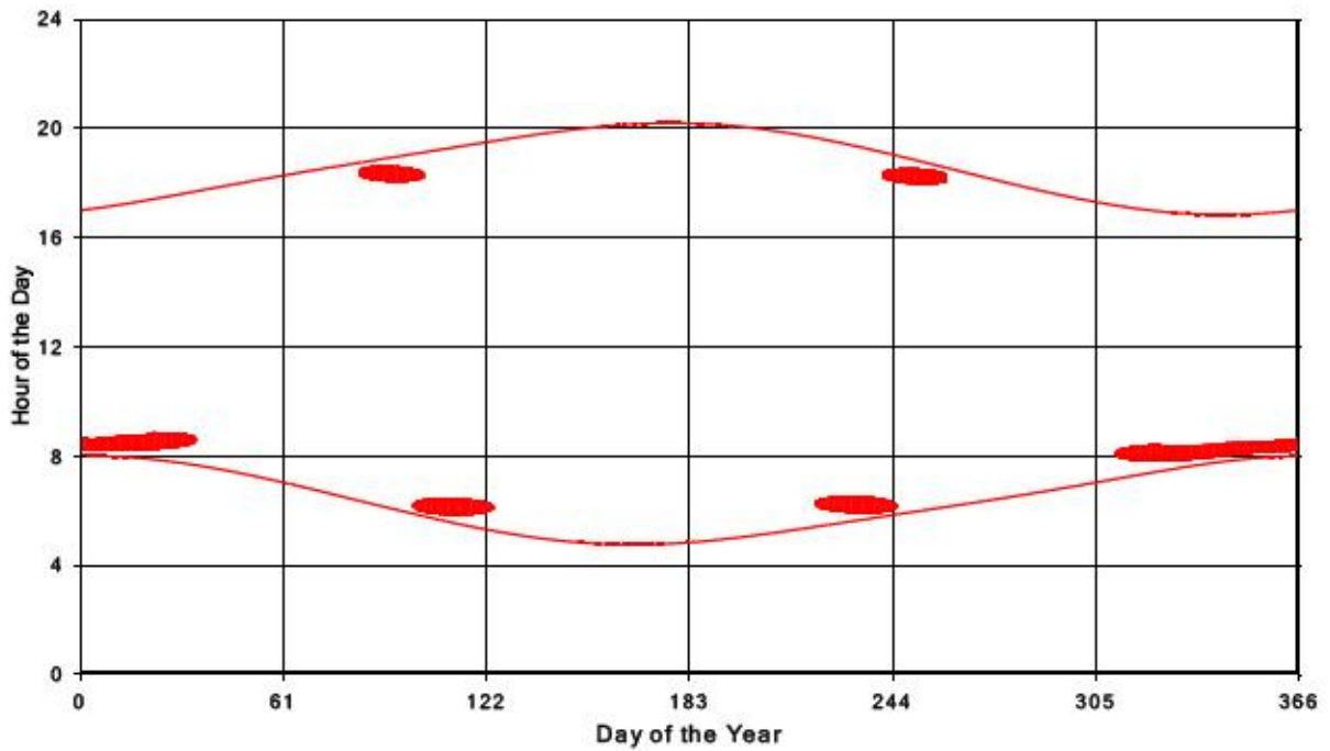
Bluewater Wind Energy Centre Shadow Times on Receptor 245, All Windows from All Turbine
