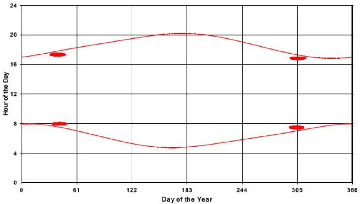
Bluewater Wind Energy Centre Shadow Times on Receptor 144, All Windows from All Turbine
