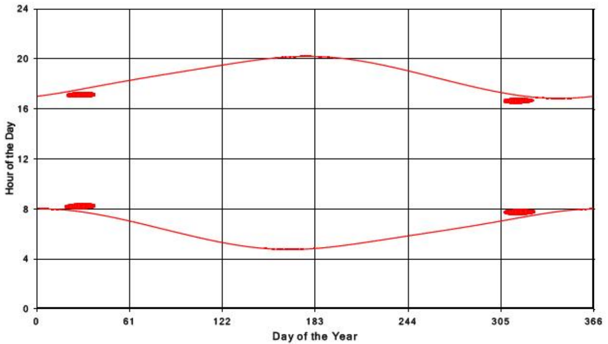
Bluewater Wind Energy Centre Shadow Times on Receptor 145, All Windows from All Turbine
