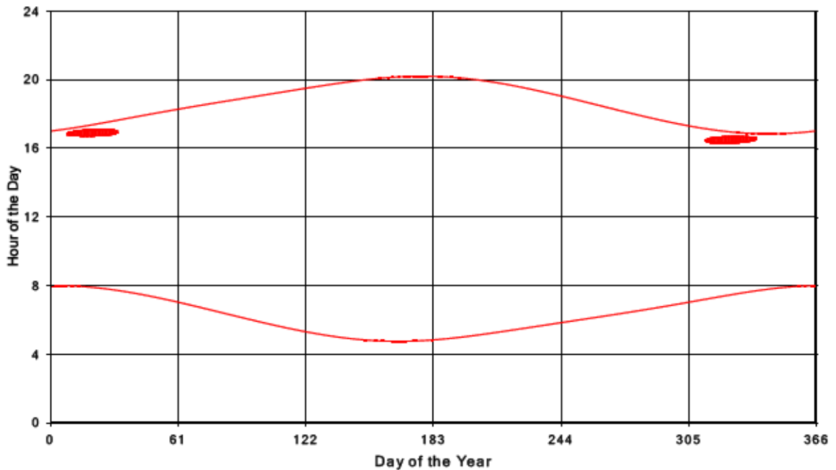
Bluewater Wind Energy Centre Shadow Times on Receptor 131, All Windows from All Turbine
