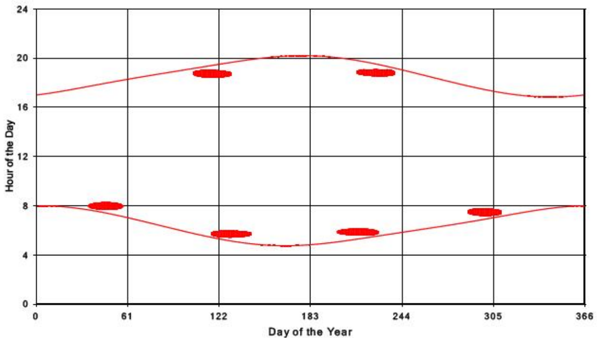
Bluewater Wind Energy Centre Shadow Times on Receptor 242, All Windows from All Turbine
