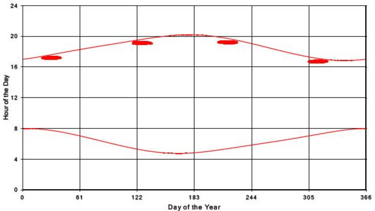
Bluewater Wind Energy Centre Shadow Times on Receptor 75, All Windows from All Turbine:
