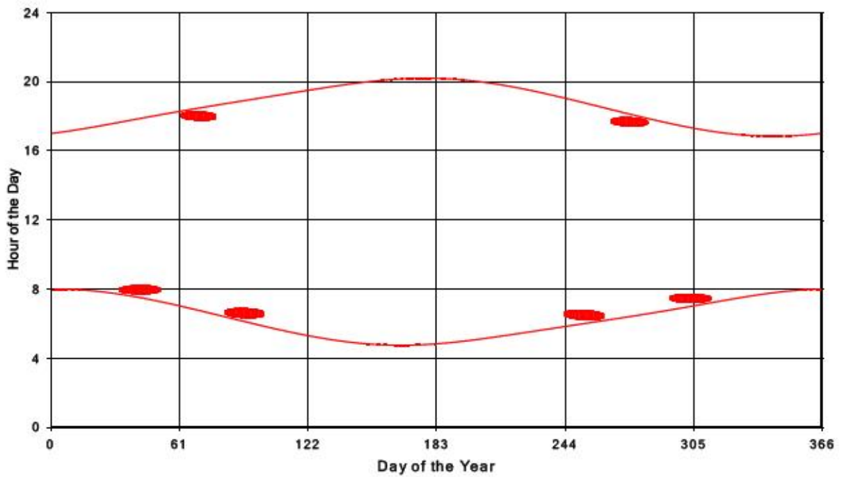
Bluewater Wind Energy Centre Shadow Times on Receptor 114, All Windows from All Turbine
