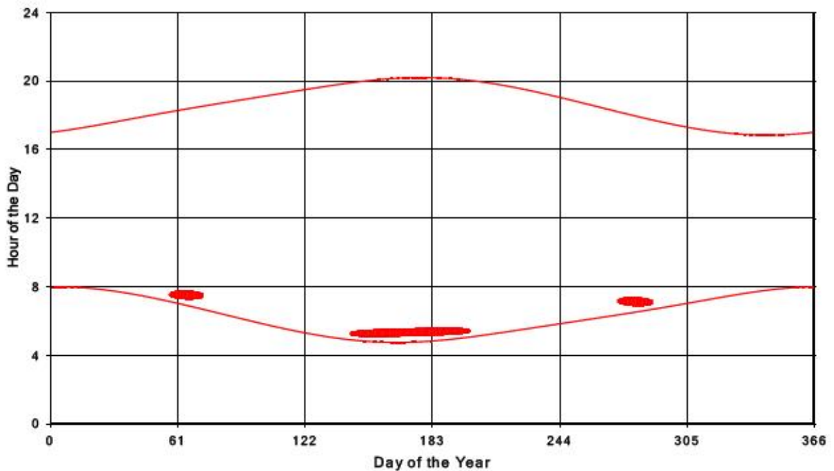
Bluewater Wind Energy Centre Shadow Times on Receptor 34, All Windows from All Turbine:
