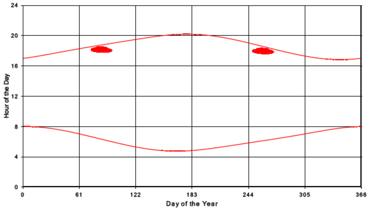
Bluewater Wind Energy Centre Shadow Times on Receptor 168, All Windows from All Turbine
