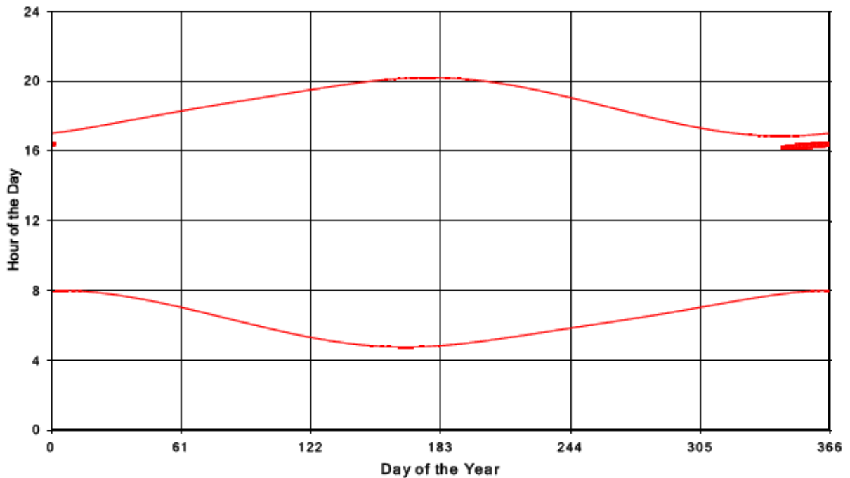
Bluewater Wind Energy Centre Shadow Times on Receptor 58, All Windows from All Turbine:
