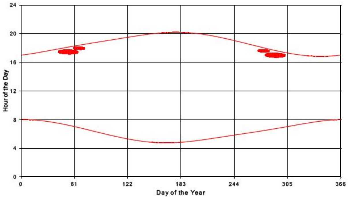
Bluewater Wind Energy Centre Shadow Times on Receptor 309, All Windows from All Turbine
