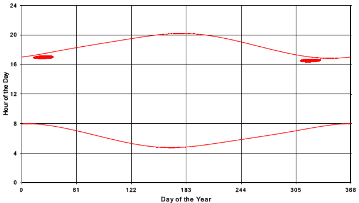
Bluewater Wind Energy Centre Shadow Times on Receptor 187, All Windows from All Turbine
