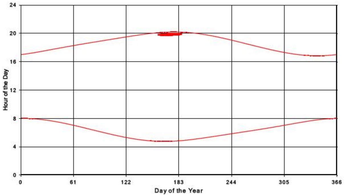
Bluewater Wind Energy Centre Shadow Times on Receptor 199, All Windows from All Turbine
