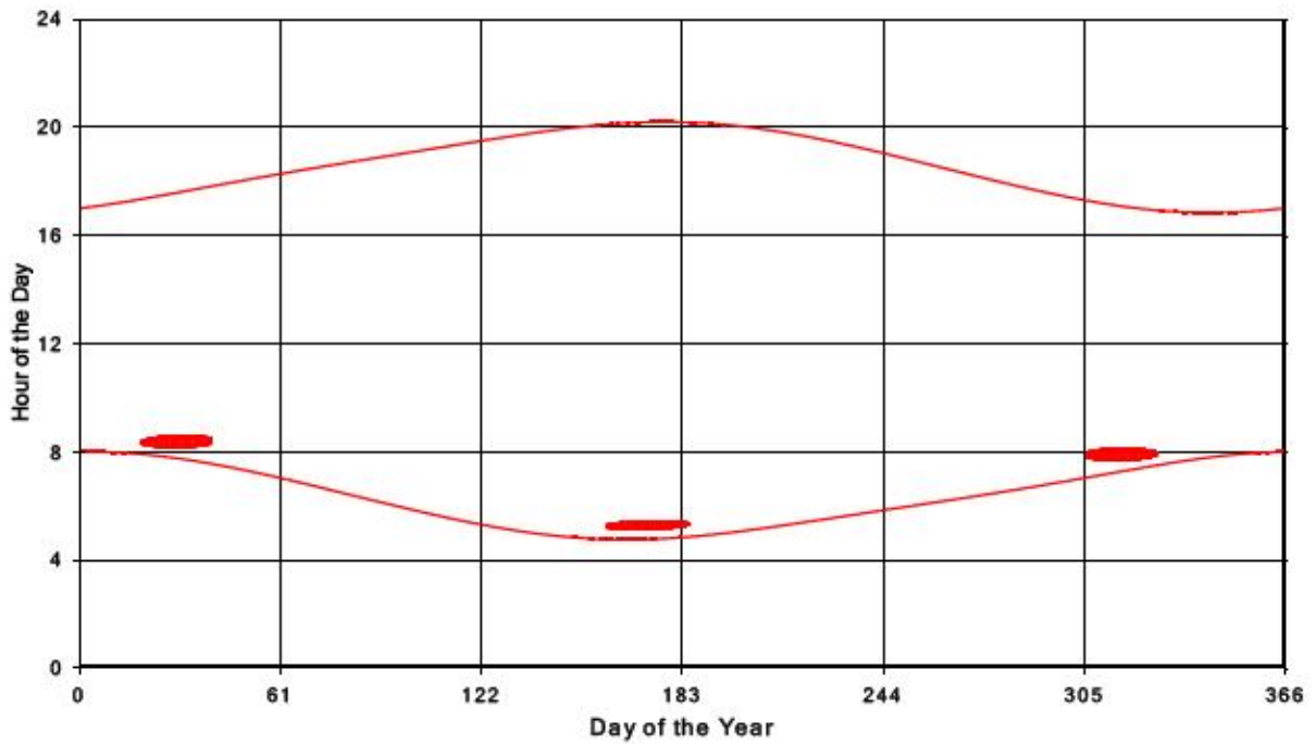
Bluewater Wind Energy Centre Shadow Times on Receptor 17, All Windows from All Turbine:
