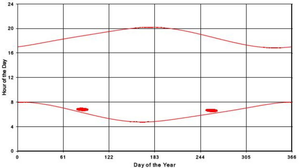
Bluewater Wind Energy Centre Shadow Times on Receptor 331, All Windows from All Turbine
