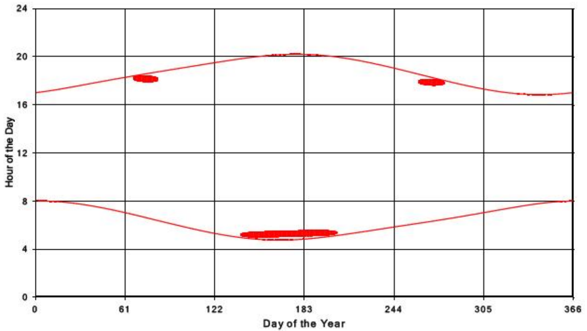
Bluewater Wind Energy Centre Shadow Times on Receptor 99, All Windows from All Turbine:
