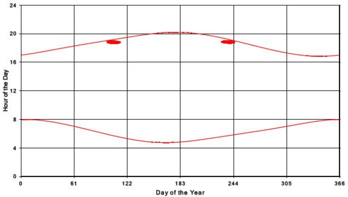
Bluewater Wind Energy Centre Shadow Times on Receptor 78, All Windows from All Turbine:
