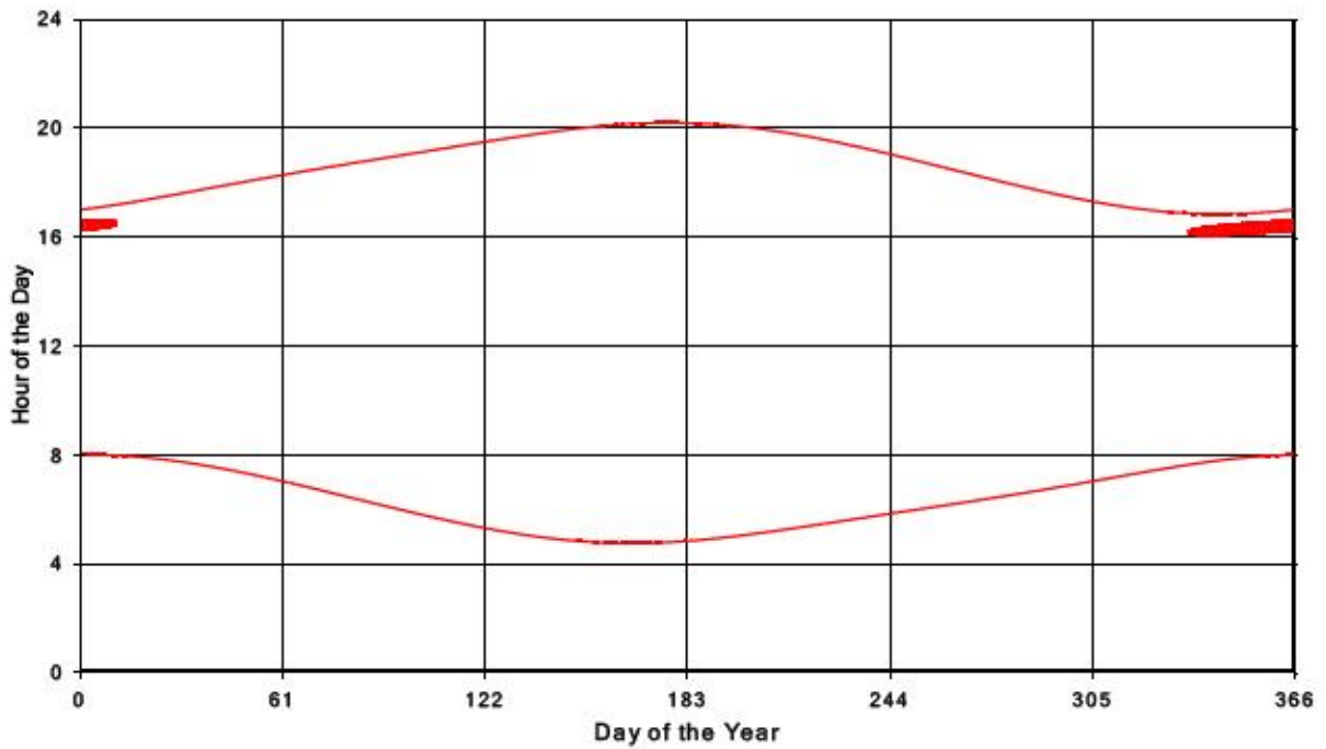
Bluewater Wind Energy Centre Shadow Times on Receptor 262, All Windows from All Turbine
