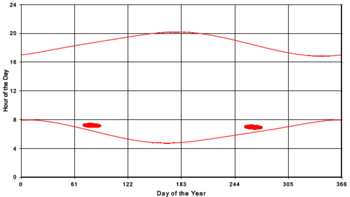
Bluewater Wind Energy Centre Shadow Times on Receptor 196, All Windows from All Turbine
