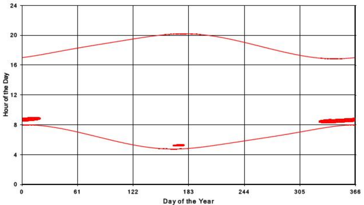
Bluewater Wind Energy Centre Shadow Times on Receptor 408, All Windows from All Turbine
