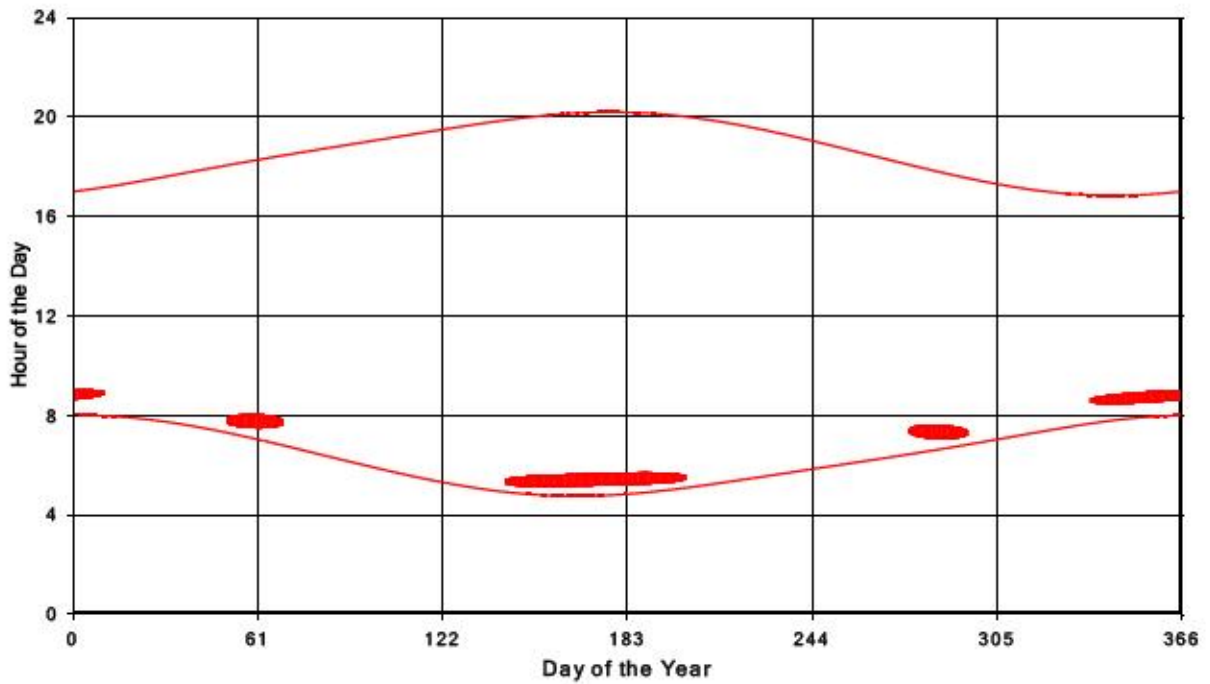
Bluewater Wind Energy Centre Shadow Times on Receptor 387, All Windows from All Turbine
