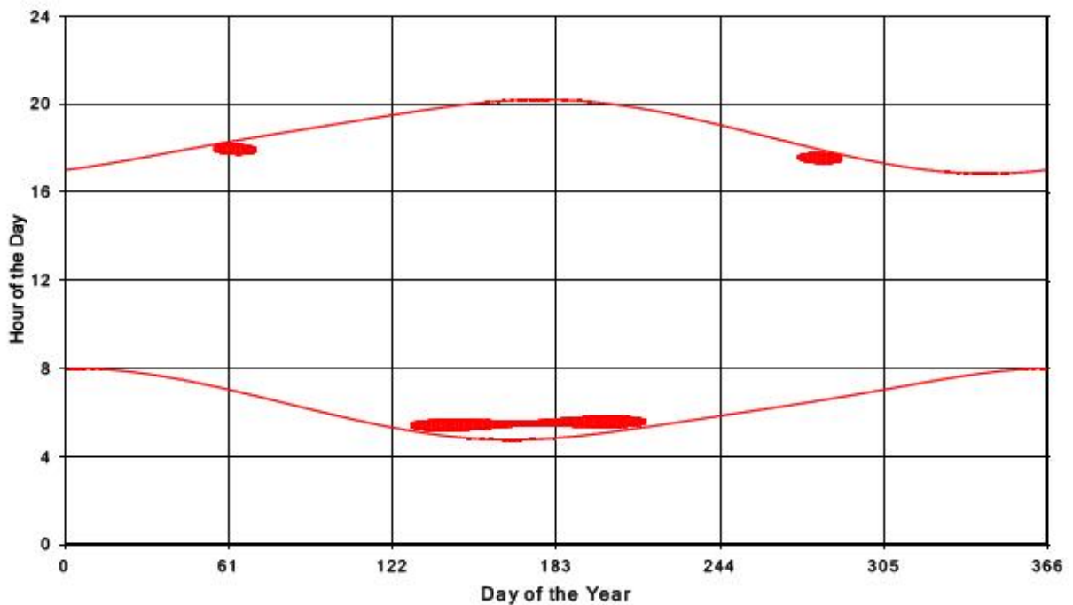
Bluewater Wind Energy Centre Shadow Times on Receptor 362, All Windows from All Turbine
