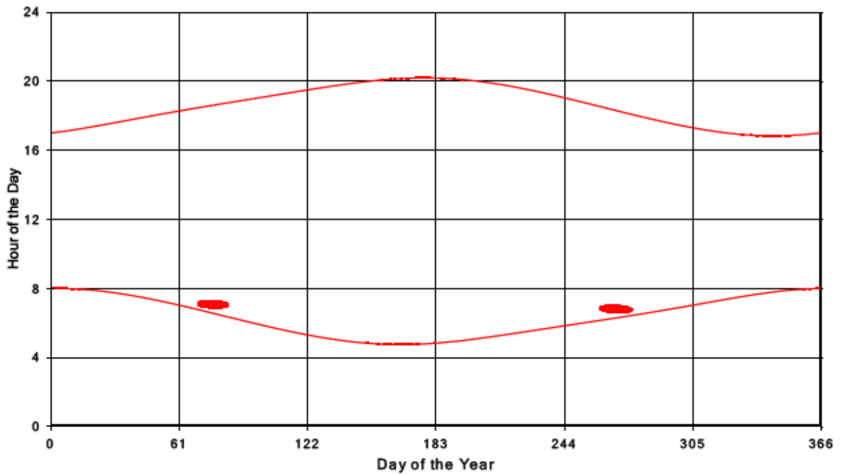
Bluewater Wind Energy Centre Shadow Times on Receptor 7, All Windows from All Turbine:
