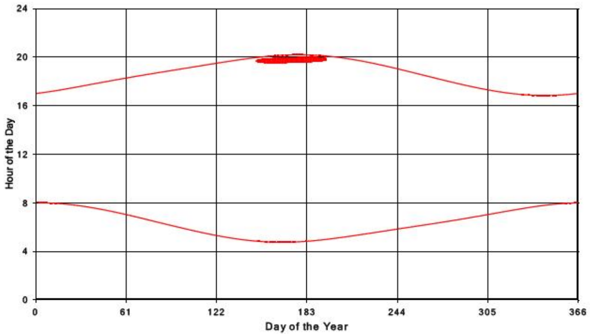
Bluewater Wind Energy Centre Shadow Times on Receptor 81, All Windows from All Turbine:
