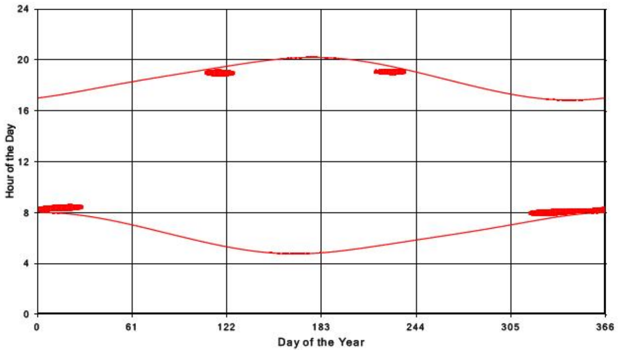
Bluewater Wind Energy Centre Shadow Times on Receptor 218, All Windows from All Turbine
