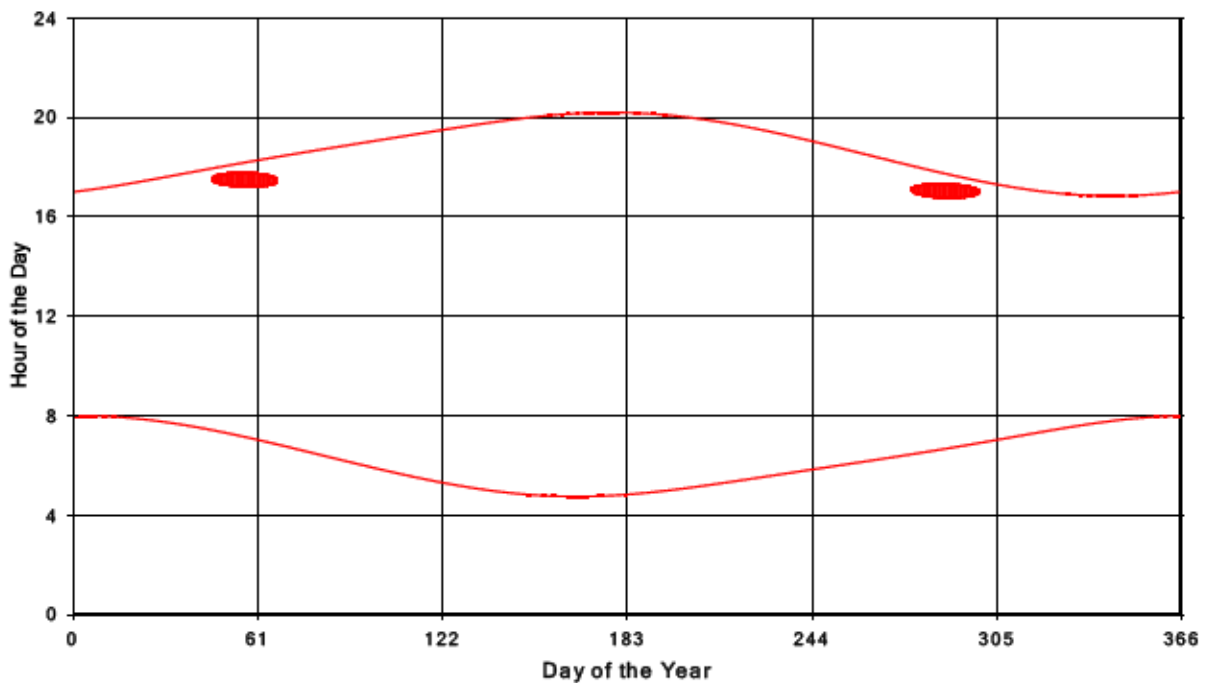
Bluewater Wind Energy Centre Shadow Times on Receptor 297, All Windows from All Turbine
