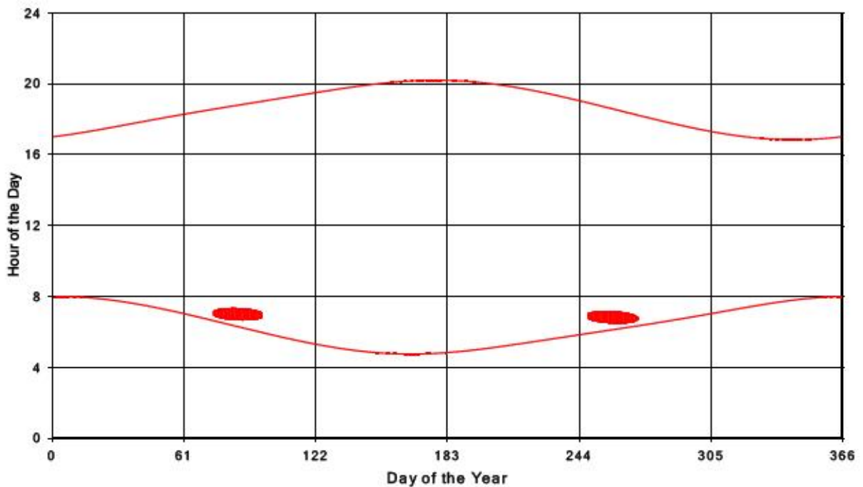
Bluewater Wind Energy Centre Shadow Times on Receptor 382, All Windows from All Turbine
