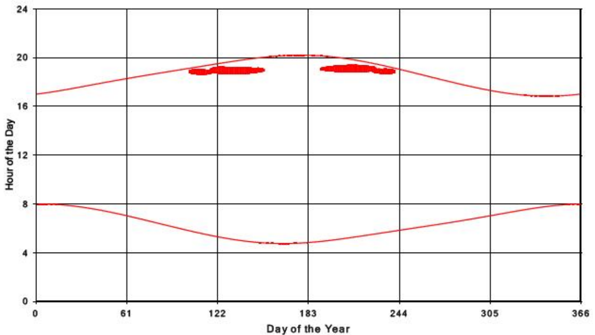
Bluewater Wind Energy Centre Shadow Times on Receptor 406, All Windows from All Turbine
