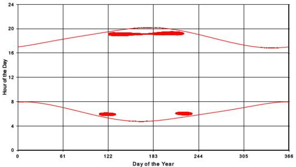
Bluewater Wind Energy Centre Shadow Times on Receptor 178, All Windows from All Turbine
