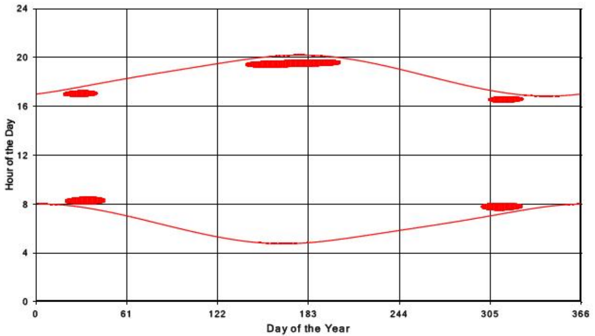
Bluewater Wind Energy Centre Shadow Times on Receptor 389, All Windows from All Turbine
