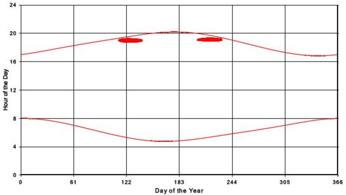
Bluewater Wind Energy Centre Shadow Times on Receptor 73, All Windows from All Turbine:
