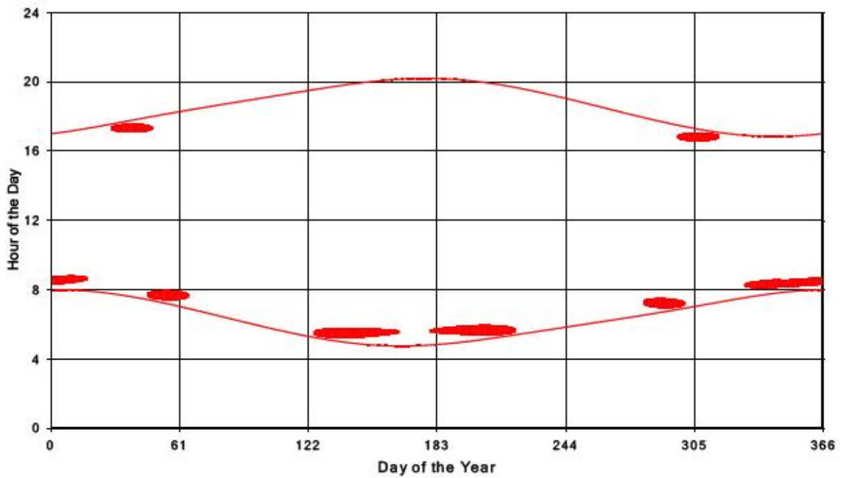
Bluewater Wind Energy Centre Shadow Times on Receptor 112, All Windows from All Turbine
