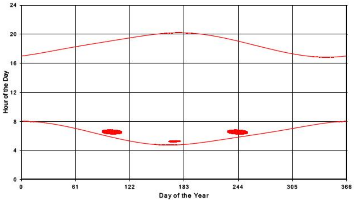
Bluewater Wind Energy Centre Shadow Times on Receptor 87, All Windows from All Turbine:
