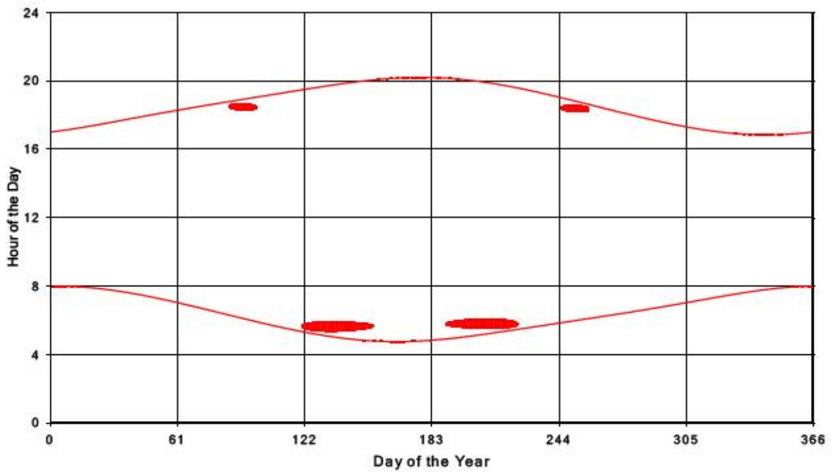
Bluewater Wind Energy Centre Shadow Times on Receptor 244, All Windows from All Turbine
