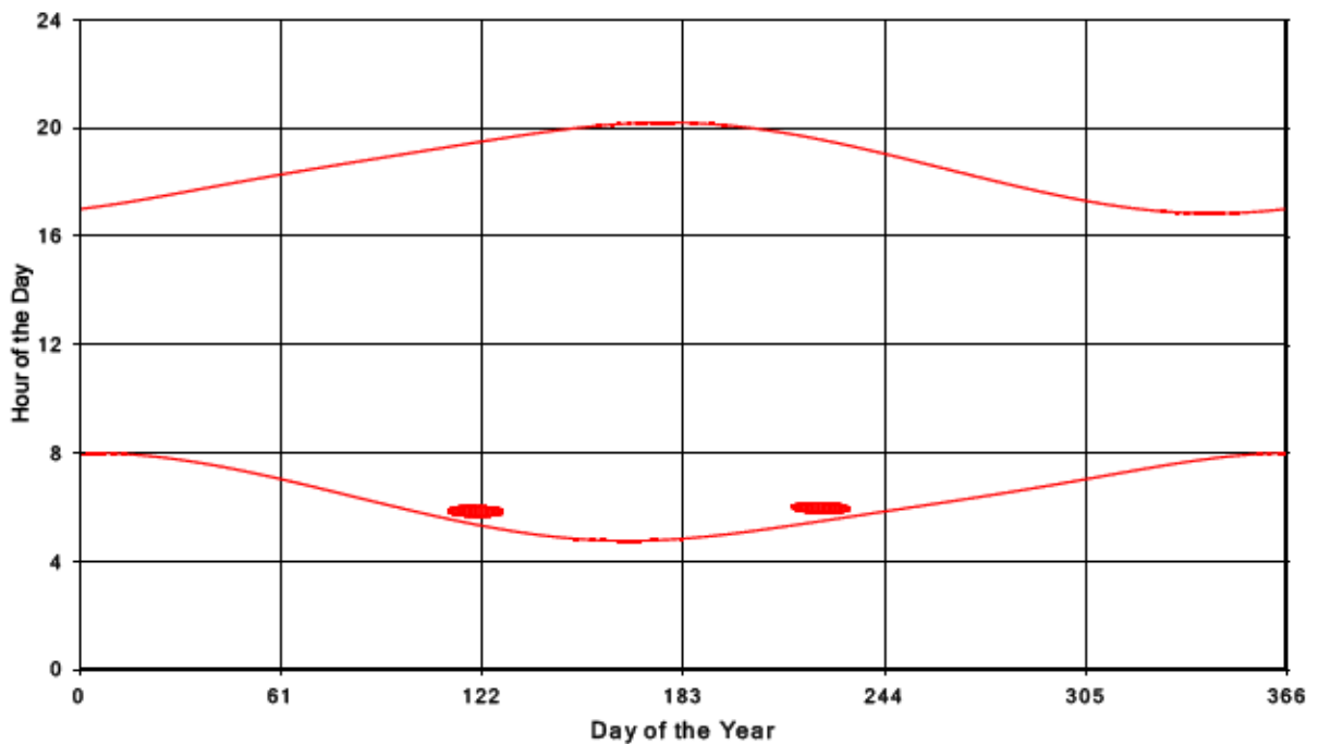
Bluewater Wind Energy Centre Shadow Times on Receptor 6, All Windows from All Turbine:
