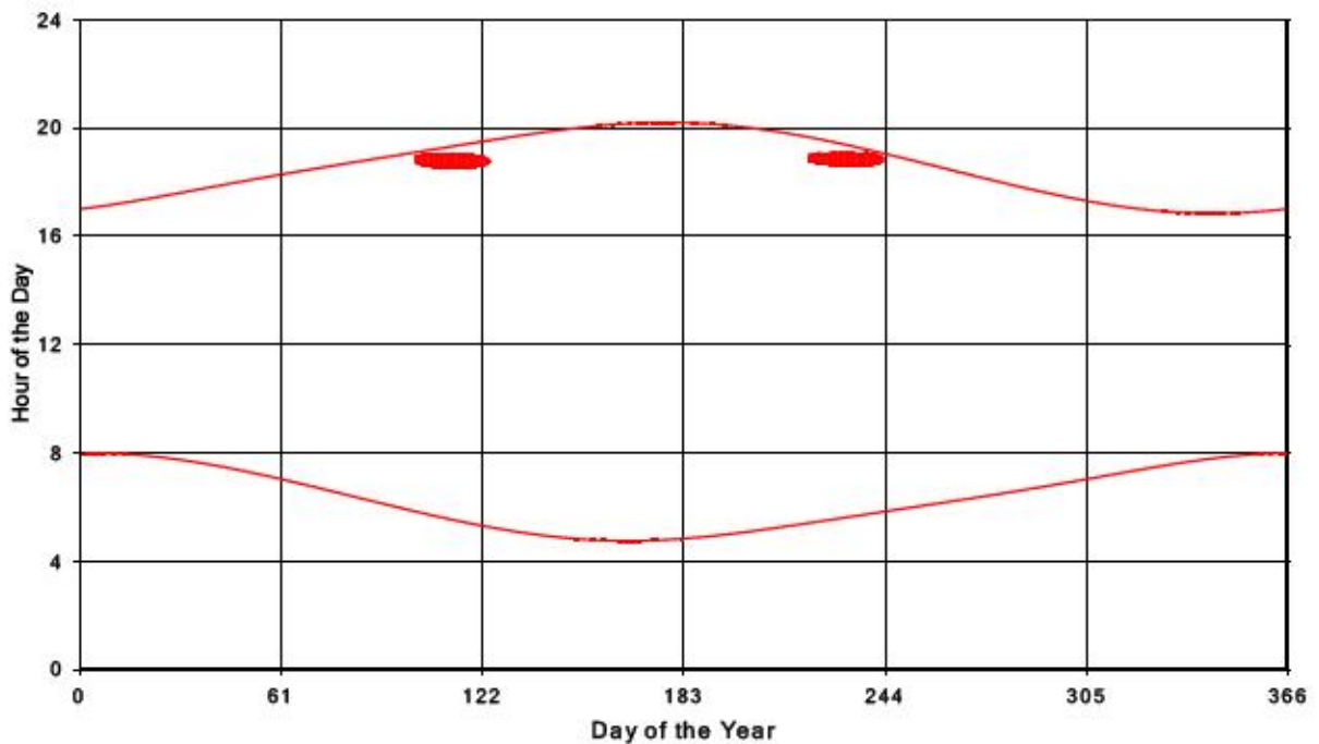
Bluewater Wind Energy Centre Shadow Times on Receptor 264, All Windows from All Turbine
