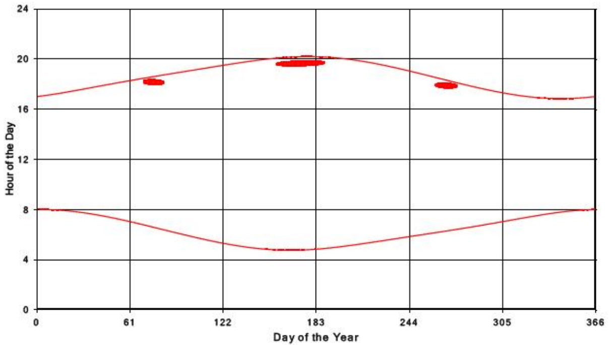
Bluewater Wind Energy Centre Shadow Times on Receptor 141, All Windows from All Turbine
