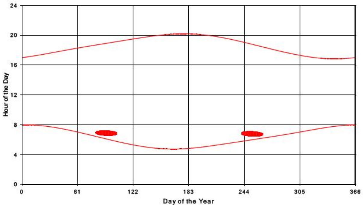
Bluewater Wind Energy Centre Shadow Times on Receptor 398, All Windows from All Turbine
