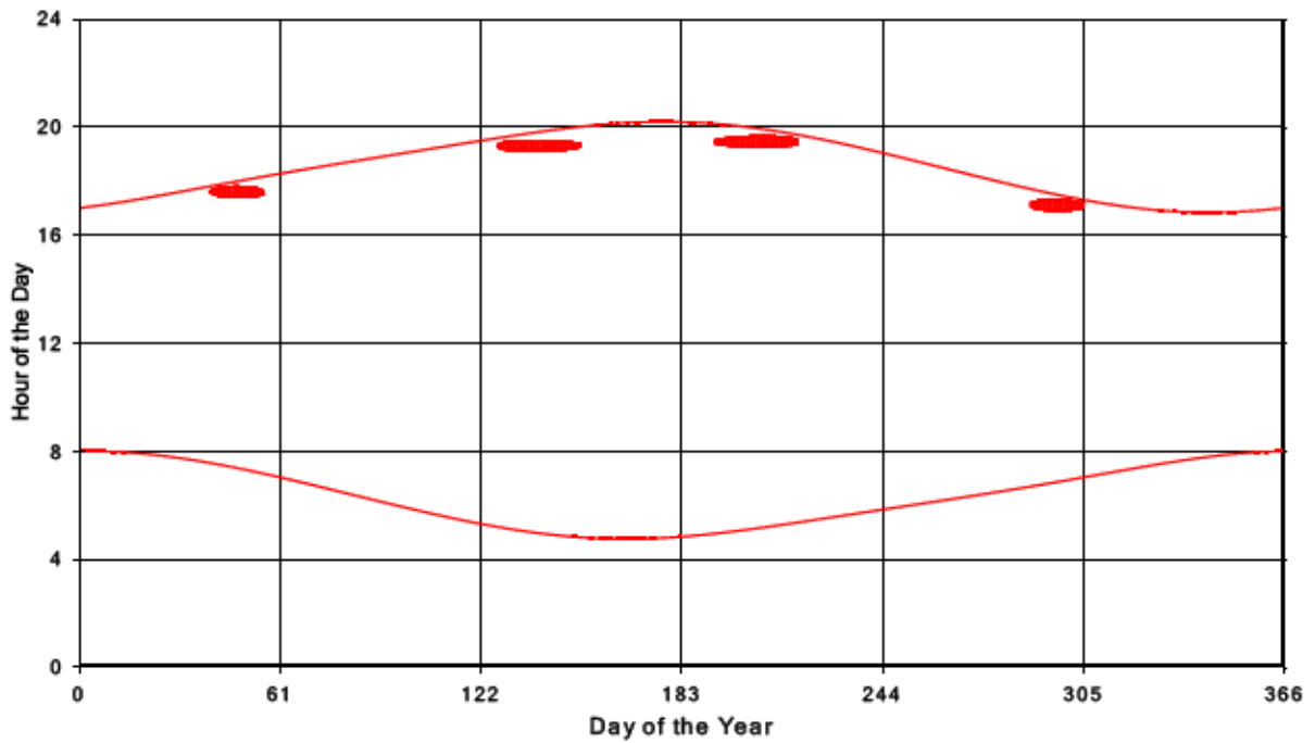
Bluewater Wind Energy Centre Shadow Times on Receptor 265, All Windows from All Turbine
