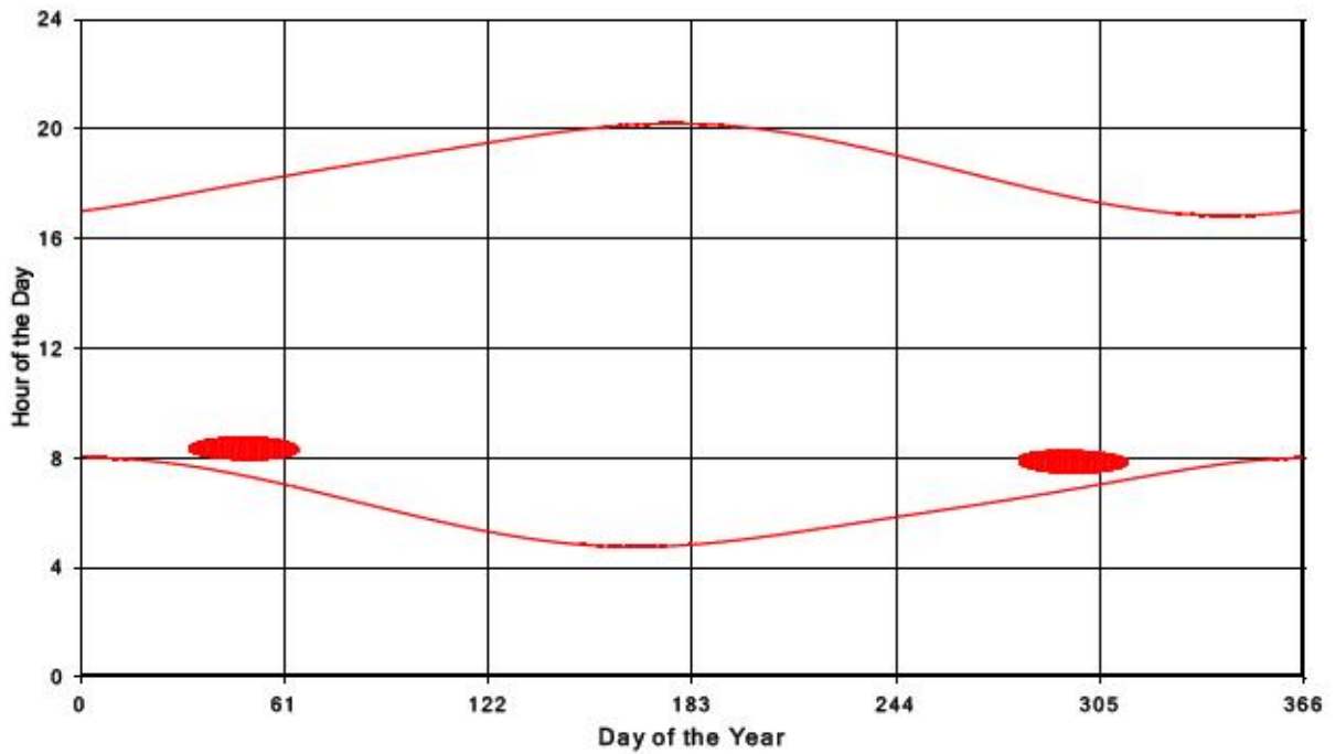
Bluewater Wind Energy Centre Shadow Times on Receptor 409, All Windows from All Turbine
