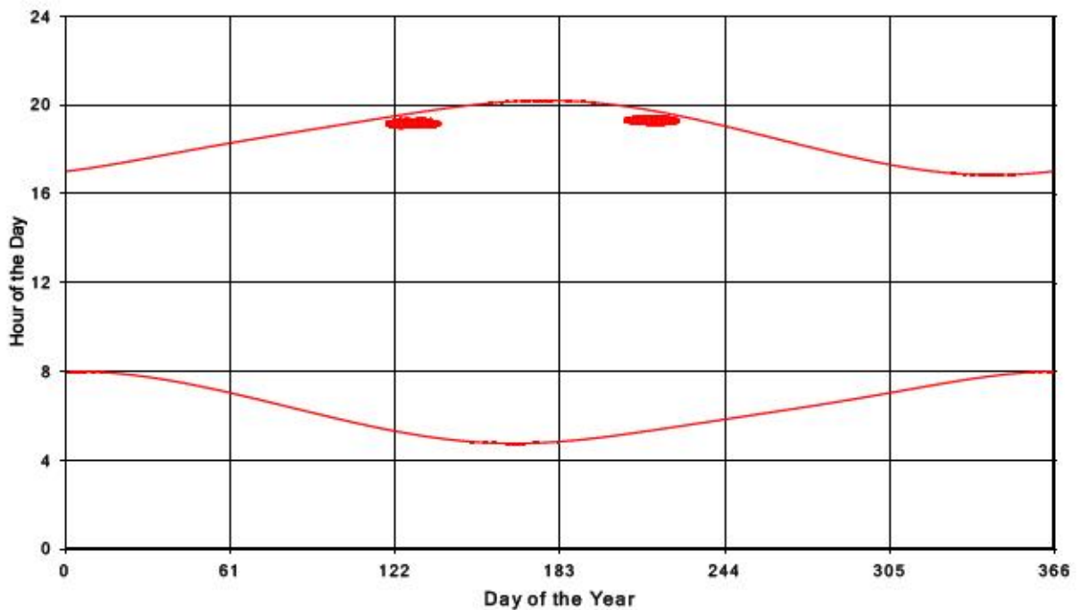
Bluewater Wind Energy Centre Shadow Times on Receptor 116, All Windows from All Turbine
