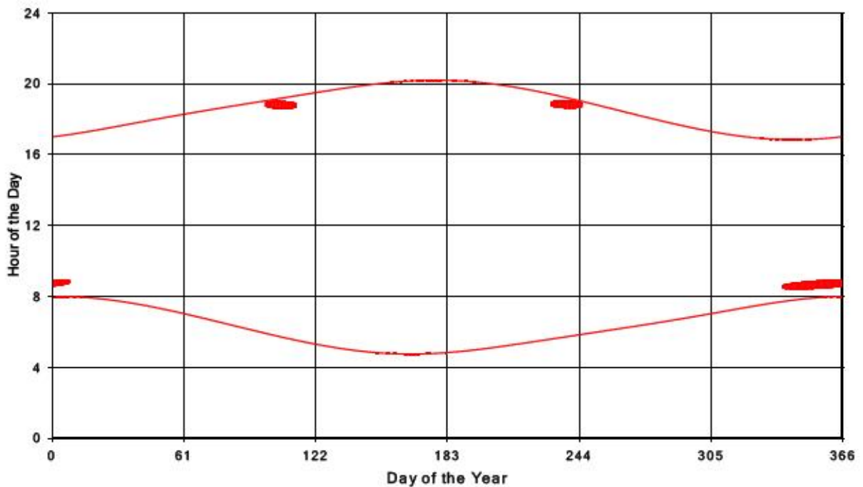
Bluewater Wind Energy Centre Shadow Times on Receptor 221, All Windows from All Turbine
