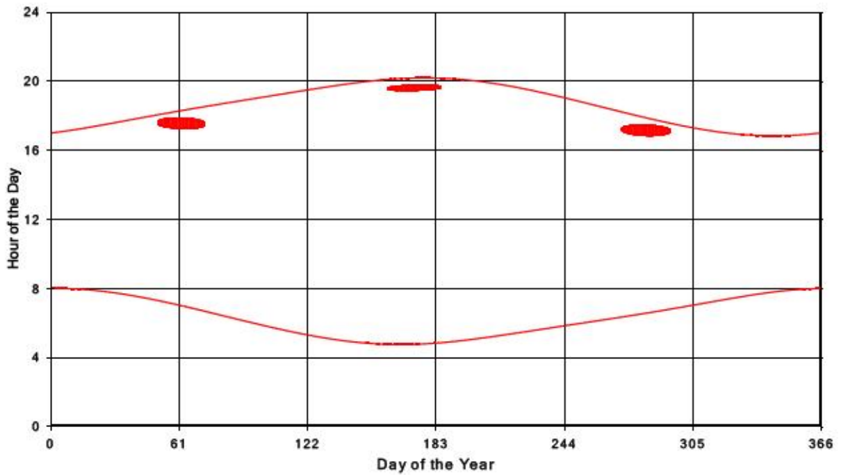
Bluewater Wind Energy Centre Shadow Times on Receptor 383, All Windows from All Turbine
