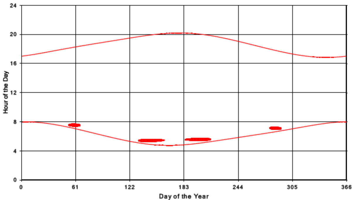
Bluewater Wind Energy Centre Shadow Times on Receptor 325, All Windows from All Turbine
