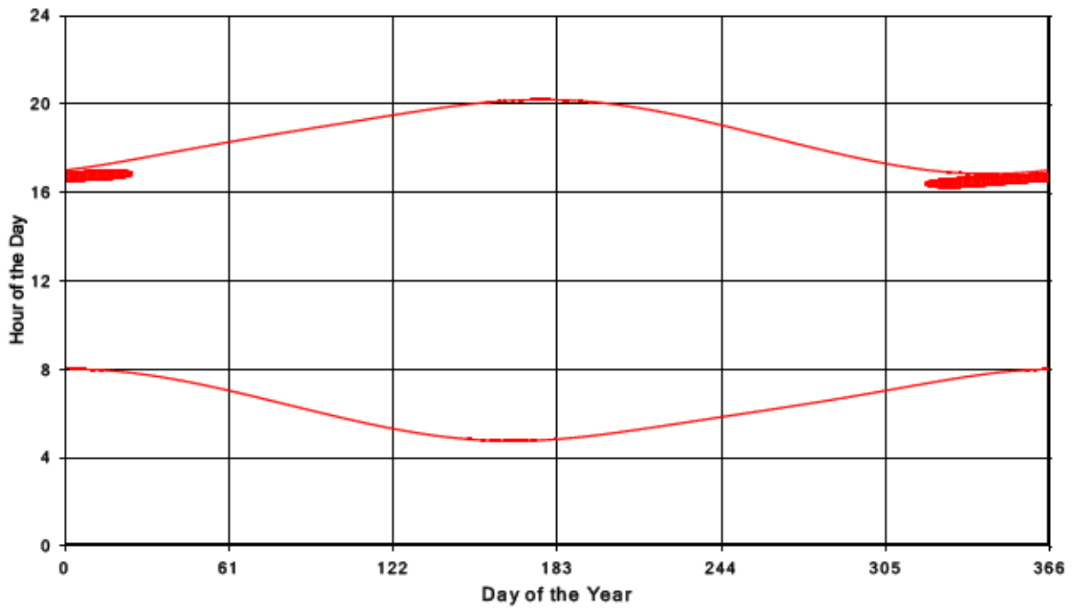
Bluewater Wind Energy Centre Shadow Times on Receptor 62, All Windows from All Turbine:
