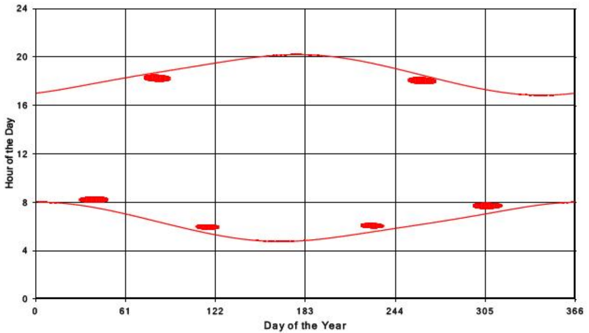
Bluewater Wind Energy Centre Shadow Times on Receptor 47, All Windows from All Turbine:
