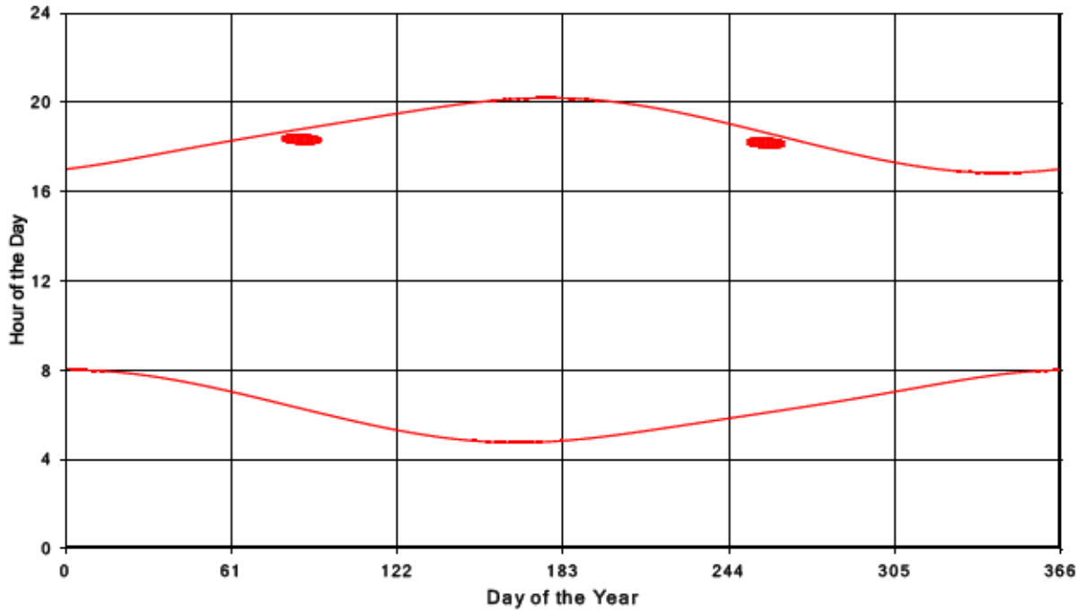
Bluewater Wind Energy Centre Shadow Times on Receptor 319, All Windows from All Turbine
