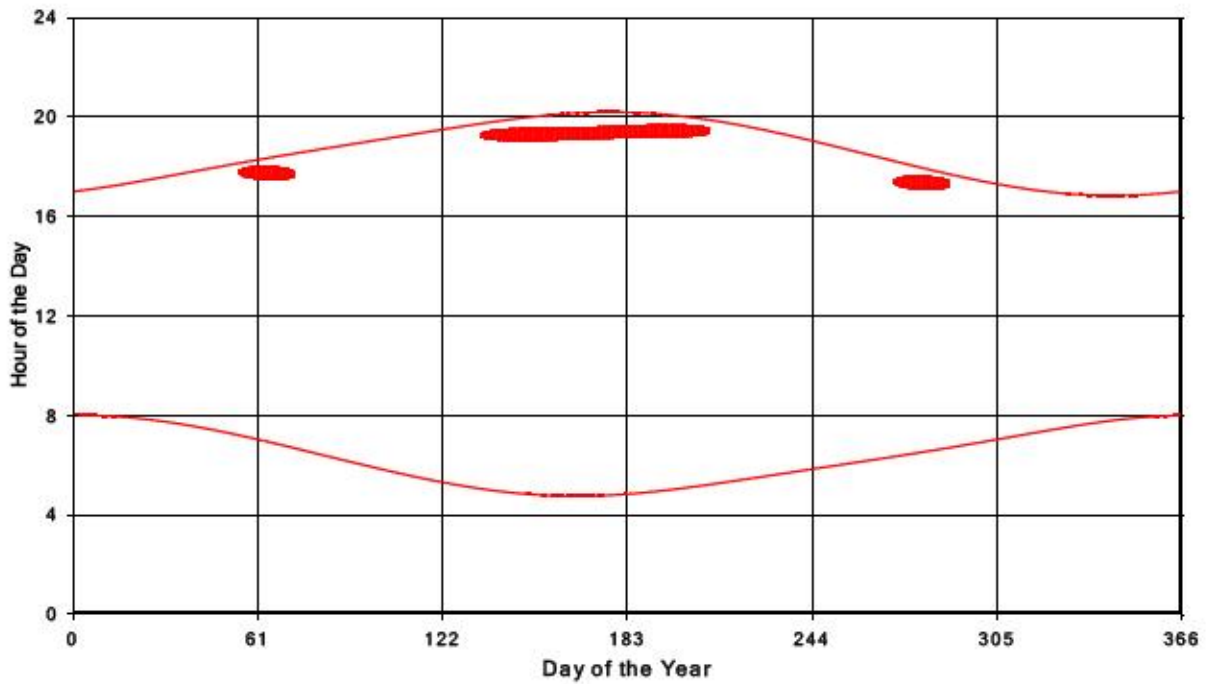
Bluewater Wind Energy Centre Shadow Times on Receptor 291, All Windows from All Turbine
