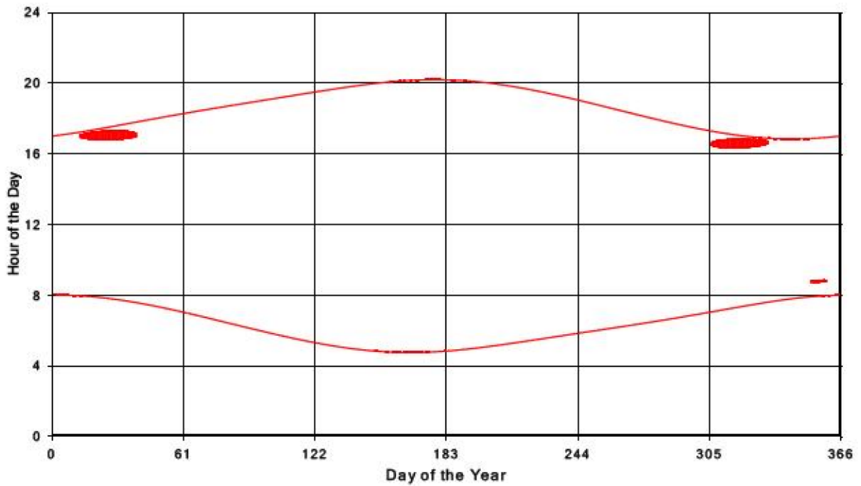
Bluewater Wind Energy Centre Shadow Times on Receptor 39, All Windows from All Turbine:
