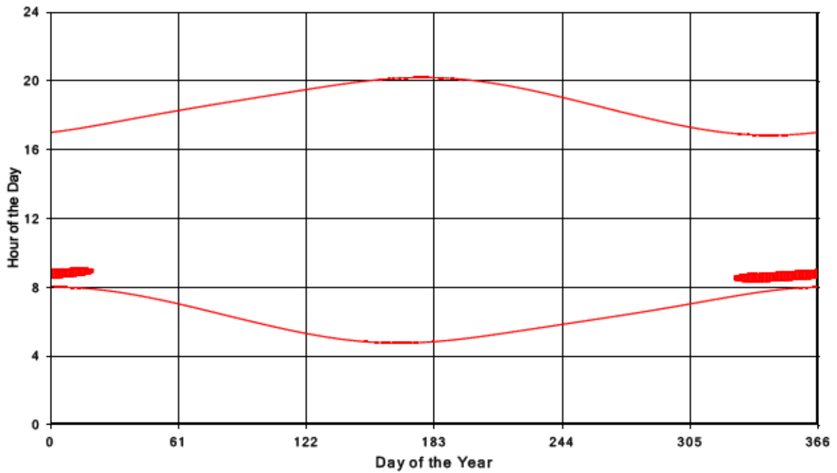
Bluewater Wind Energy Centre Shadow Times on Receptor 83, All Windows from All Turbine:
