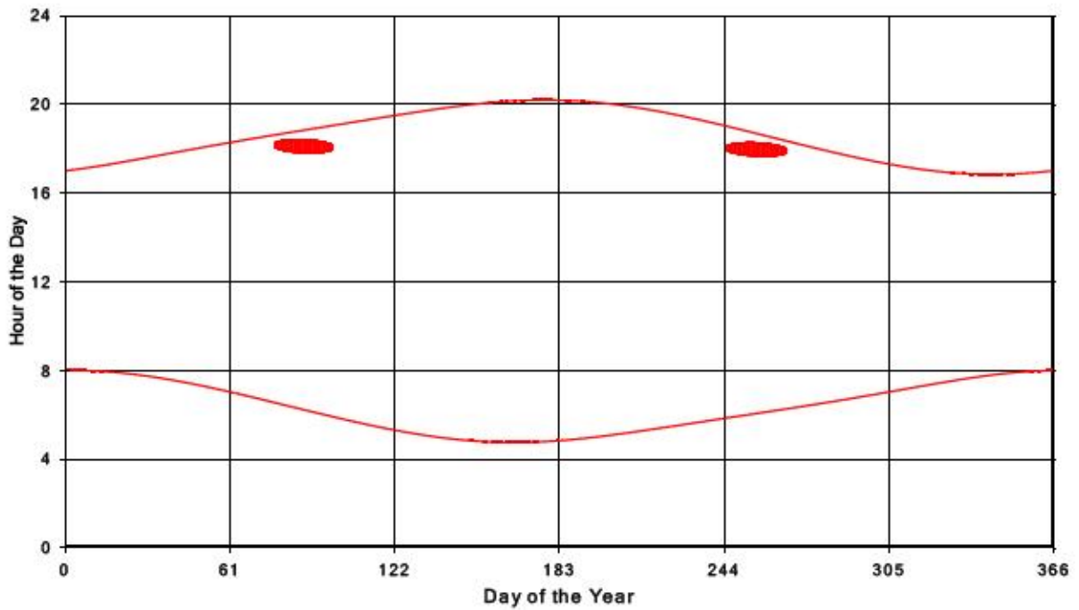
Bluewater Wind Energy Centre Shadow Times on Receptor 404, All Windows from All Turbine
