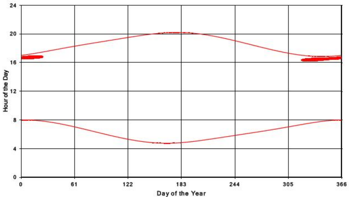
Bluewater Wind Energy Centre Shadow Times on Receptor 394, All Windows from All Turbine
