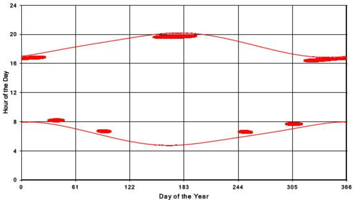
Bluewater Wind Energy Centre Shadow Times on Receptor 46, All Windows from All Turbine:
