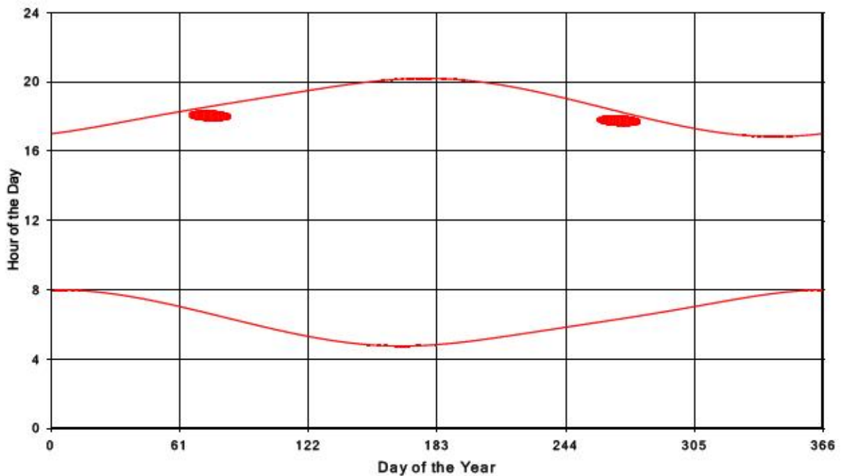
Bluewater Wind Energy Centre Shadow Times on Receptor 203, All Windows from All Turbine
