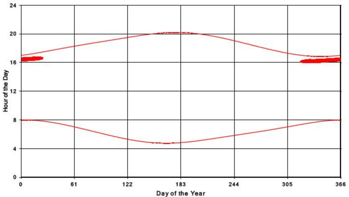
Bluewater Wind Energy Centre Shadow Times on Receptor 386, All Windows from All Turbine
