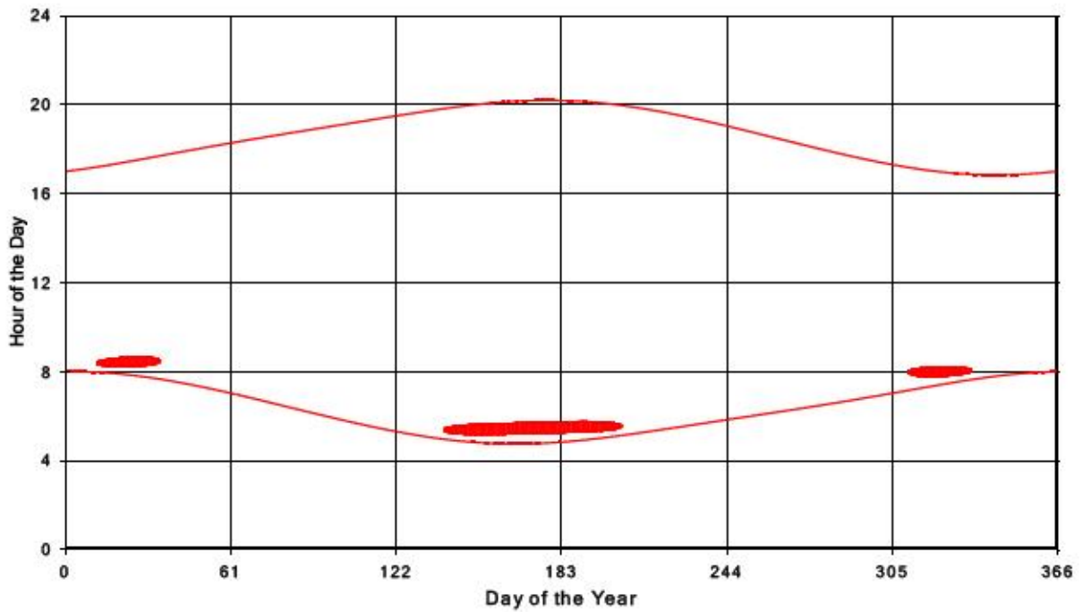
Bluewater Wind Energy Centre Shadow Times on Receptor 22, All Windows from All Turbine:
