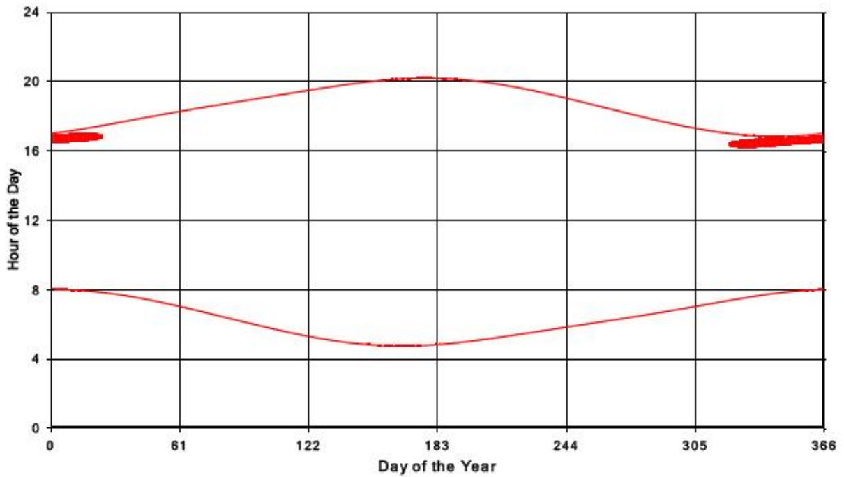
Bluewater Wind Energy Centre Shadow Times on Receptor 66, All Windows from All Turbine:
