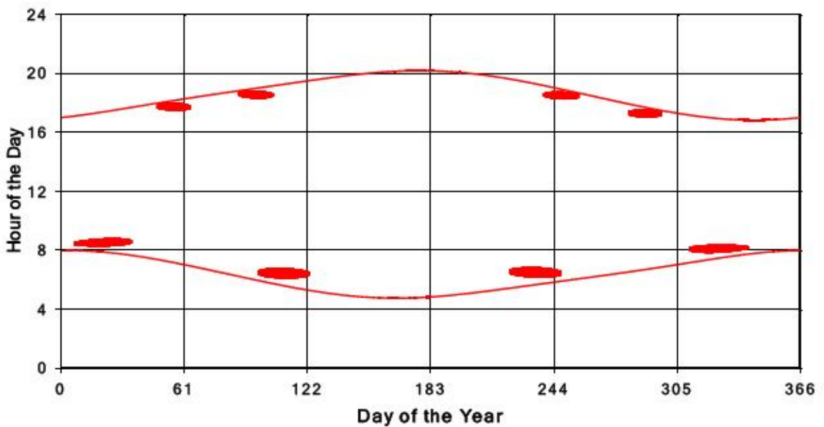
Bluewater Wind Energy Centre Shadow Times on Receptor 36, All Windows from All Turbine:
