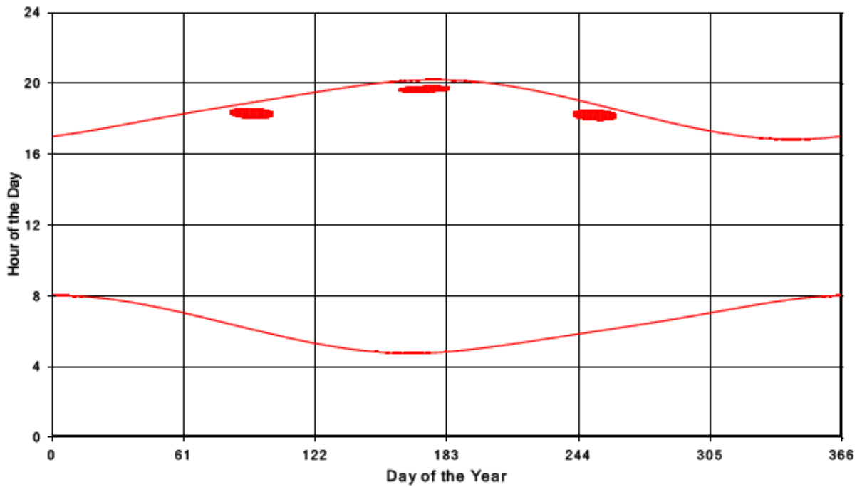
Bluewater Wind Energy Centre Shadow Times on Receptor 301, All Windows from All Turbine
