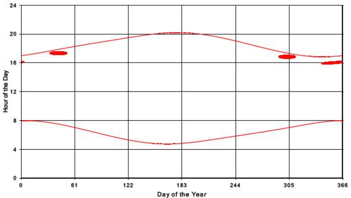
Bluewater Wind Energy Centre Shadow Times on Receptor 129, All Windows from All Turbine
