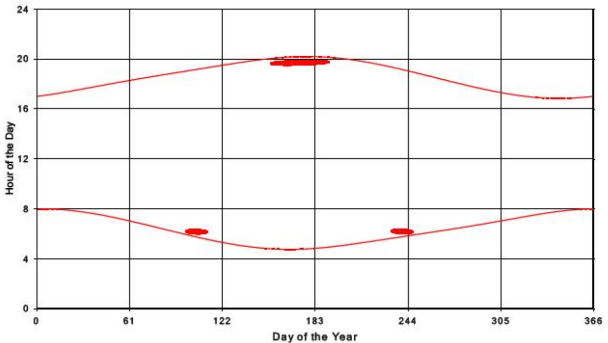
Bluewater Wind Energy Centre Shadow Times on Receptor 295, All Windows from All Turbine
