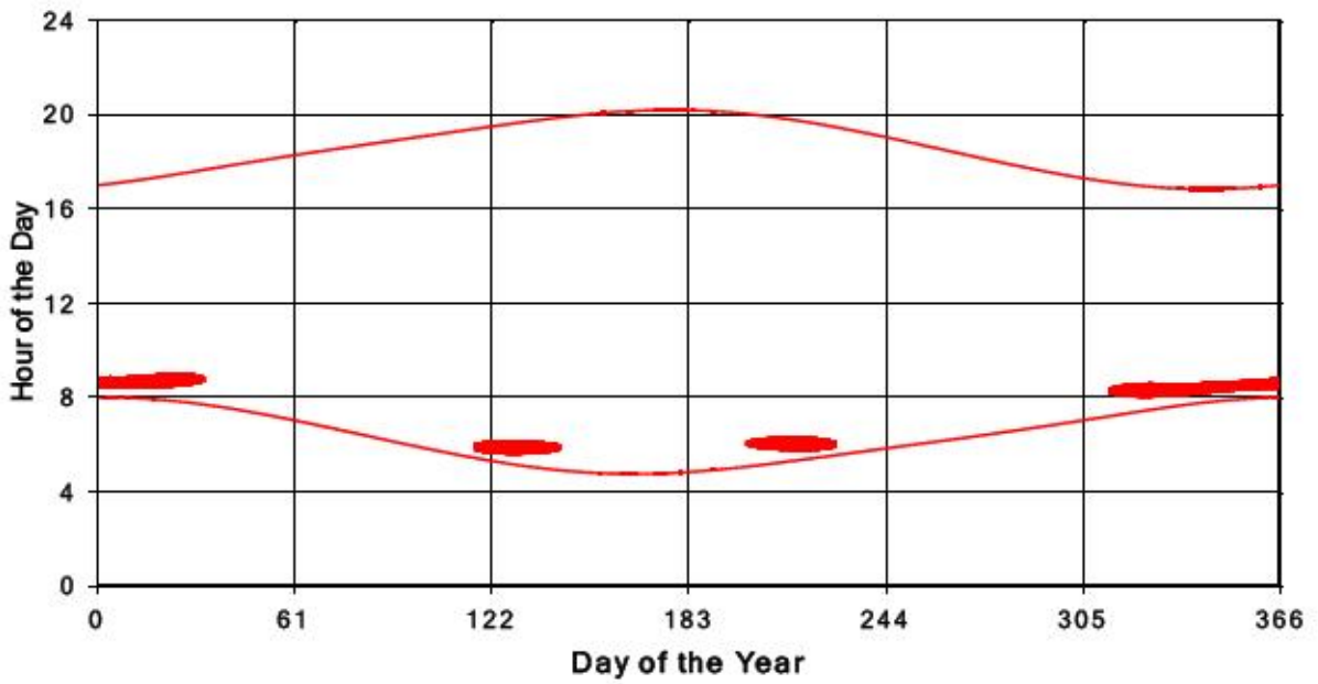
Bluewater Wind Energy Centre Shadow Times on Receptor 229, All Windows from All Turbine
