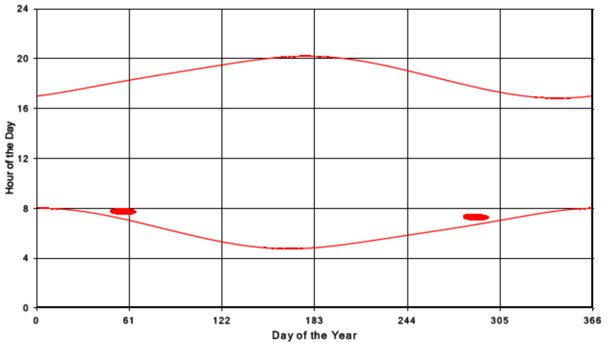
Bluewater Wind Energy Centre Shadow Times on Receptor 24, All Windows from All Turbine:
