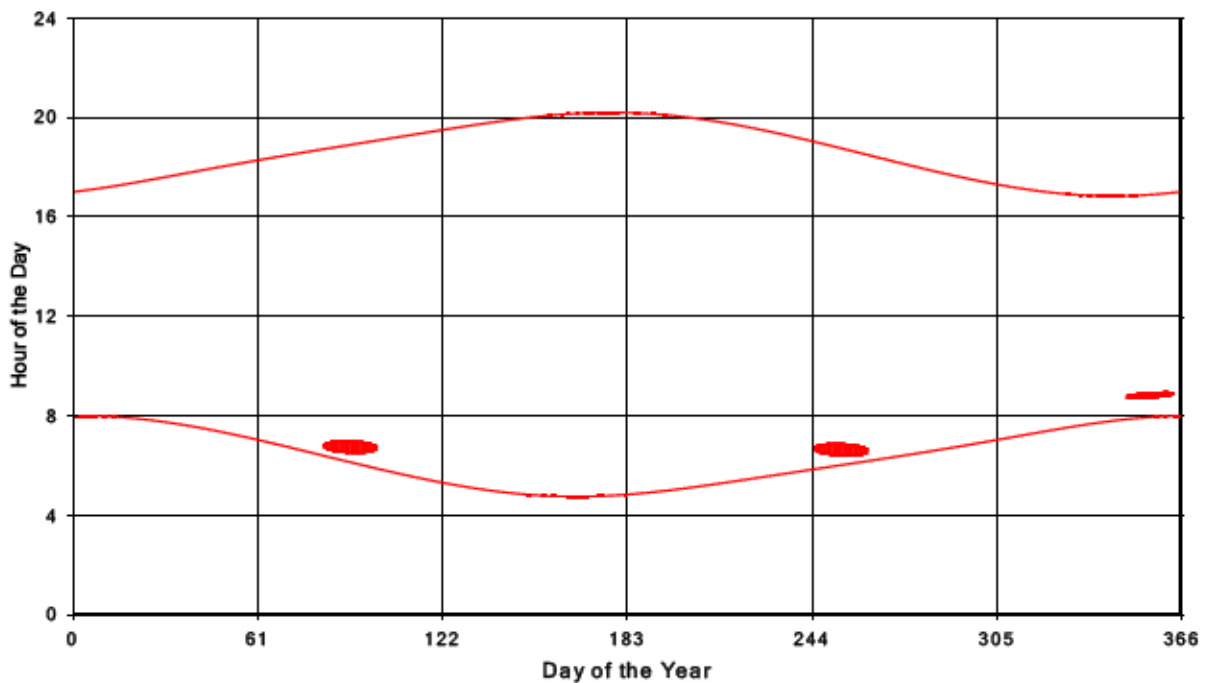
Bluewater Wind Energy Centre Shadow Times on Receptor 26, All Windows from All Turbine:
