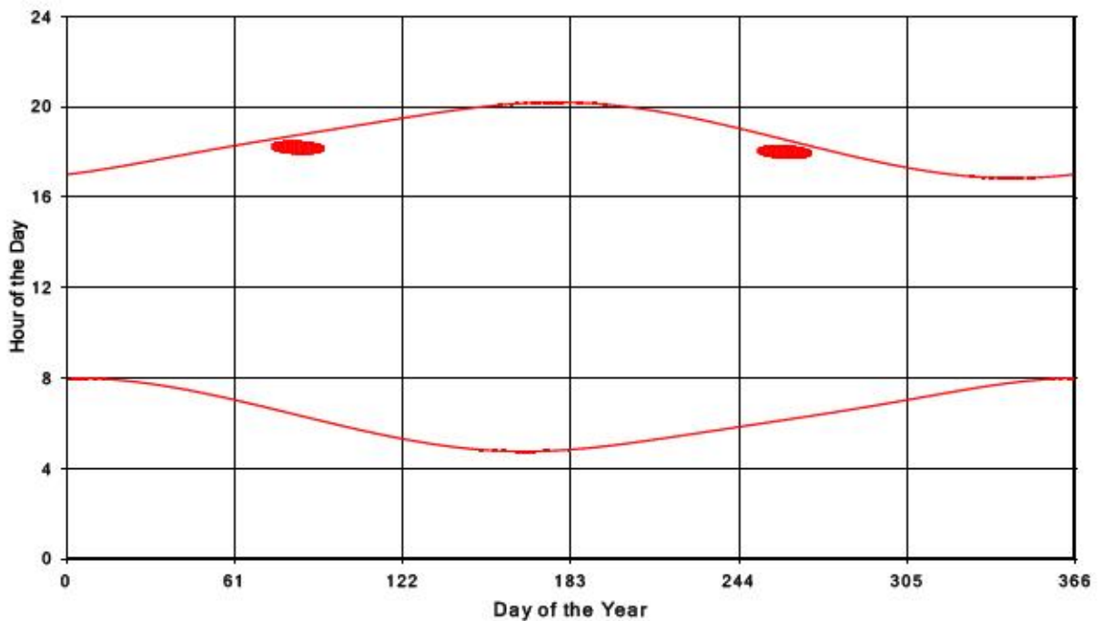
Bluewater Wind Energy Centre Shadow Times on Receptor 251, All Windows from All Turbine
