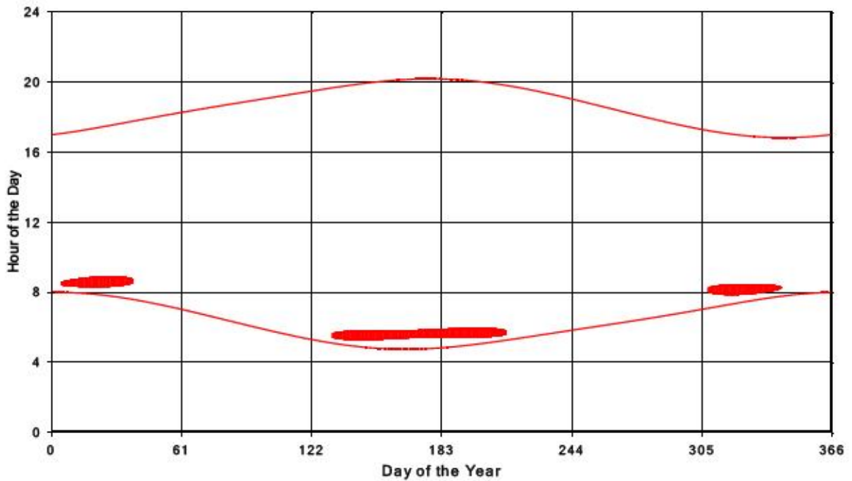
Bluewater Wind Energy Centre Shadow Times on Receptor 348, All Windows from All Turbine
