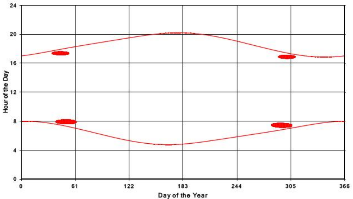
Bluewater Wind Energy Centre Shadow Times on Receptor 293, All Windows from All Turbine
