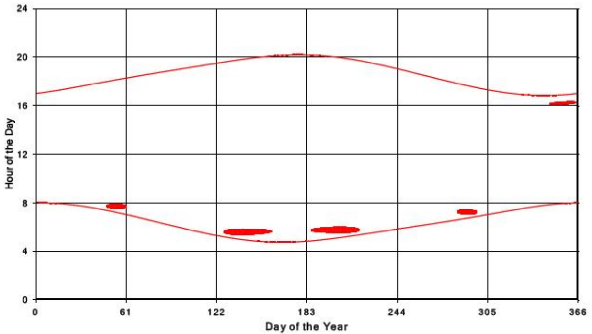
Bluewater Wind Energy Centre Shadow Times on Receptor 41, All Windows from All Turbine:
