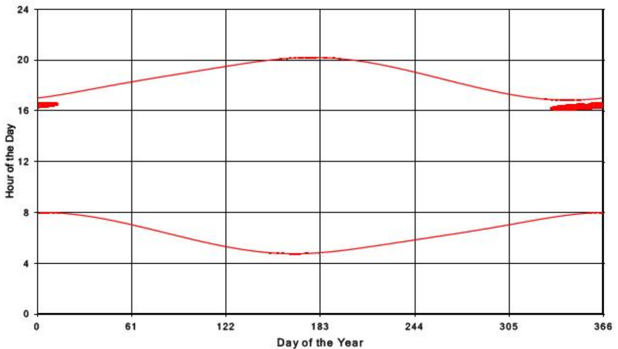
Bluewater Wind Energy Centre Shadow Times on Receptor 52, All Windows from All Turbine:
