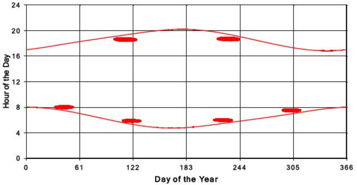
Bluewater Wind Energy Centre Shadow Times on Receptor 237, All Windows from All Turbine
