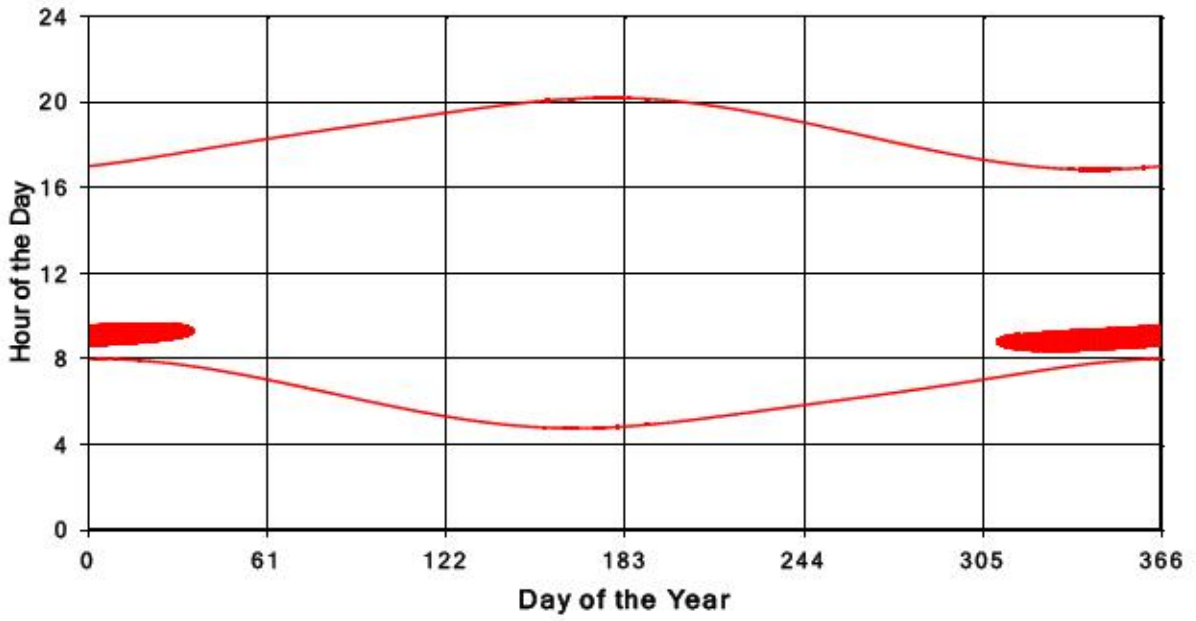
Bluewater Wind Energy Centre Shadow Times on Receptor 231, All Windows from All Turbine
