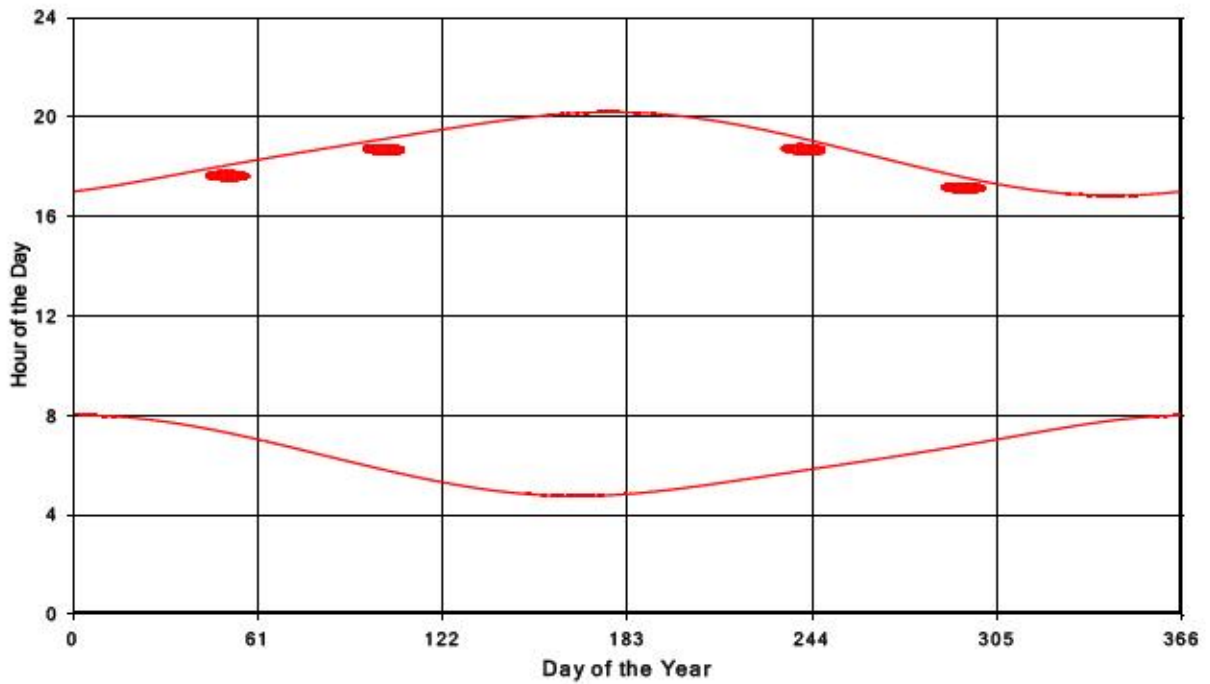
Bluewater Wind Energy Centre Shadow Times on Receptor 393, All Windows from All Turbine
