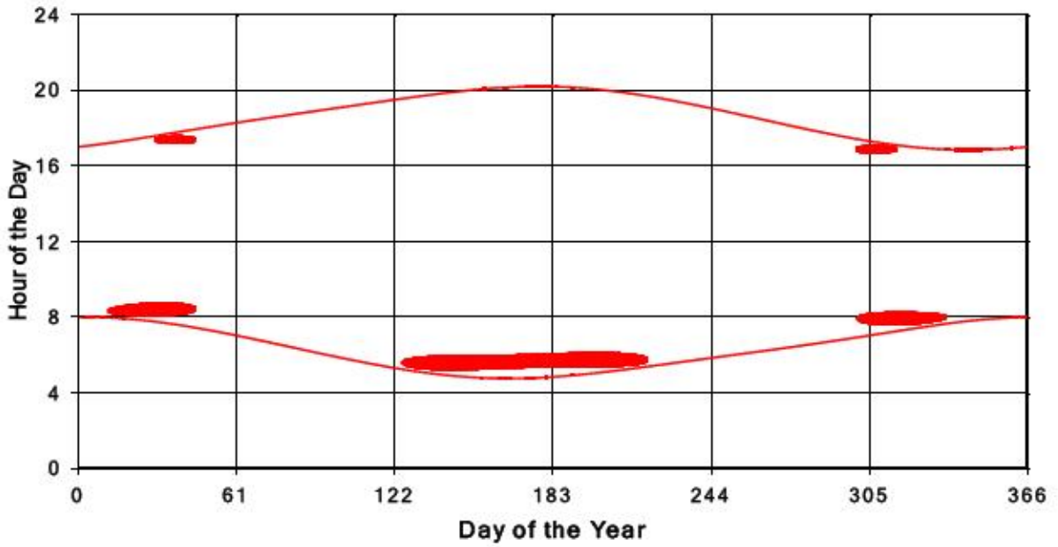
Bluewater Wind Energy Centre Shadow Times on Receptor 226, All Windows from All Turbine
