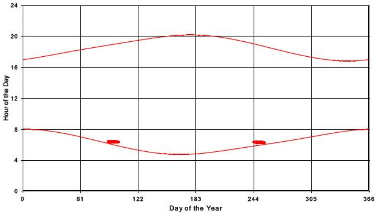
Bluewater Wind Energy Centre Shadow Times on Receptor 127, All Windows from All Turbine
