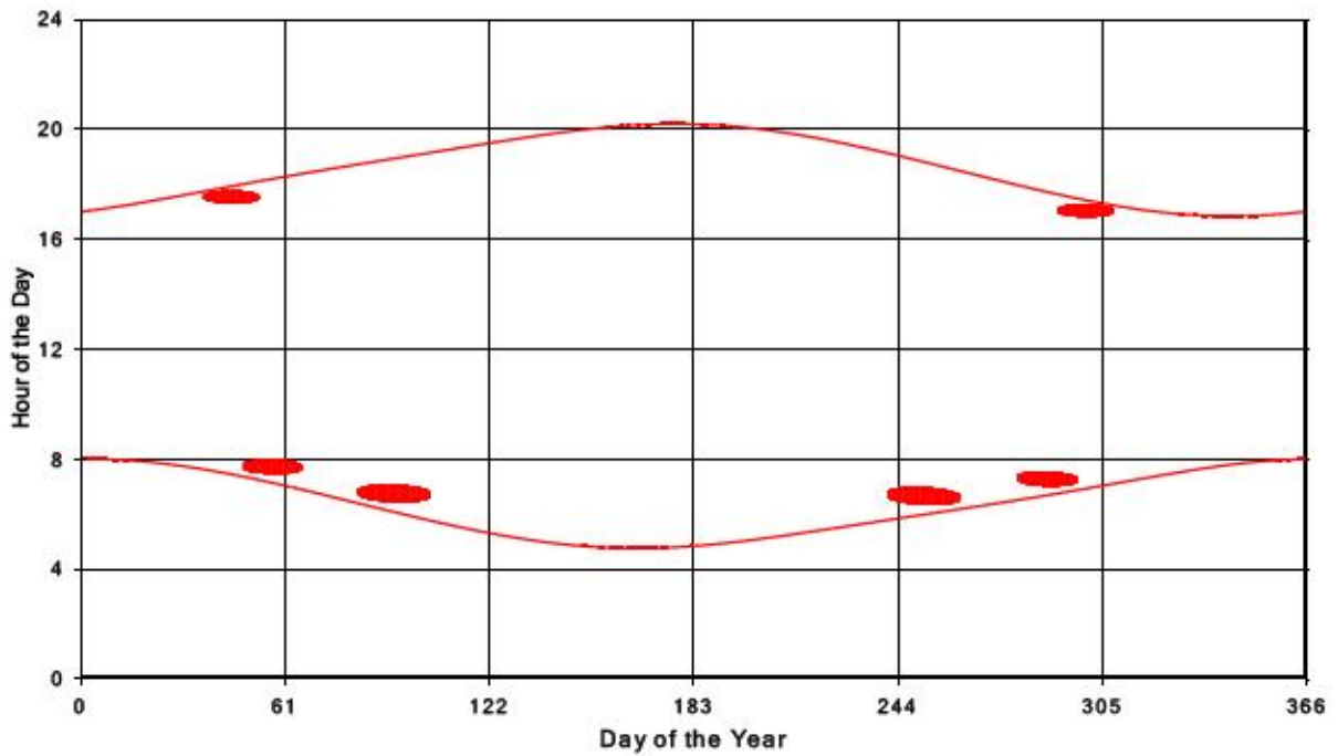
Bluewater Wind Energy Centre Shadow Times on Receptor 271, All Windows from All Turbine
