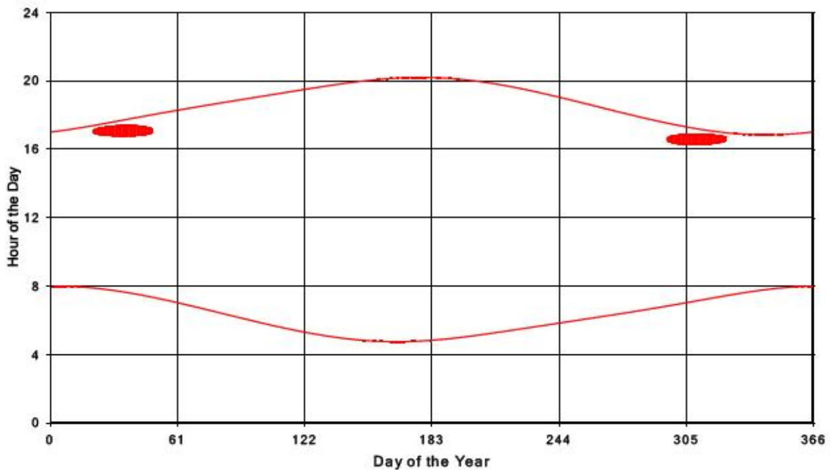
Bluewater Wind Energy Centre Shadow Times on Receptor 67, All Windows from All Turbine:
