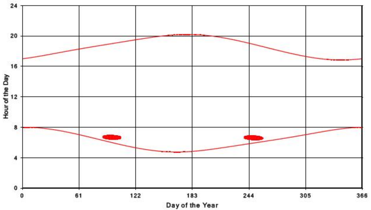
Bluewater Wind Energy Centre Shadow Times on Receptor 190, All Windows from All Turbine
