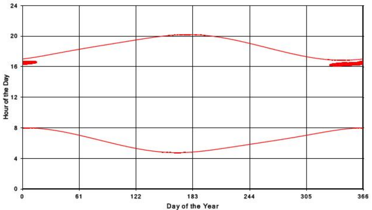
Bluewater Wind Energy Centre Shadow Times on Receptor 54, All Windows from All Turbine:
