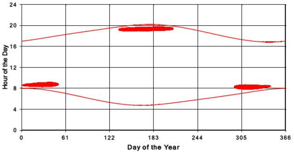
Bluewater Wind Energy Centre Shadow Times on Receptor 238, All Windows from All Turbine
