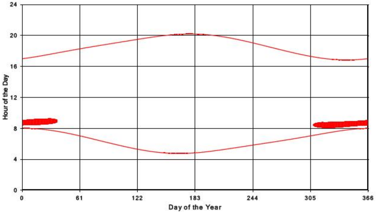
Bluewater Wind Energy Centre Shadow Times on Receptor 330, All Windows from All Turbine
