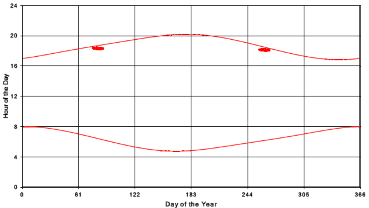
Bluewater Wind Energy Centre Shadow Times on Receptor 312, All Windows from All Turbine
