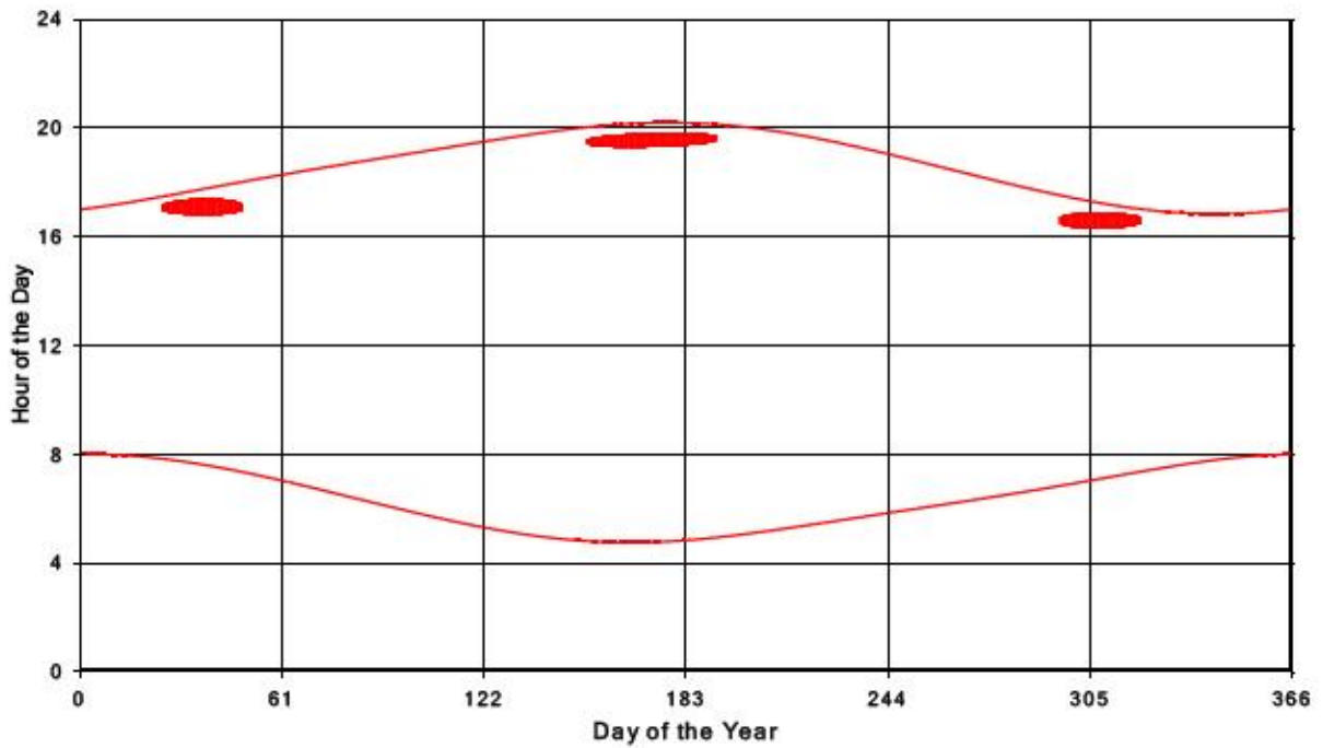
Bluewater Wind Energy Centre Shadow Times on Receptor 298, All Windows from All Turbine
