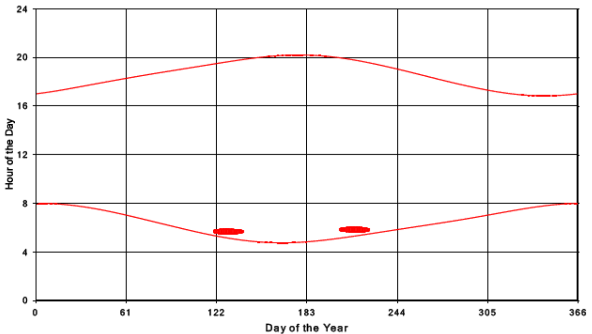
Bluewater Wind Energy Centre Shadow Times on Receptor 8, All Windows from All Turbine:
