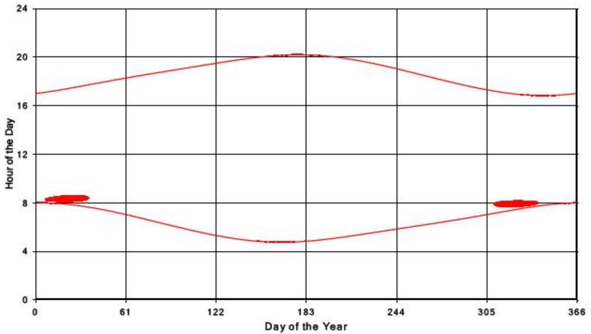
Bluewater Wind Energy Centre Shadow Times on Receptor 118, All Windows from All Turbine
