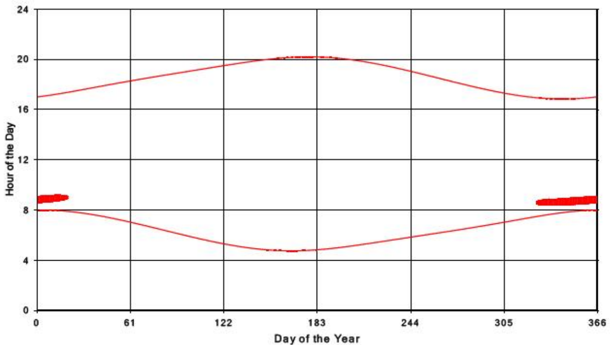
Bluewater Wind Energy Centre Shadow Times on Receptor 10, All Windows from All Turbine:
