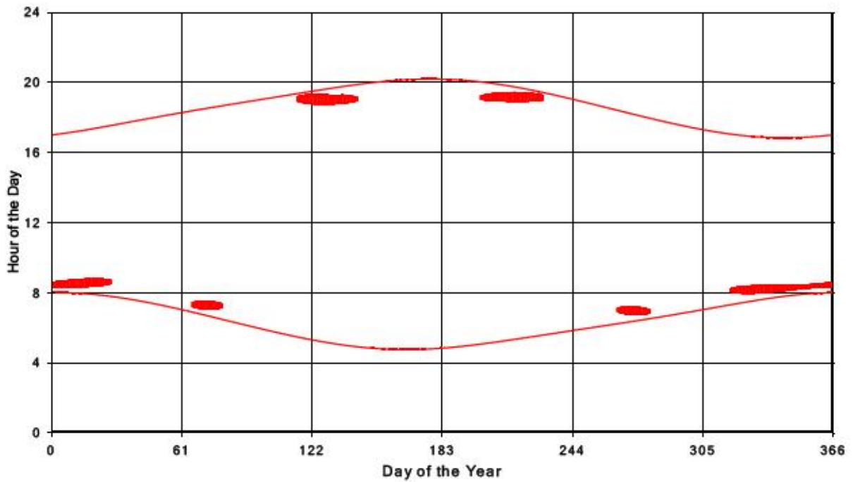
Bluewater Wind Energy Centre Shadow Times on Receptor 43, All Windows from All Turbine:
