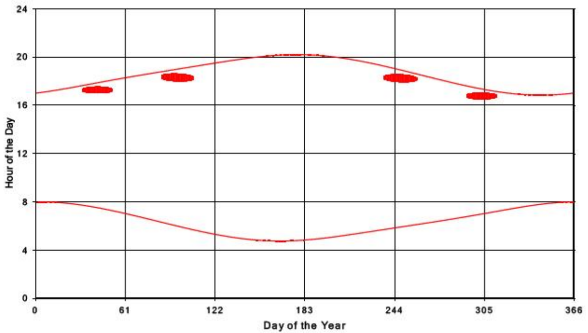
Bluewater Wind Energy Centre Shadow Times on Receptor 300, All Windows from All Turbine
