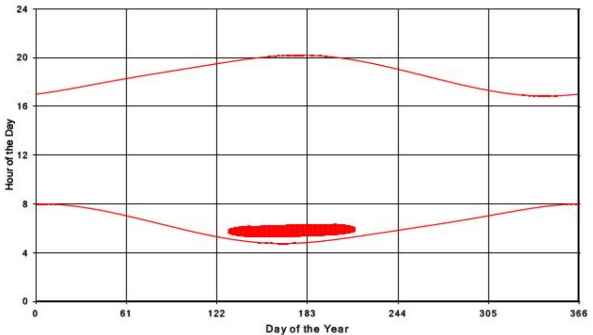
Bluewater Wind Energy Centre Shadow Times on Receptor 388, All Windows from All Turbine
