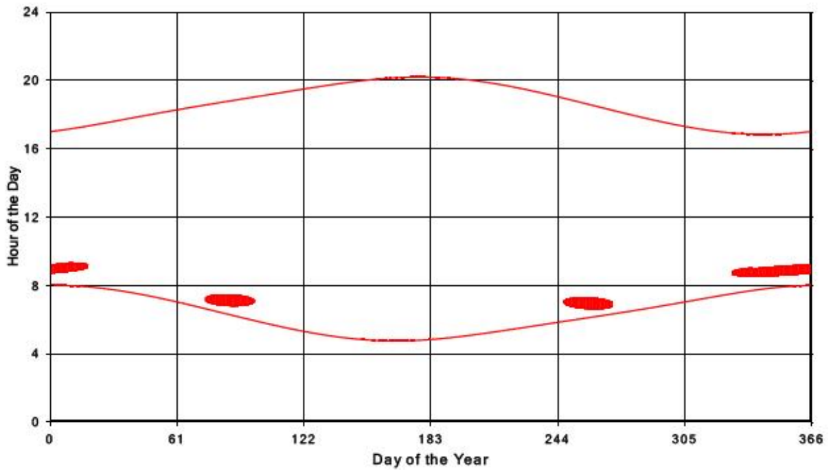
Bluewater Wind Energy Centre Shadow Times on Receptor 53, All Windows from All Turbine:
