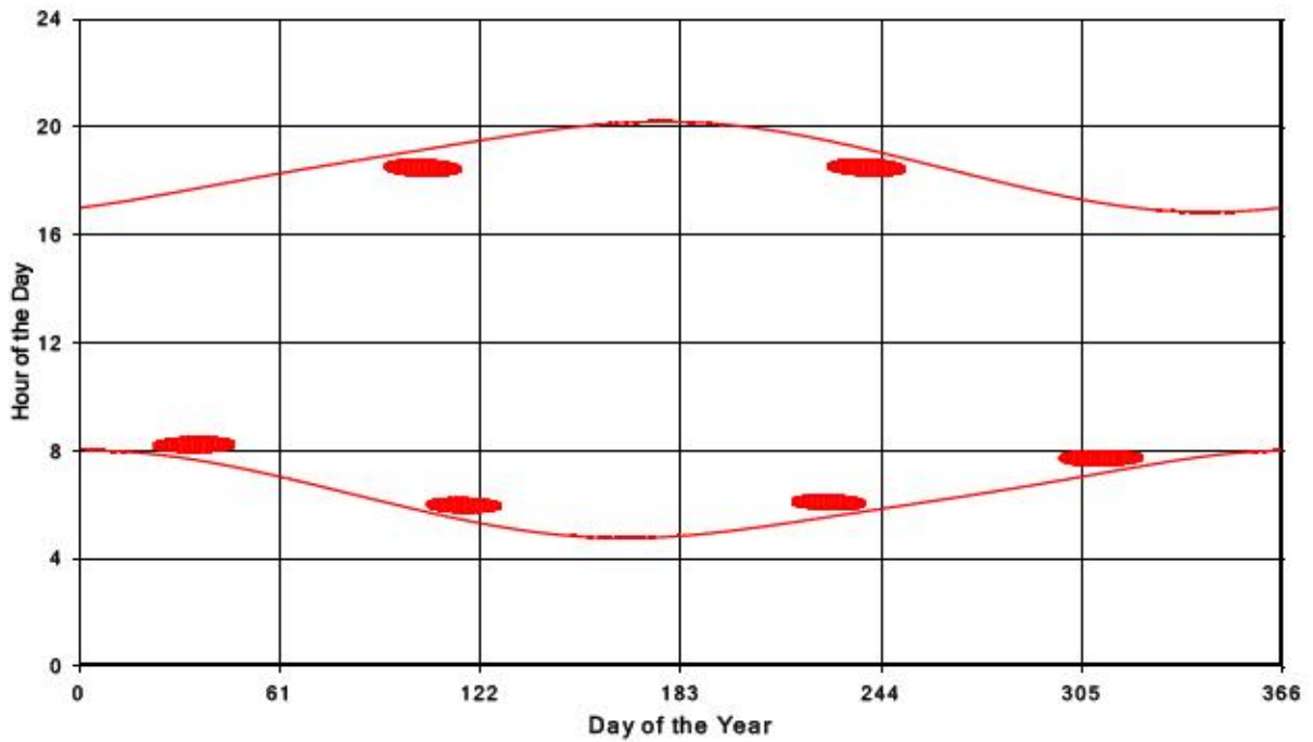
Bluewater Wind Energy Centre Shadow Times on Receptor 241, All Windows from All Turbine
