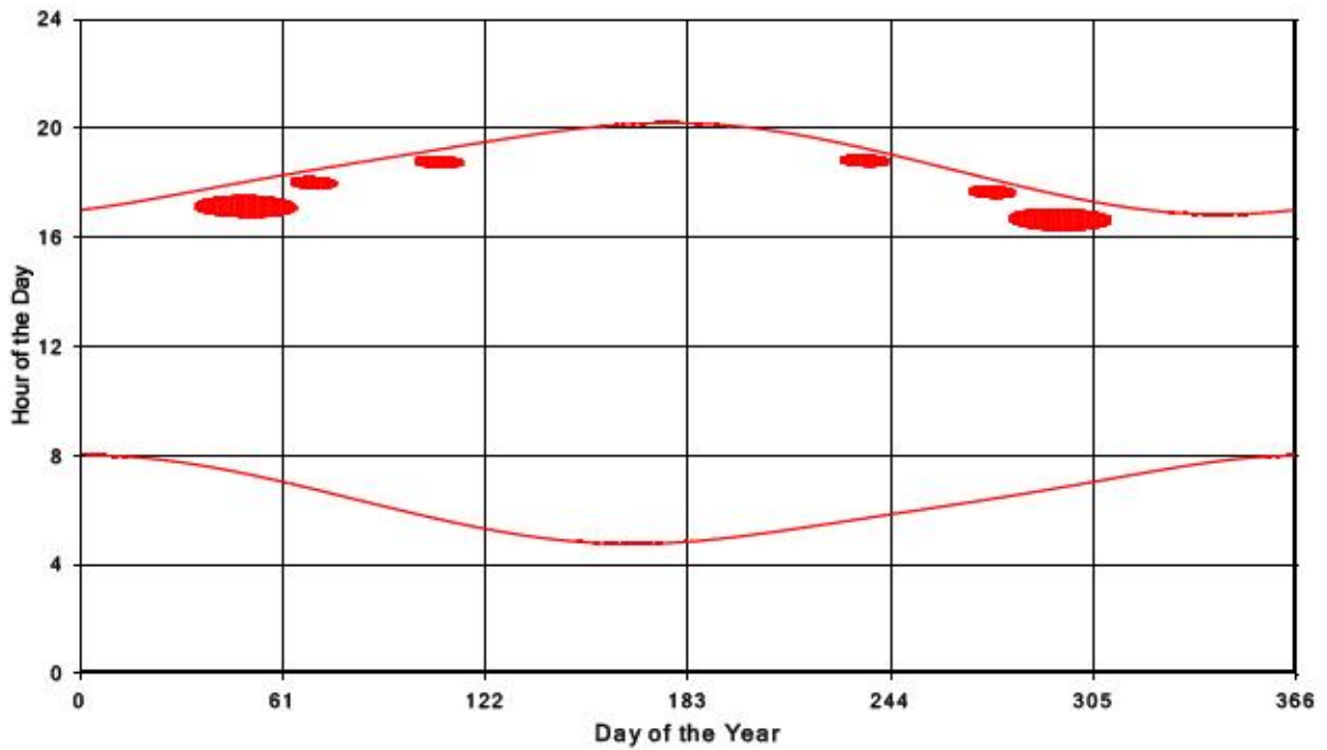
Bluewater Wind Energy Centre Shadow Times on Receptor 397, All Windows from All Turbine
