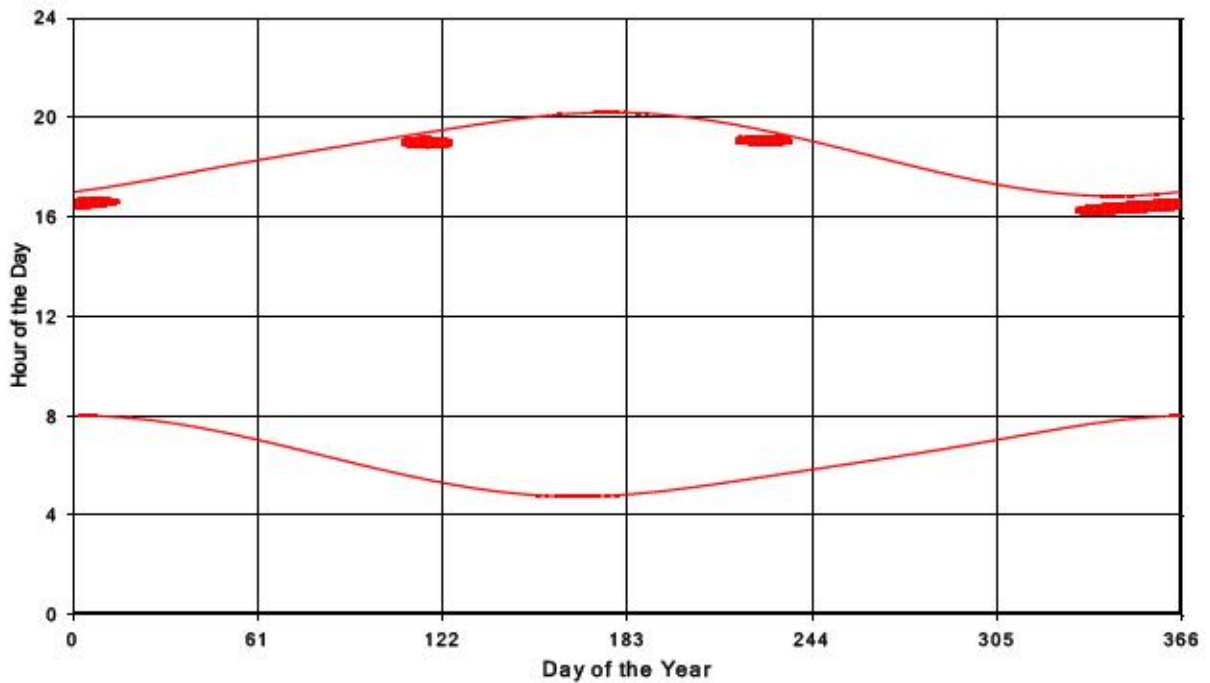
Bluewater Wind Energy Centre Shadow Times on Receptor 210, All Windows from All Turbine
