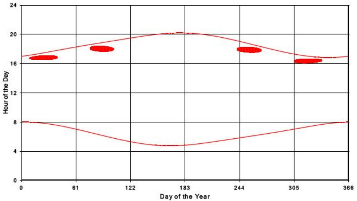
Bluewater Wind Energy Centre Shadow Times on Receptor 402, All Windows from All Turbine
