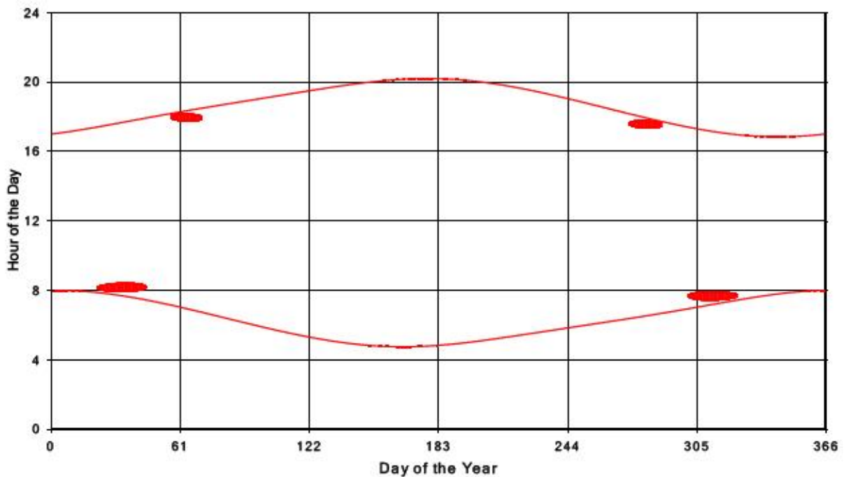
Bluewater Wind Energy Centre Shadow Times on Receptor 277, All Windows from All Turbine
