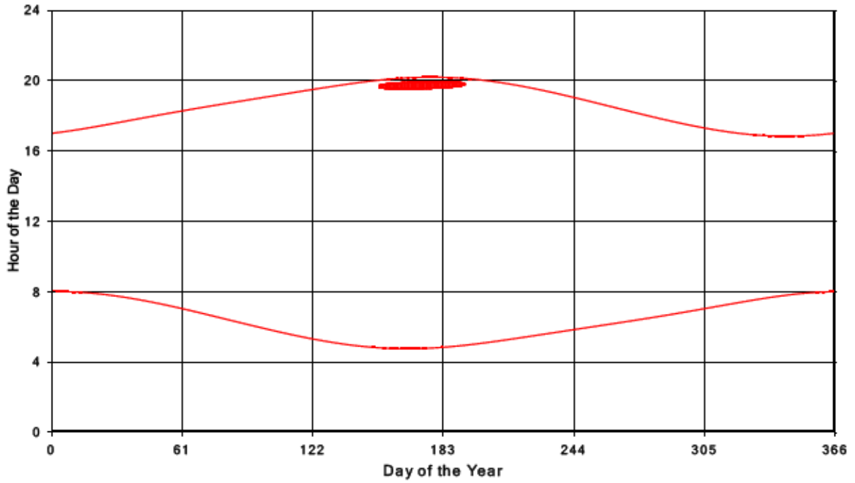
Bluewater Wind Energy Centre Shadow Times on Receptor 183, All Windows from All Turbine
