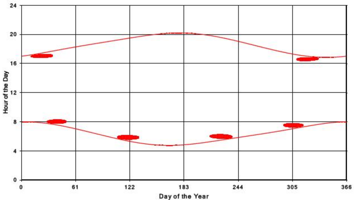
Bluewater Wind Energy Centre Shadow Times on Receptor 110, All Windows from All Turbine
