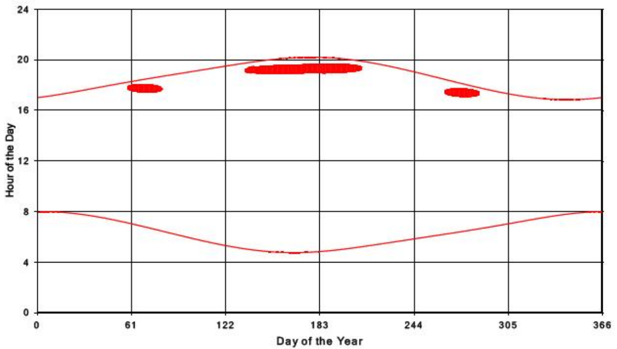
Bluewater Wind Energy Centre Shadow Times on Receptor 403, All Windows from All Turbine
