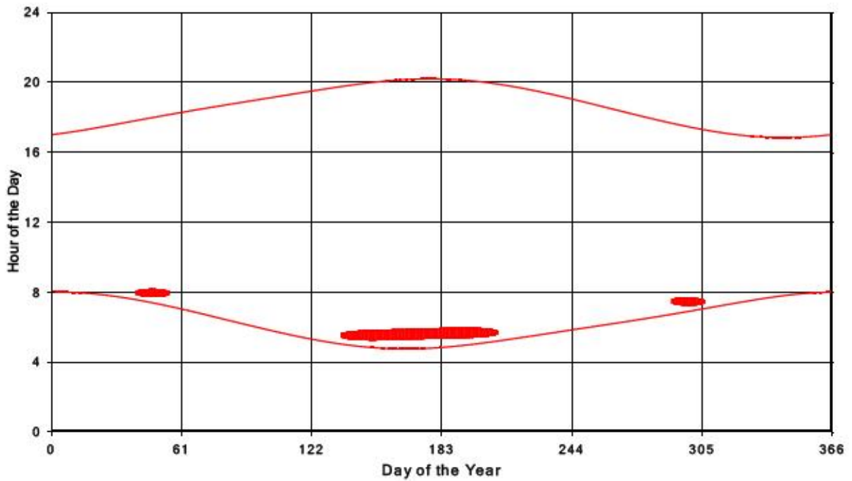
Bluewater Wind Energy Centre Shadow Times on Receptor 197, All Windows from All Turbine
