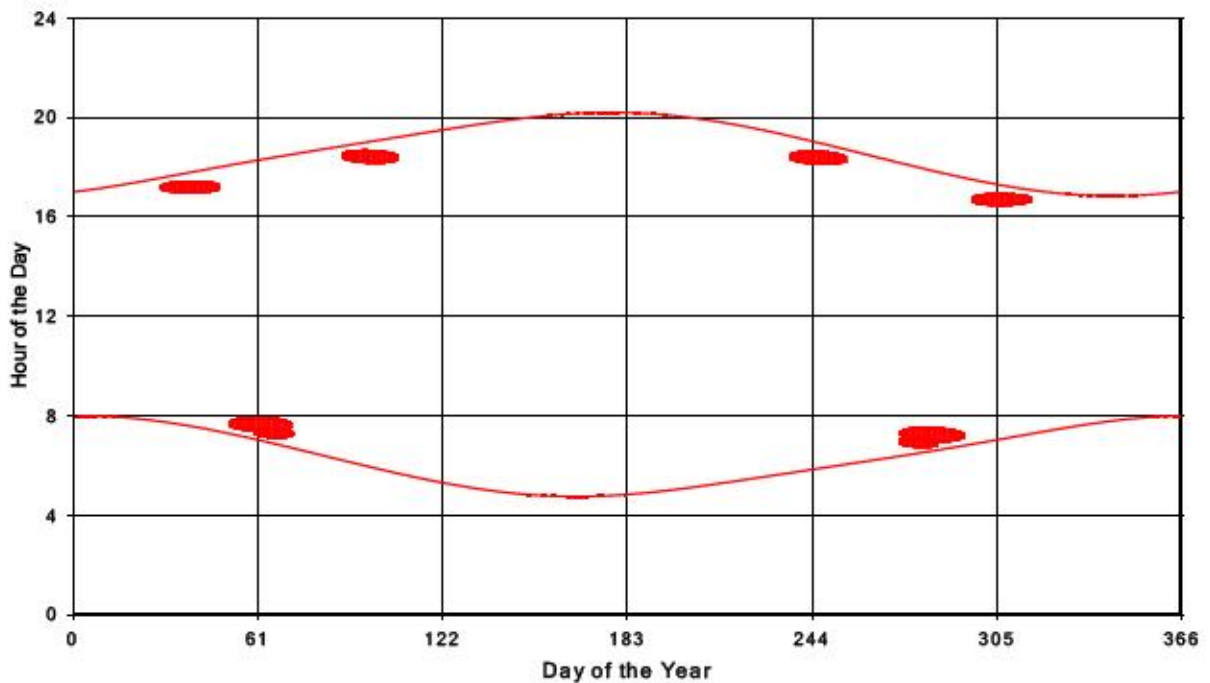
Bluewater Wind Energy Centre Shadow Times on Receptor 288, All Windows from All Turbine
