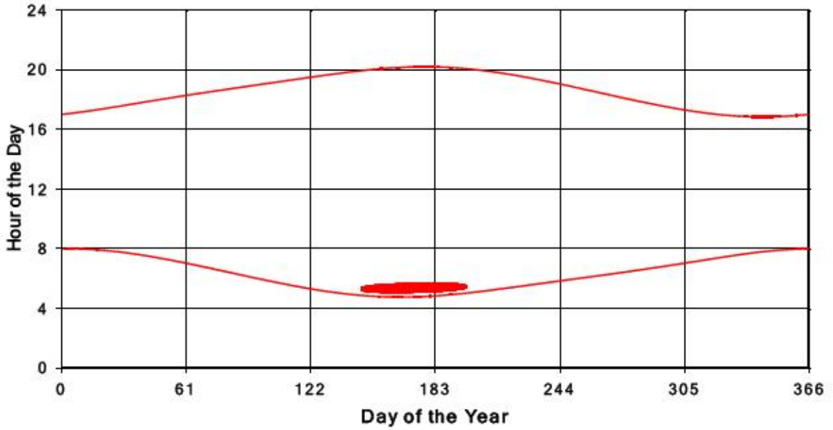
Bluewater Wind Energy Centre Shadow Times on Receptor 235, All Windows from All Turbine
