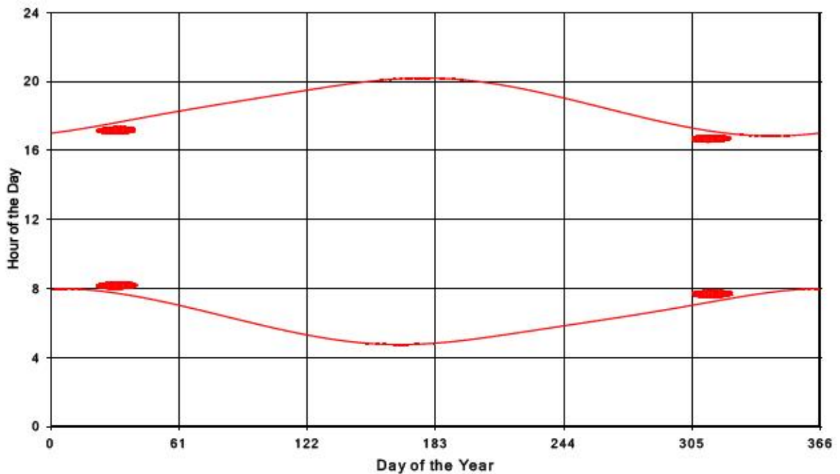
Bluewater Wind Energy Centre Shadow Times on Receptor 146, All Windows from All Turbine
