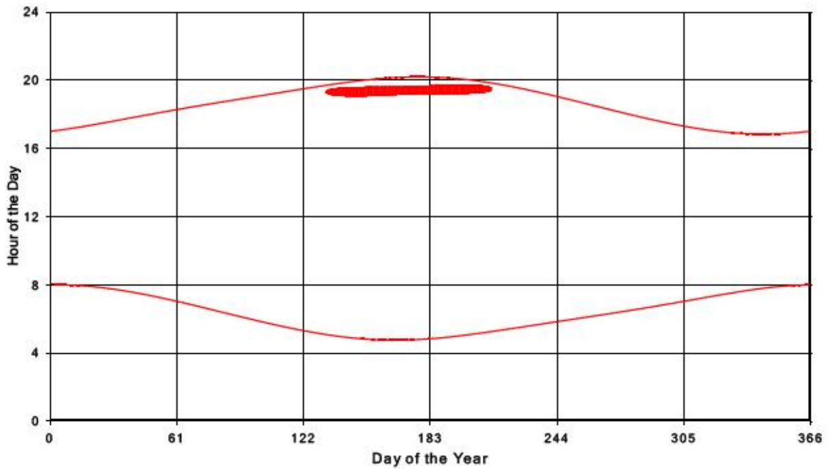
Bluewater Wind Energy Centre Shadow Times on Receptor 407, All Windows from All Turbine
