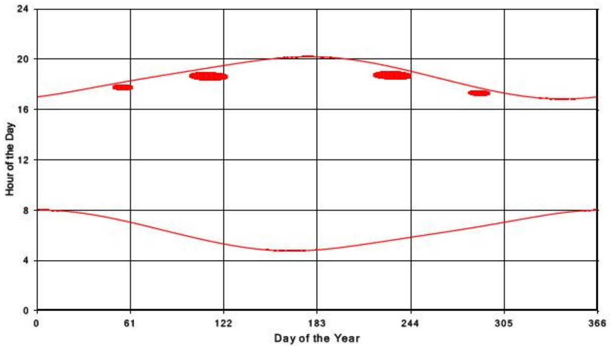
Bluewater Wind Energy Centre Shadow Times on Receptor 294, All Windows from All Turbine
