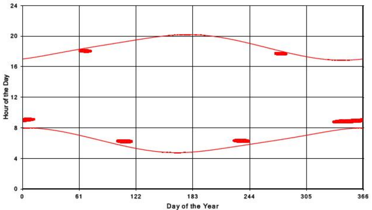
Bluewater Wind Energy Centre Shadow Times on Receptor 350, All Windows from All Turbine
