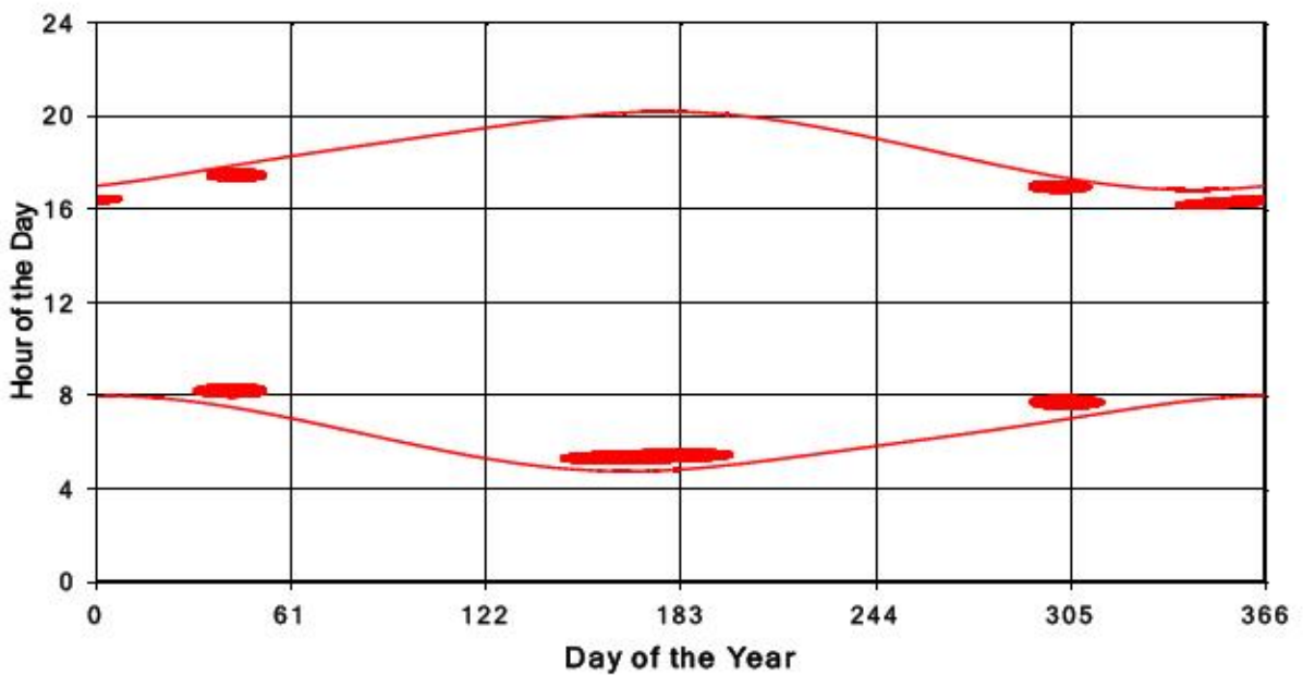
Bluewater Wind Energy Centre Shadow Times on Receptor 192, All Windows from All Turbine
