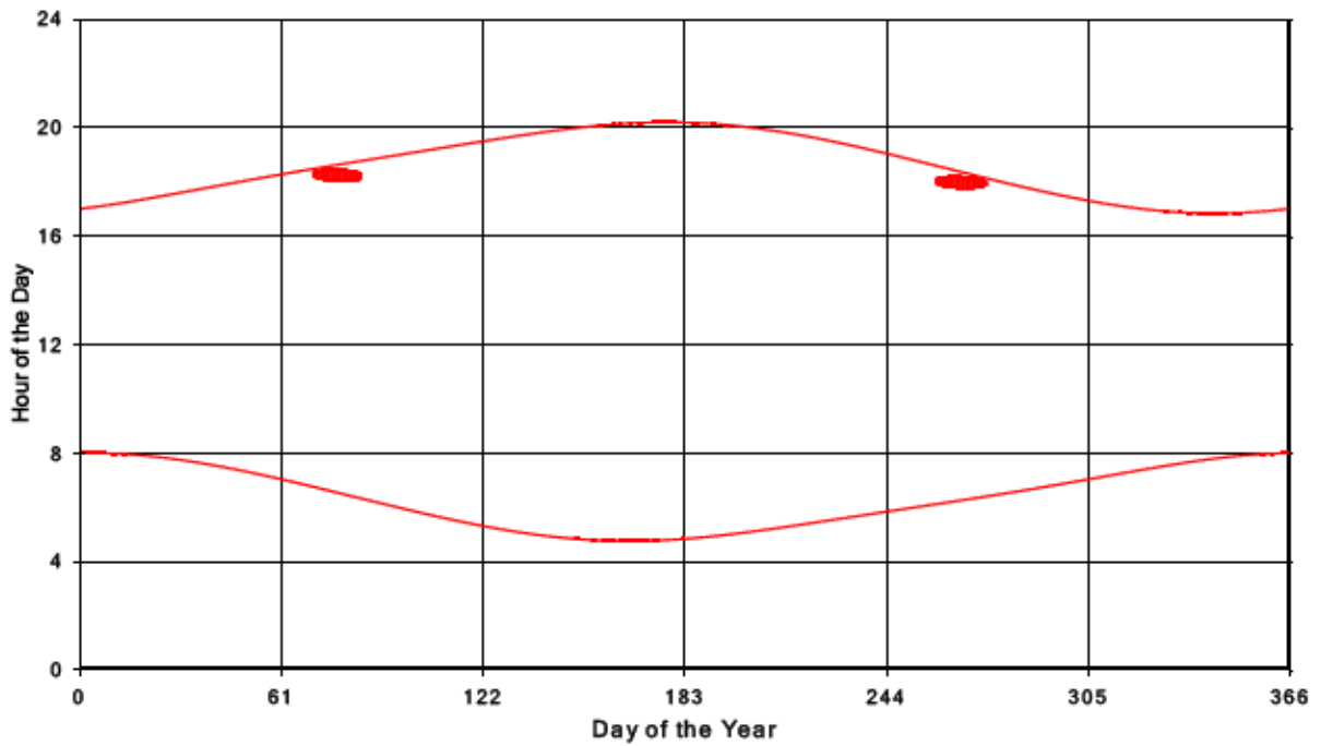
Bluewater Wind Energy Centre Shadow Times on Receptor 79, All Windows from All Turbine:
