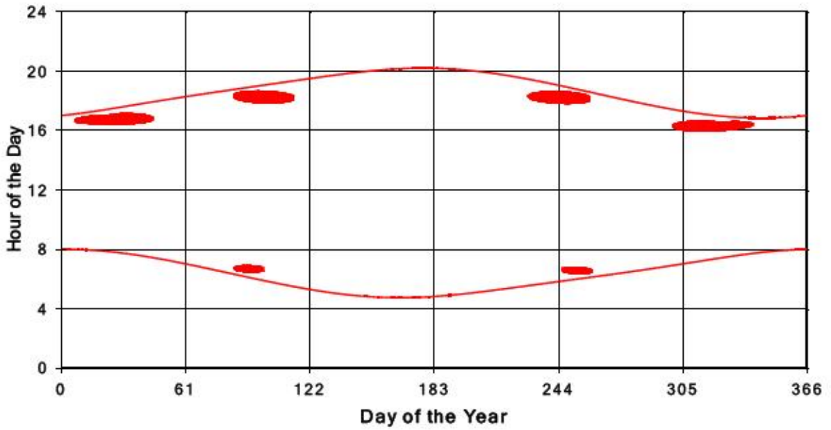
Bluewater Wind Energy Centre Shadow Times on Receptor 239, All Windows from All Turbine
