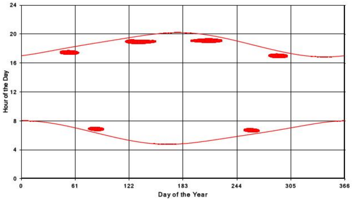
Bluewater Wind Energy Centre Shadow Times on Receptor 379, All Windows from All Turbine
