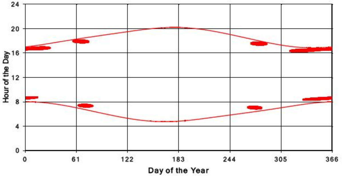
Bluewater Wind Energy Centre Shadow Times on Receptor 29, All Windows from All Turbine
