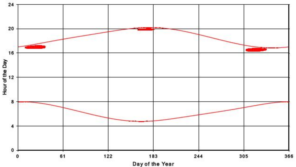
Bluewater Wind Energy Centre Shadow Times on Receptor 206, All Windows from All Turbine
