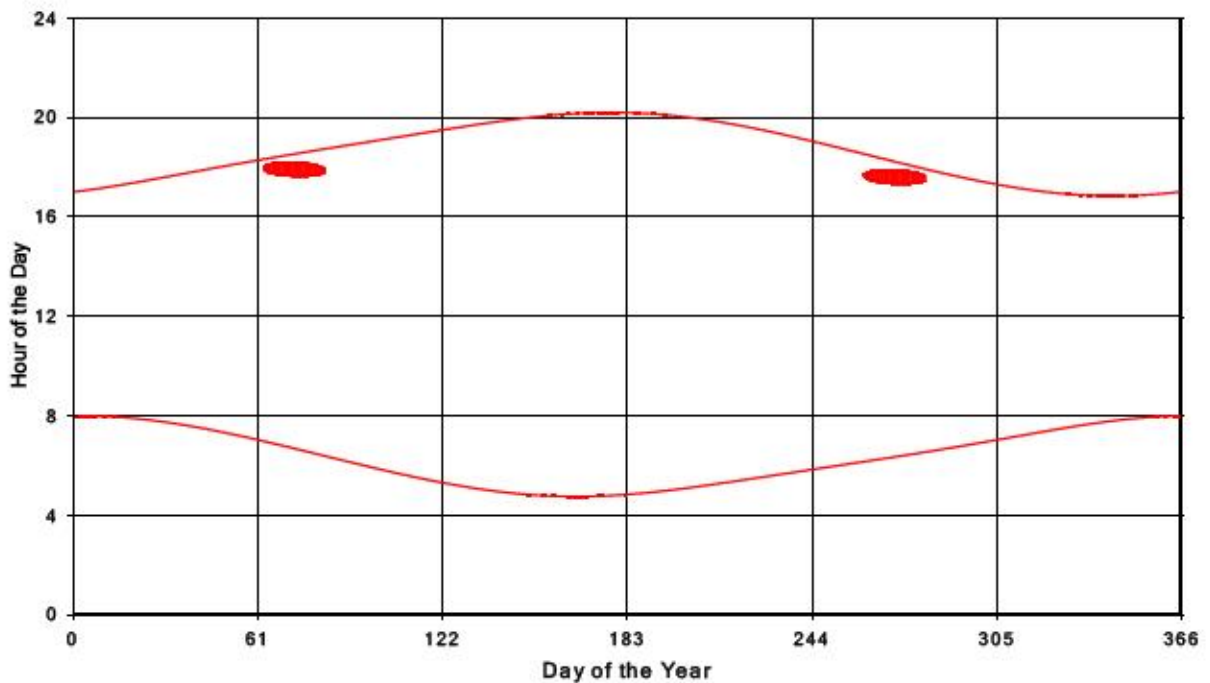
Bluewater Wind Energy Centre Shadow Times on Receptor 246, All Windows from All Turbine
