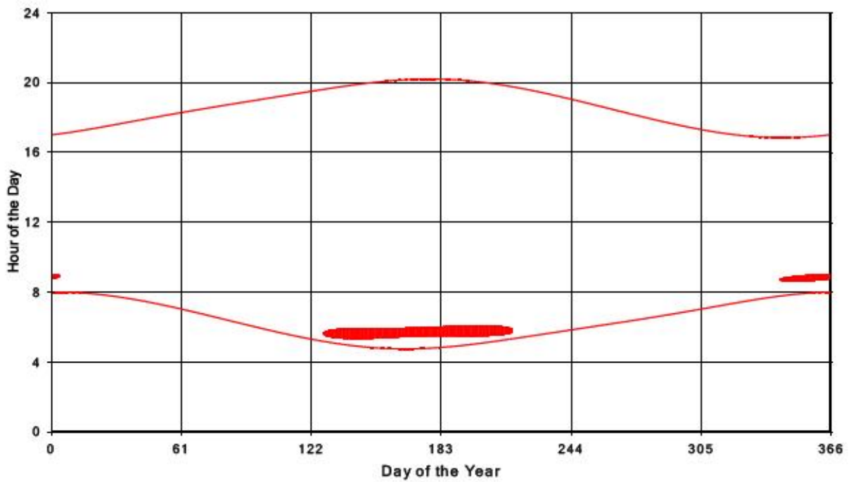
Bluewater Wind Energy Centre Shadow Times on Receptor 255, All Windows from All Turbine
