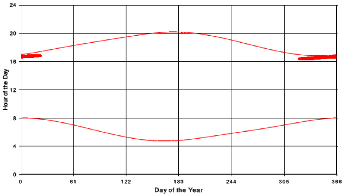
Bluewater Wind Energy Centre Shadow Times on Receptor 69, All Windows from All Turbine:
