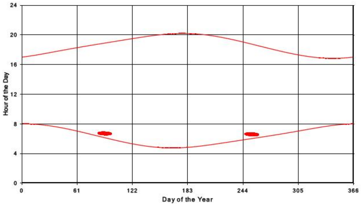
Bluewater Wind Energy Centre Shadow Times on Receptor 33, All Windows from All Turbine:
