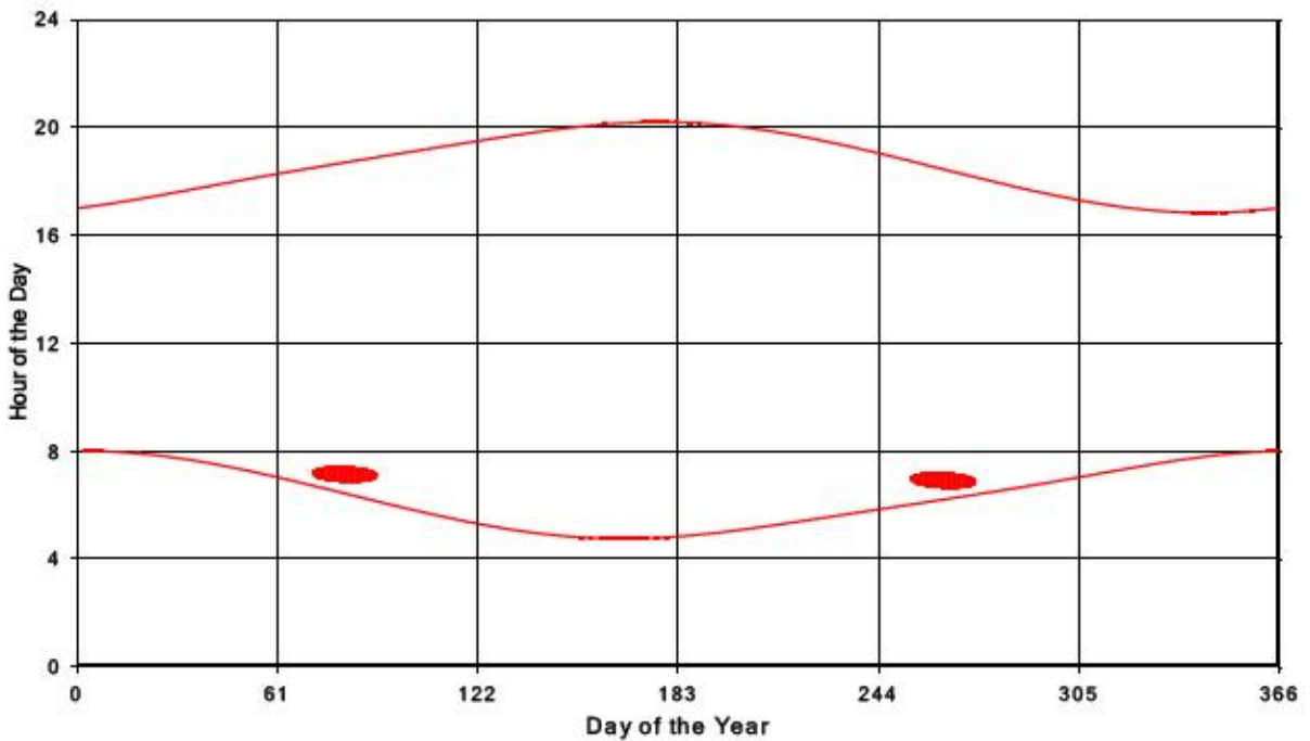
Bluewater Wind Energy Centre Shadow Times on Receptor 20, All Windows from All Turbine:
