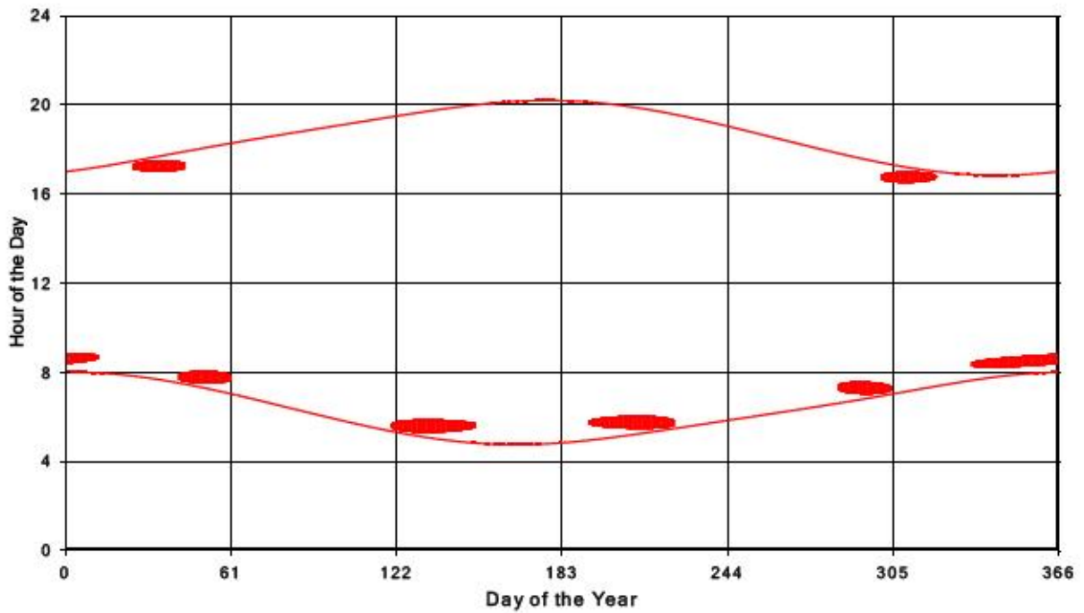
Bluewater Wind Energy Centre Shadow Times on Receptor 111, All Windows from All Turbine
