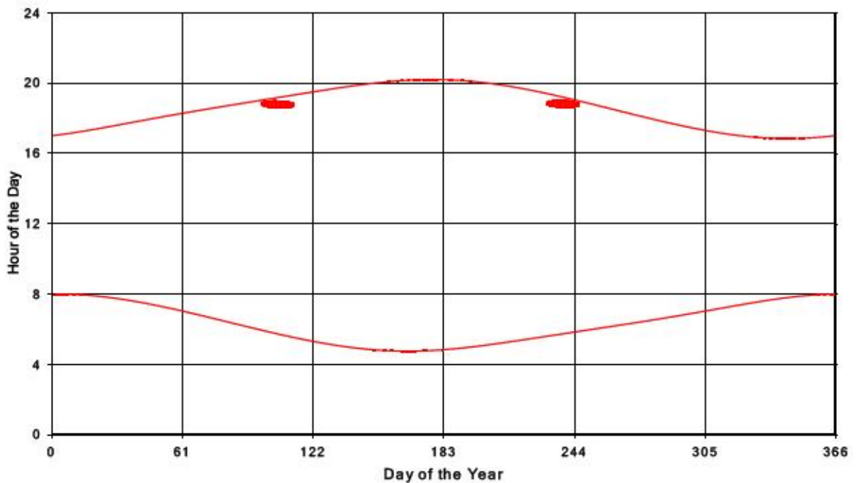
Bluewater Wind Energy Centre Shadow Times on Receptor 360, All Windows from All Turbine
