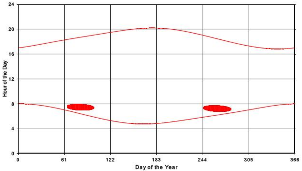
Bluewater Wind Energy Centre Shadow Times on Receptor 385, All Windows from All Turbine
