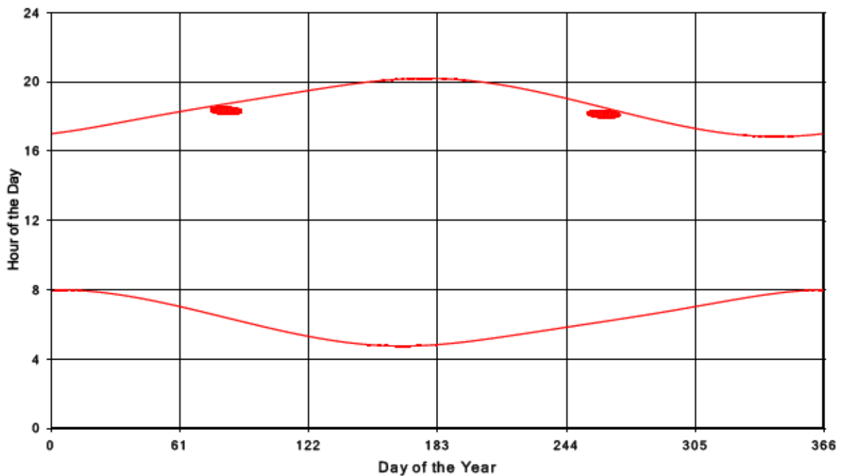
Bluewater Wind Energy Centre Shadow Times on Receptor 80, All Windows from All Turbine:
