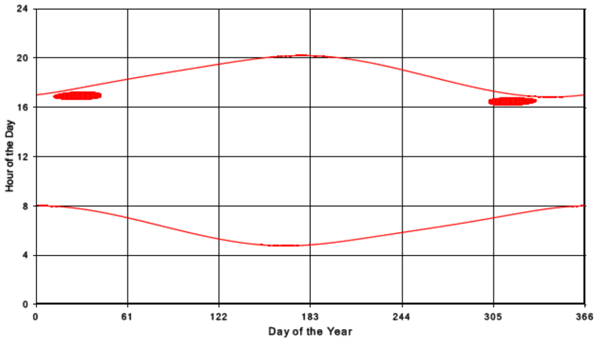
Bluewater Wind Energy Centre Shadow Times on Receptor 68, All Windows from All Turbine:
