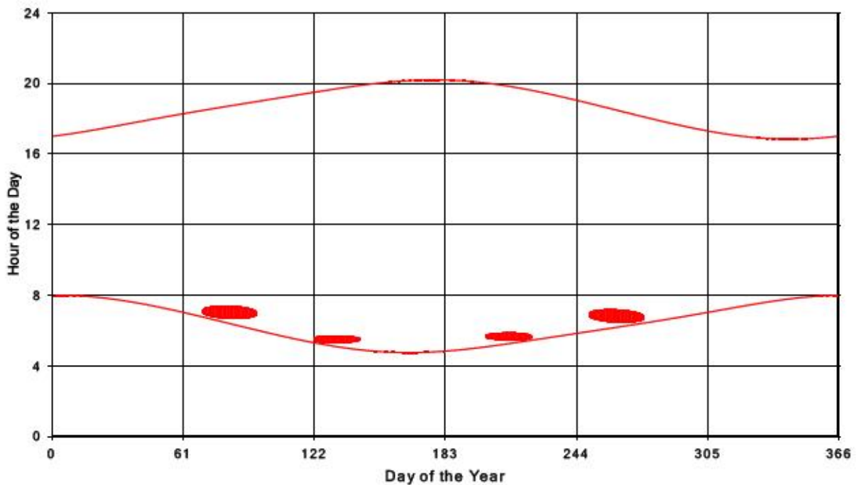
Bluewater Wind Energy Centre Shadow Times on Receptor 368, All Windows from All Turbine
