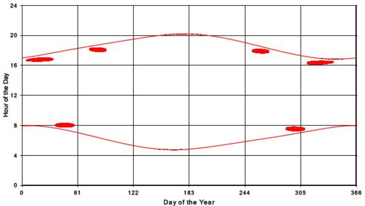
Bluewater Wind Energy Centre Shadow Times on Receptor 134, All Windows from All Turbine
