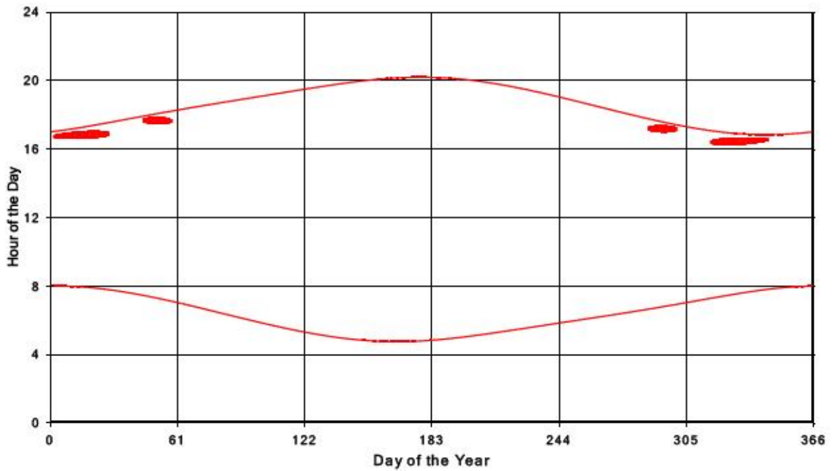
Bluewater Wind Energy Centre Shadow Times on Receptor 133, All Windows from All Turbine
