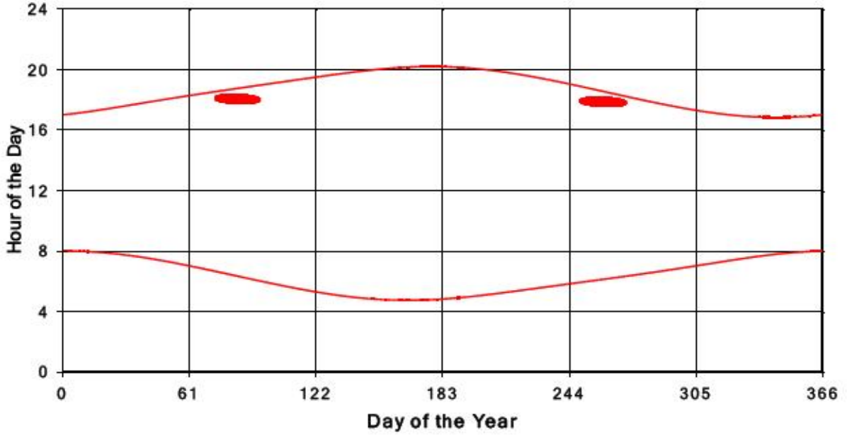
Bluewater Wind Energy Centre Shadow Times on Receptor 234, All Windows from All Turbine
