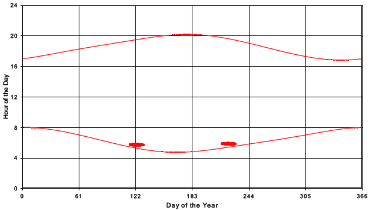
Bluewater Wind Energy Centre Shadow Times on Receptor 296, All Windows from All Turbine
