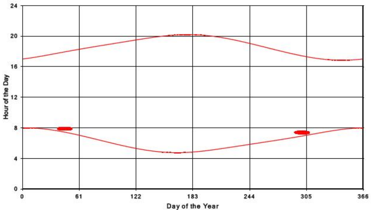
Bluewater Wind Energy Centre Shadow Times on Receptor 275, All Windows from All Turbine
