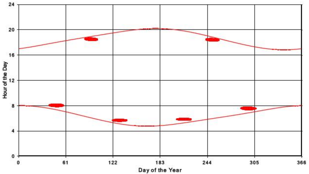
Bluewater Wind Energy Centre Shadow Times on Receptor 349, All Windows from All Turbine
