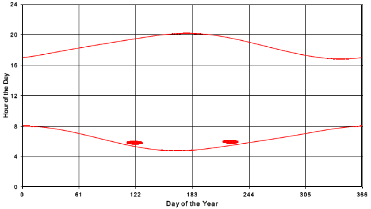
Bluewater Wind Energy Centre Shadow Times on Receptor 1, All Windows from All Turbine:
