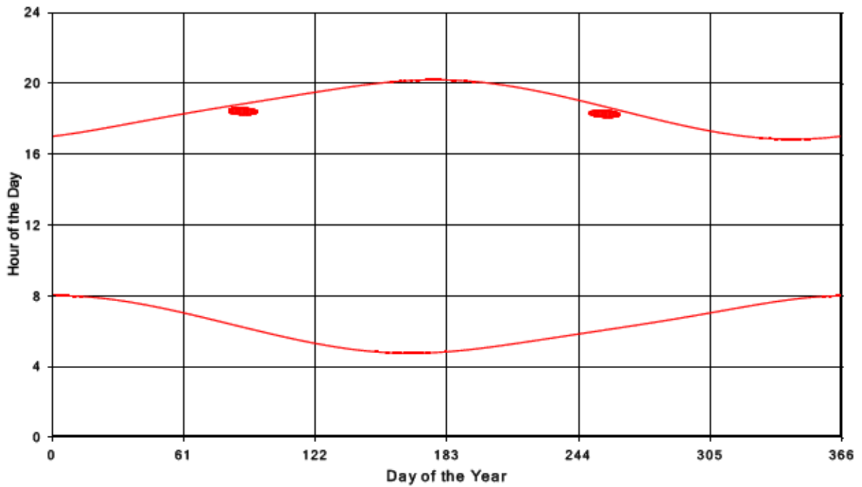
Bluewater Wind Energy Centre Shadow Times on Receptor 311, All Windows from All Turbine
