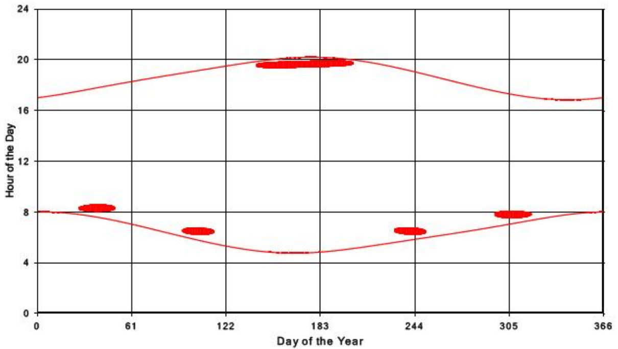
Bluewater Wind Energy Centre Shadow Times on Receptor 258, All Windows from All Turbine
