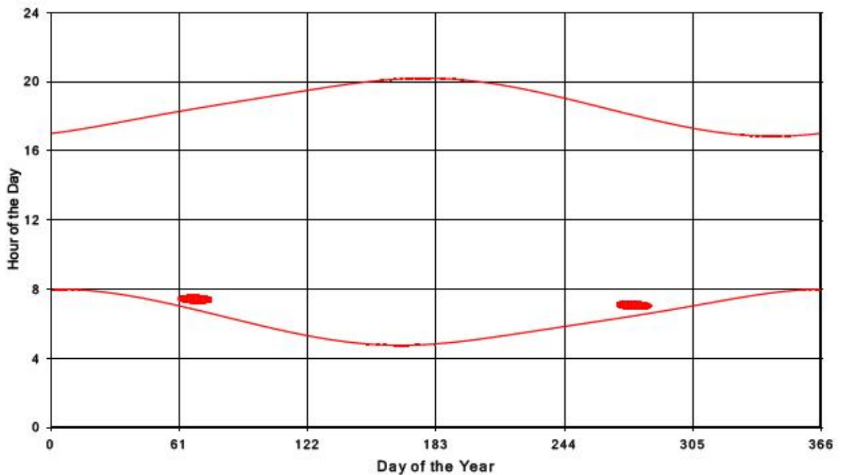
Bluewater Wind Energy Centre Shadow Times on Receptor 354, All Windows from All Turbine
