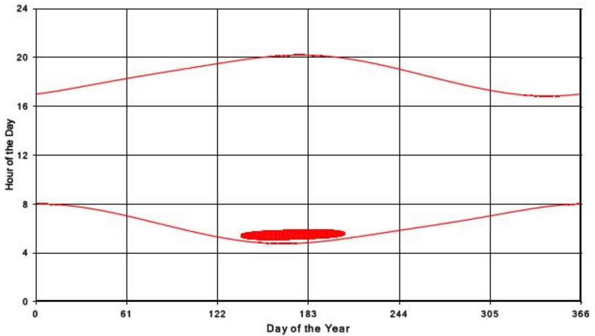
Bluewater Wind Energy Centre Shadow Times on Receptor 247, All Windows from All Turbine
