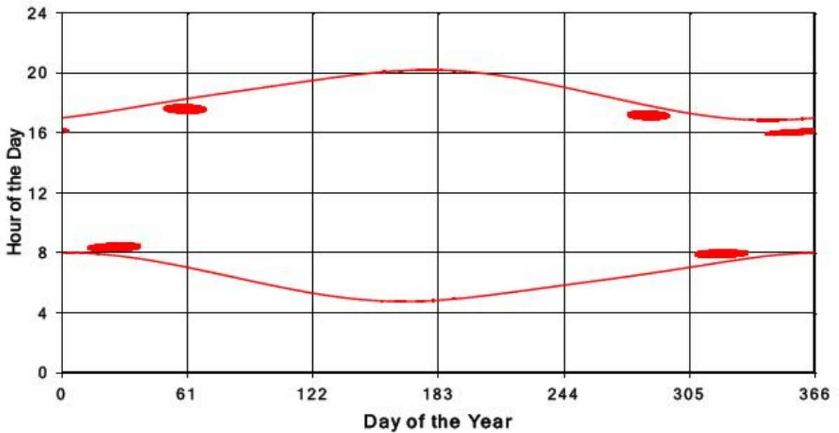
Bluewater Wind Energy Centre Shadow Times on Receptor 233, All Windows from All Turbine
