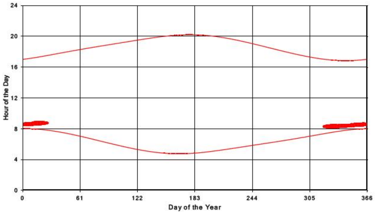
Bluewater Wind Energy Centre Shadow Times on Receptor 338, All Windows from All Turbine
