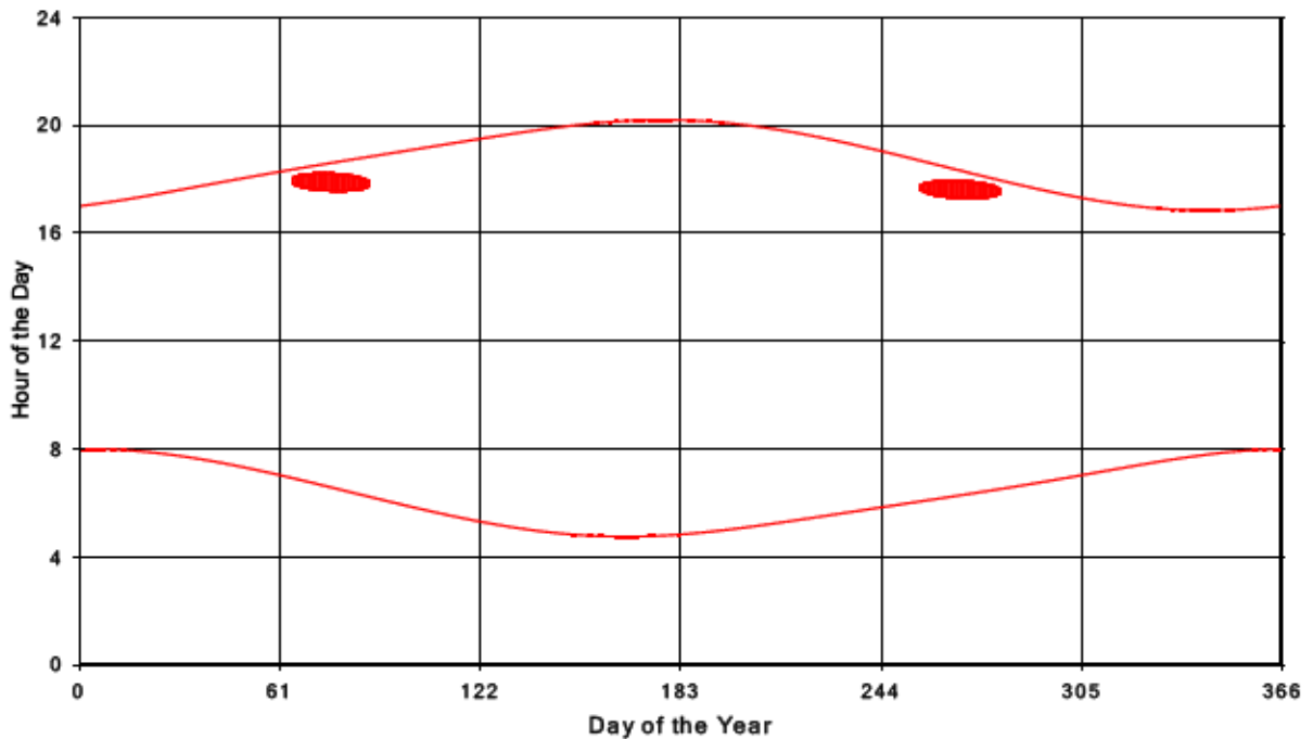
Bluewater Wind Energy Centre Shadow Times on Receptor 150, All Windows from All Turbine
