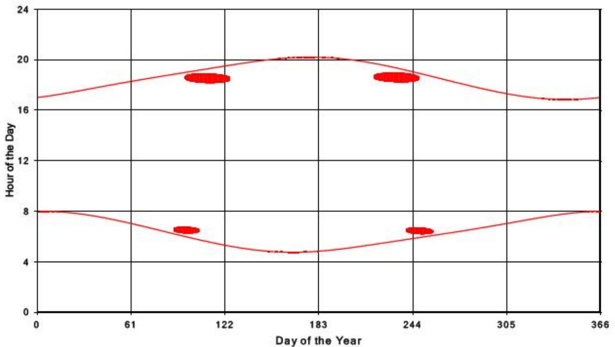
Bluewater Wind Energy Centre Shadow Times on Receptor 253, All Windows from All Turbine
