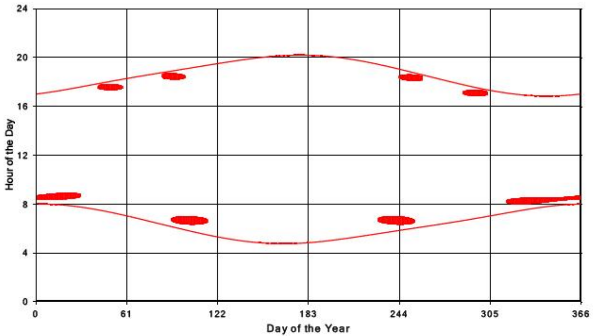
Bluewater Wind Energy Centre Shadow Times on Receptor 35, All Windows from All Turbine:
