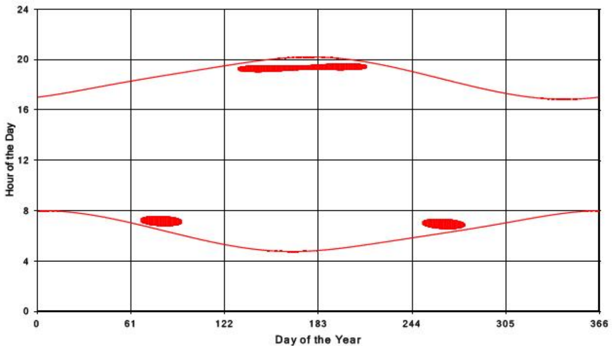
Bluewater Wind Energy Centre Shadow Times on Receptor 392, All Windows from All Turbine
