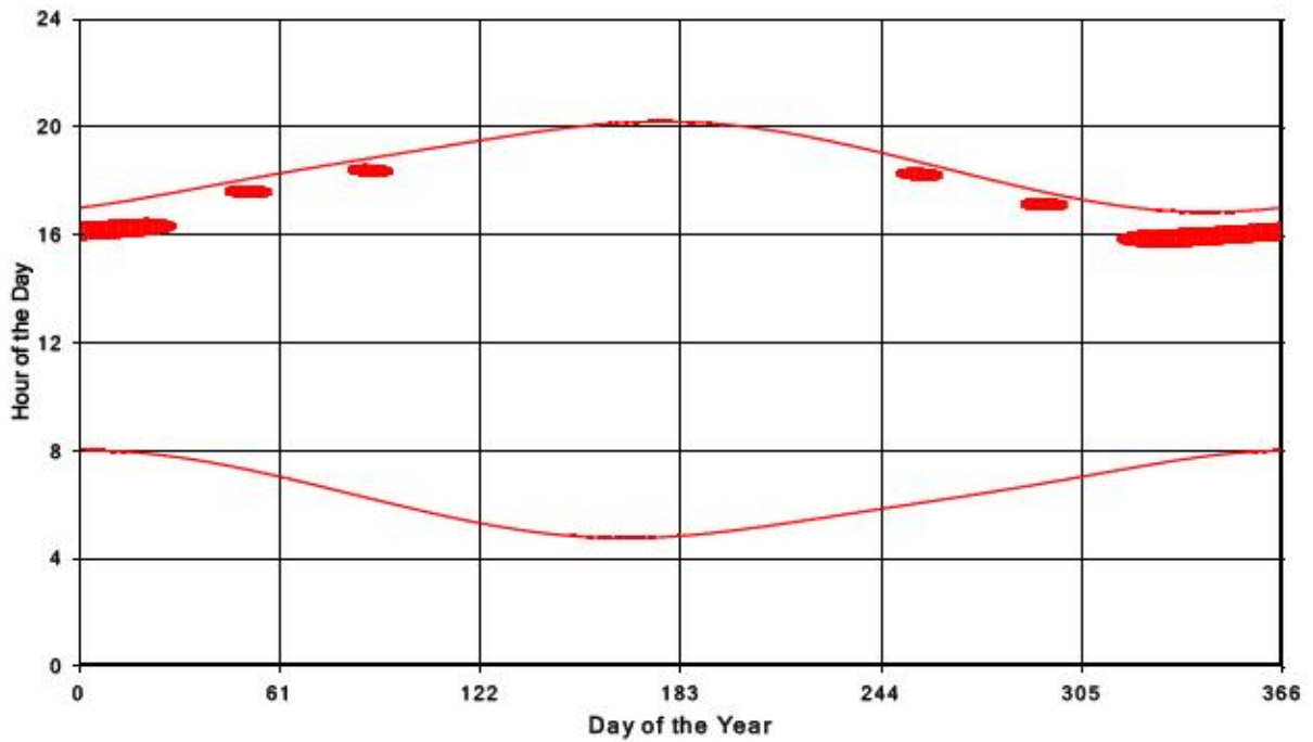
Bluewater Wind Energy Centre Shadow Times on Receptor 395, All Windows from All Turbine
