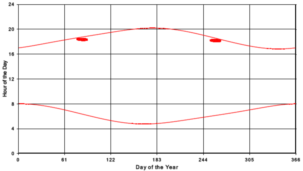
Bluewater Wind Energy Centre Shadow Times on Receptor 91, All Windows from All Turbine:
