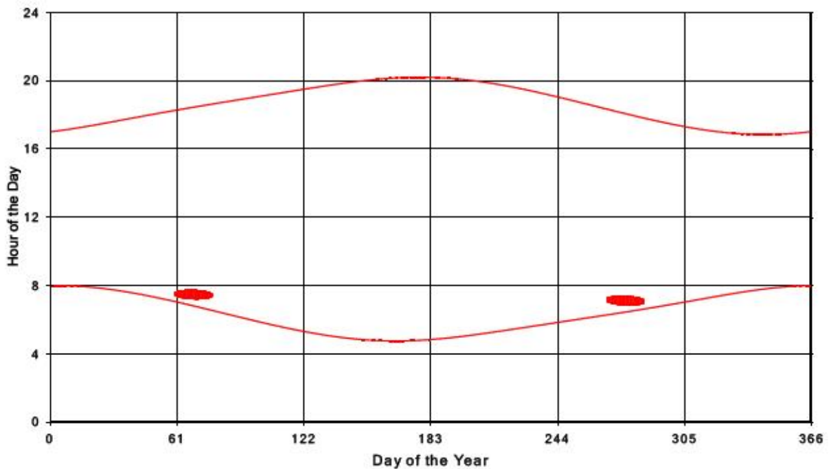
Bluewater Wind Energy Centre Shadow Times on Receptor 42, All Windows from All Turbine:
