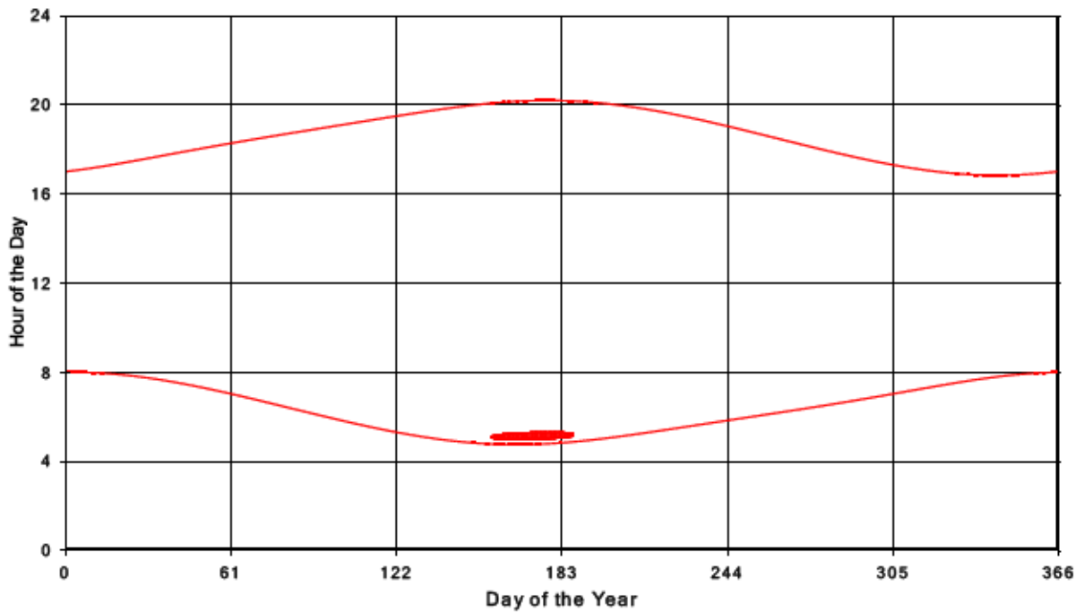
Bluewater Wind Energy Centre Shadow Times on Receptor 314, All Windows from All Turbine
