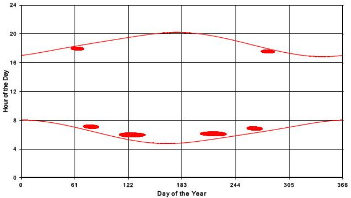
Bluewater Wind Energy Centre Shadow Times on Receptor 355, All Windows from All Turbine
