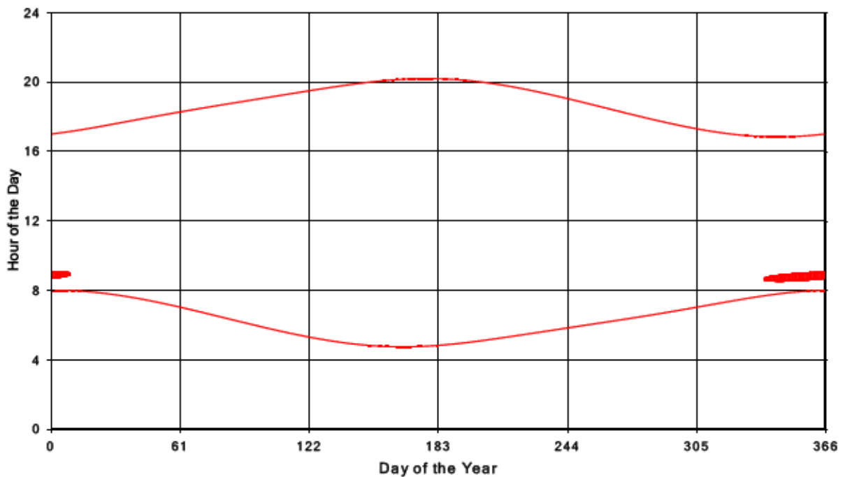
Bluewater Wind Energy Centre Shadow Times on Receptor 336, All Windows from All Turbine
