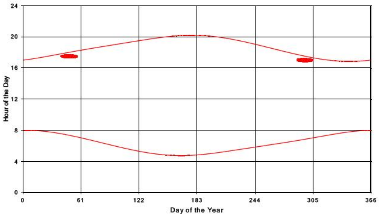
Bluewater Wind Energy Centre Shadow Times on Receptor 248, All Windows from All Turbine
