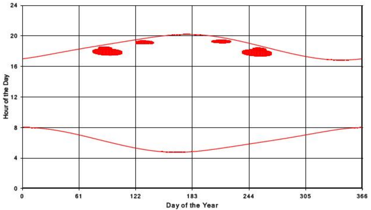
Bluewater Wind Energy Centre Shadow Times on Receptor 399, All Windows from All Turbine
