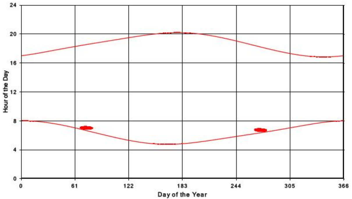
Bluewater Wind Energy Centre Shadow Times on Receptor 363, All Windows from All Turbine
