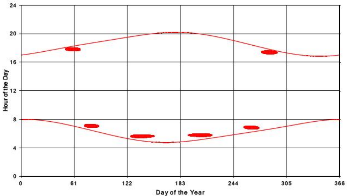
Bluewater Wind Energy Centre Shadow Times on Receptor 48, All Windows from All Turbine:
