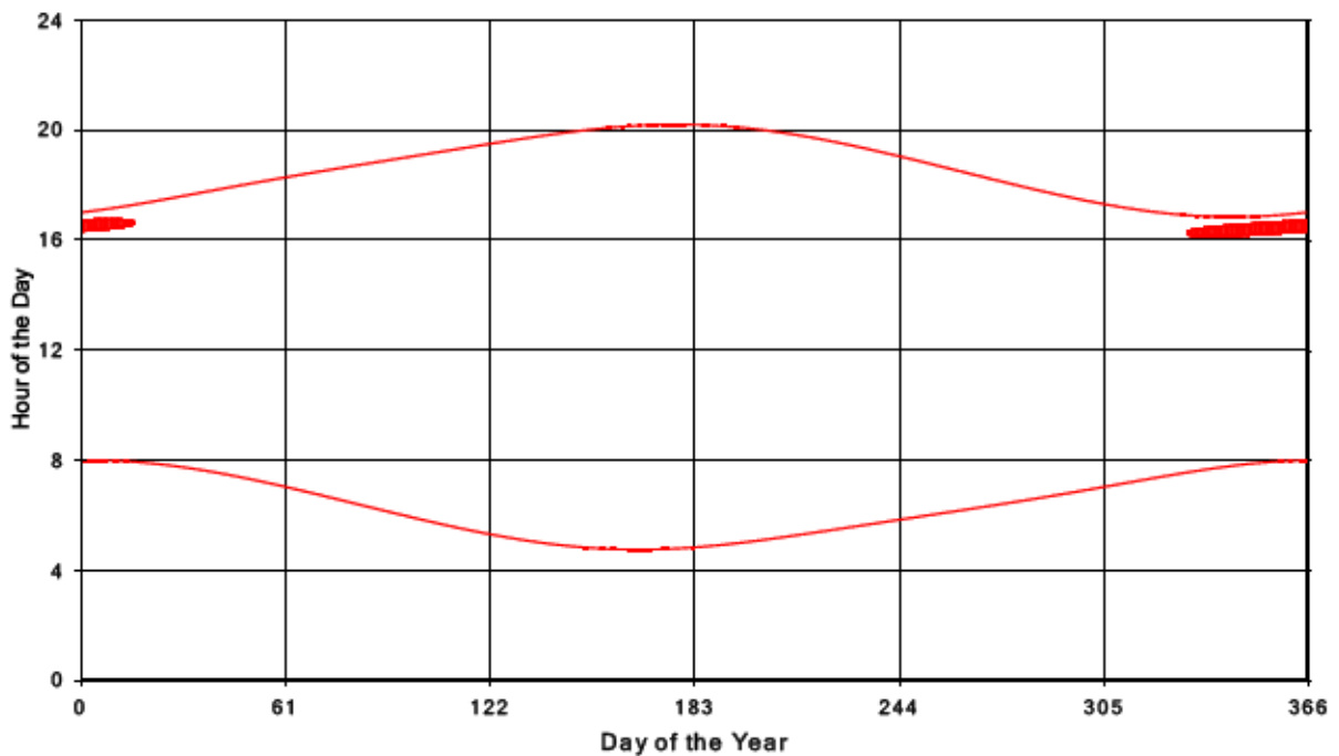
Bluewater Wind Energy Centre Shadow Times on Receptor 63, All Windows from All Turbine:
