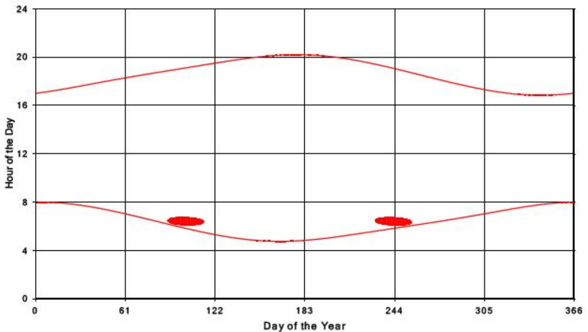
Bluewater Wind Energy Centre Shadow Times on Receptor 107, All Windows from All Turbine
