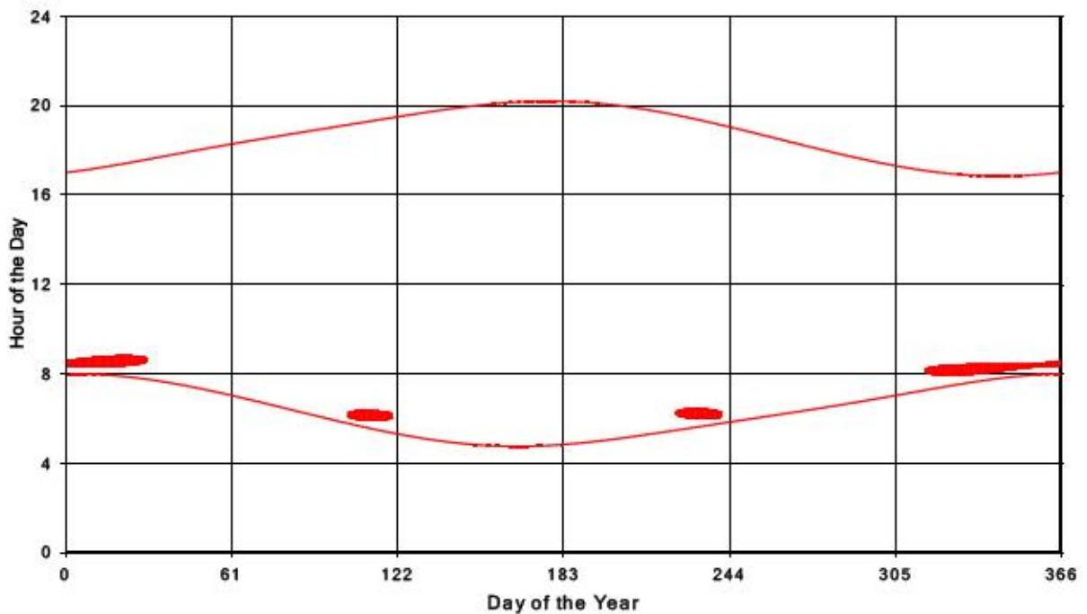
Bluewater Wind Energy Centre Shadow Times on Receptor 38, All Windows from All Turbine:
