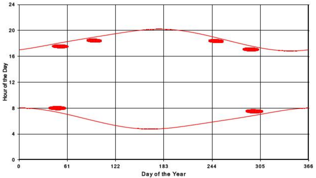
Bluewater Wind Energy Centre Shadow Times on Receptor 180, All Windows from All Turbine
