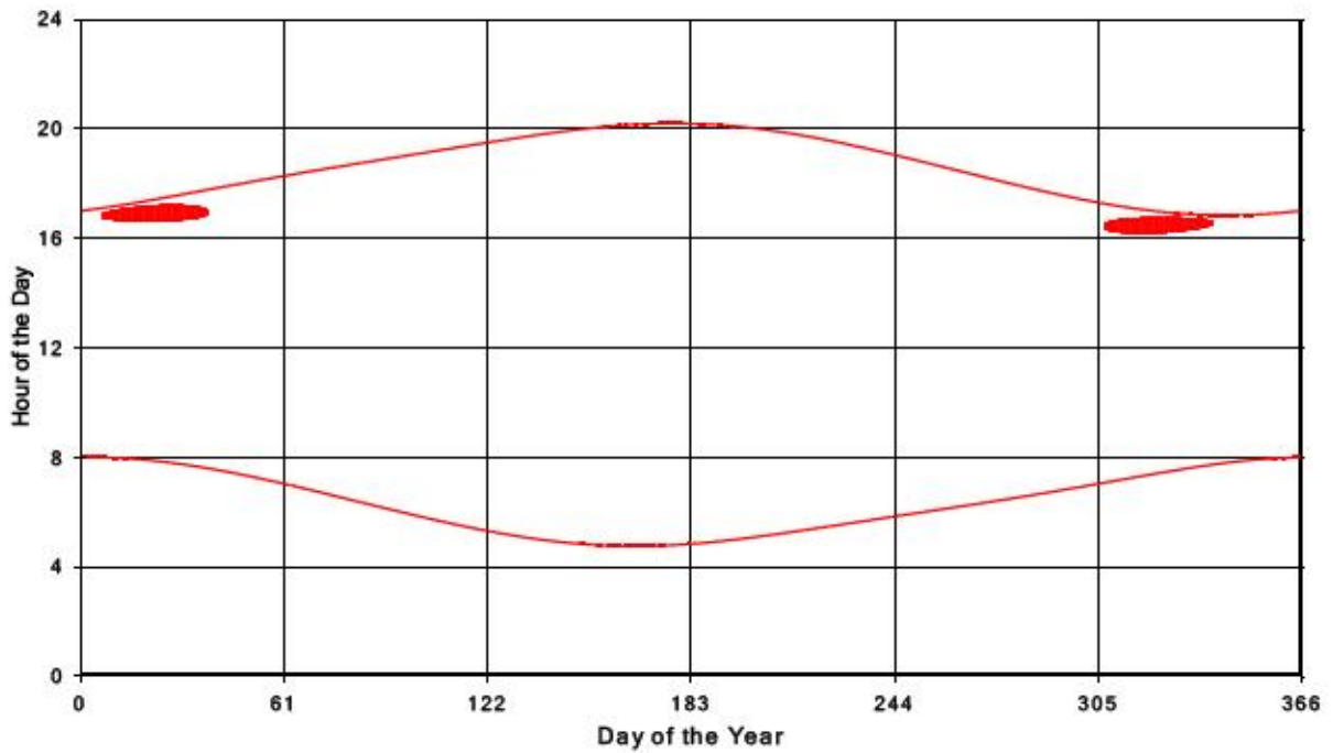
Bluewater Wind Energy Centre Shadow Times on Receptor 205, All Windows from All Turbine
