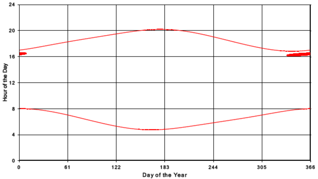
Bluewater Wind Energy Centre Shadow Times on Receptor 60, All Windows from All Turbine:
