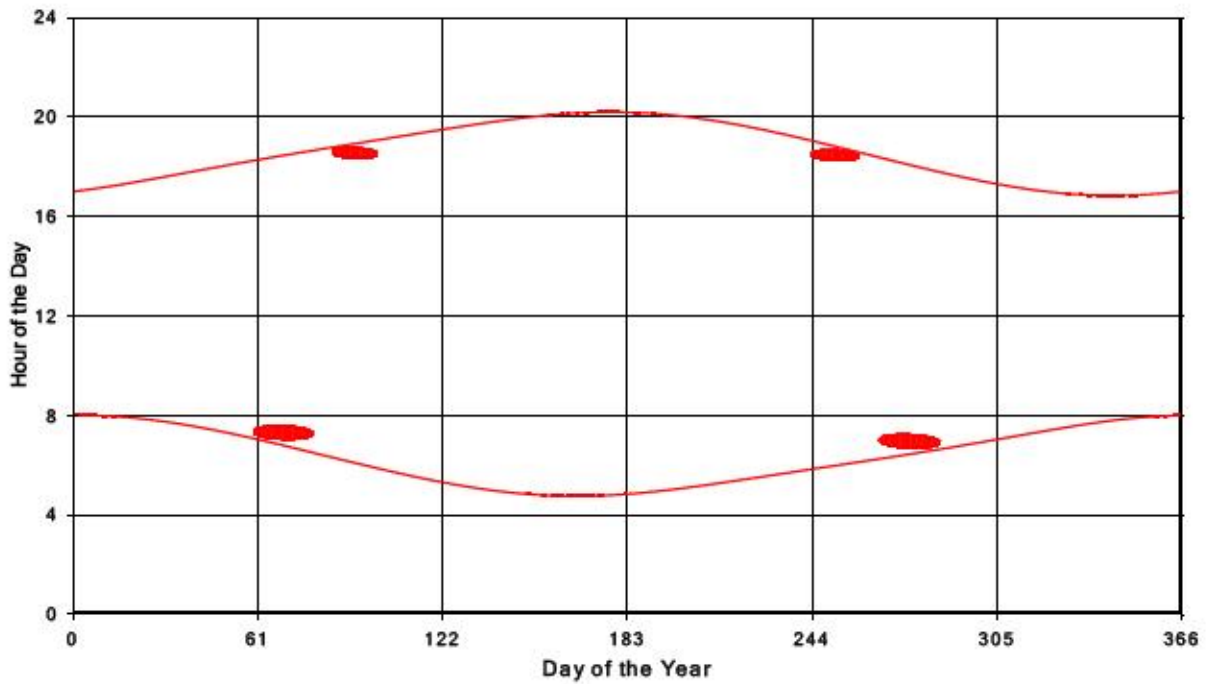
Bluewater Wind Energy Centre Shadow Times on Receptor 103, All Windows from All Turbine
