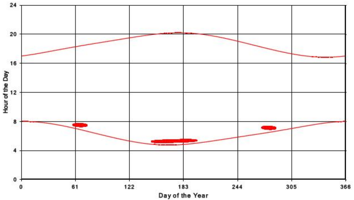
Bluewater Wind Energy Centre Shadow Times on Receptor 37, All Windows from All Turbine:
