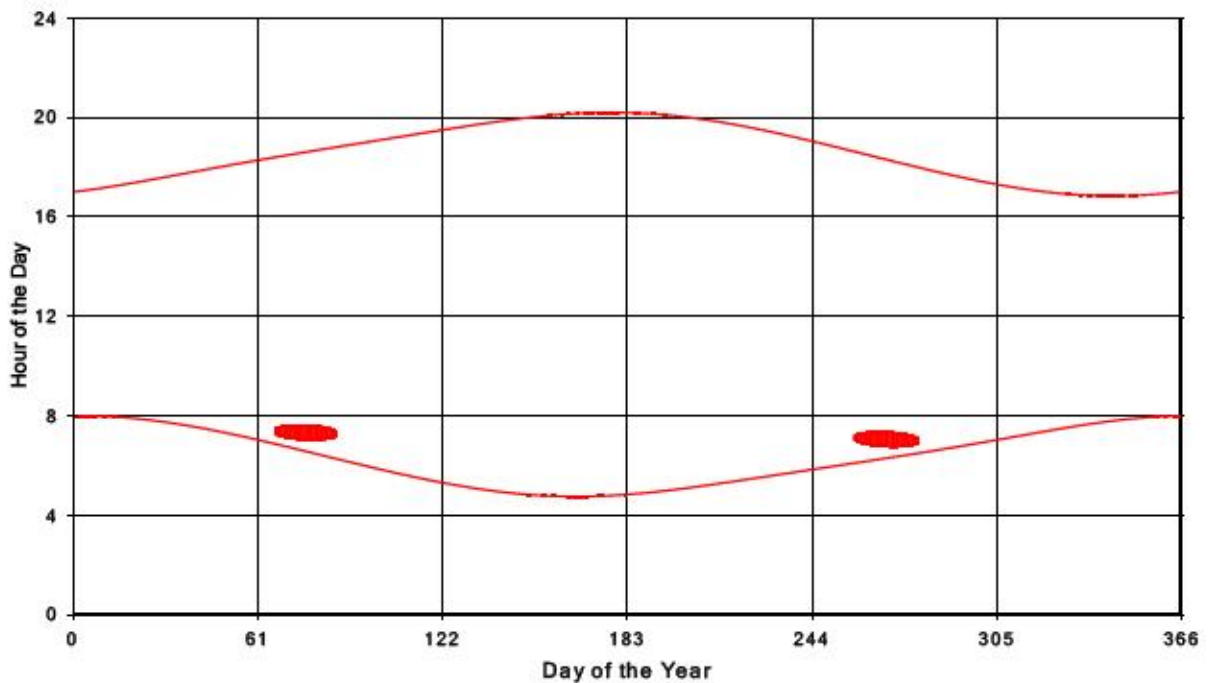
Bluewater Wind Energy Centre Shadow Times on Receptor 23, All Windows from All Turbine:
