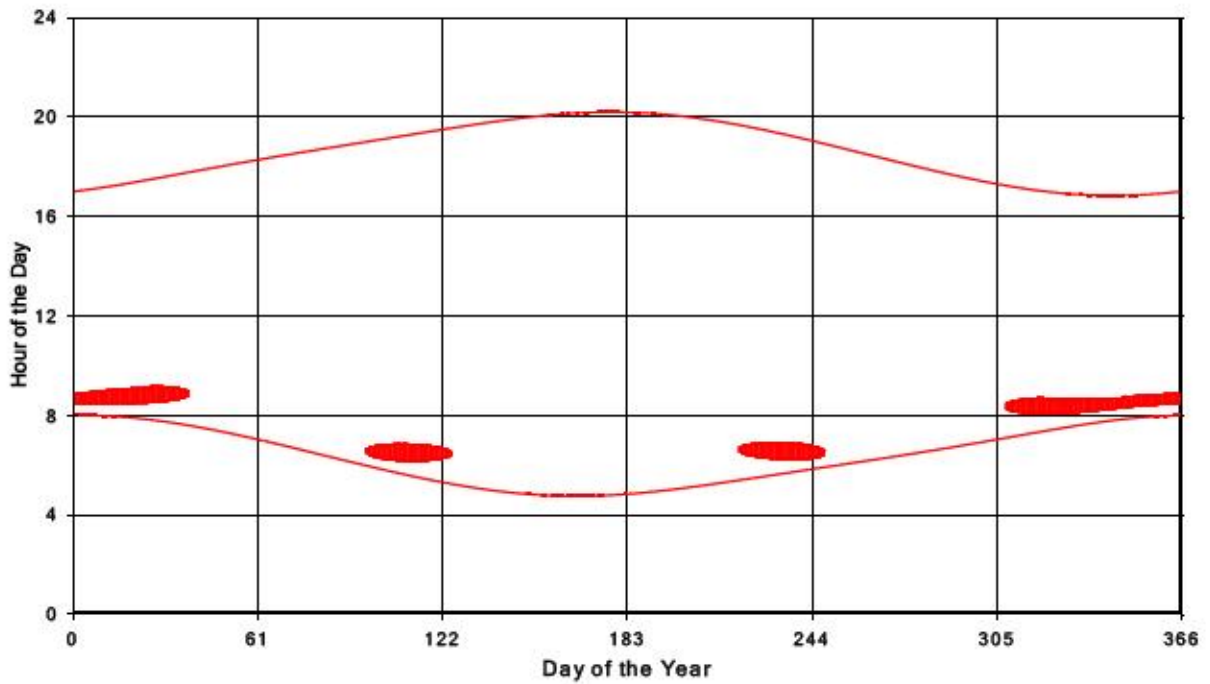
Bluewater Wind Energy Centre Shadow Times on Receptor 351, All Windows from All Turbine
