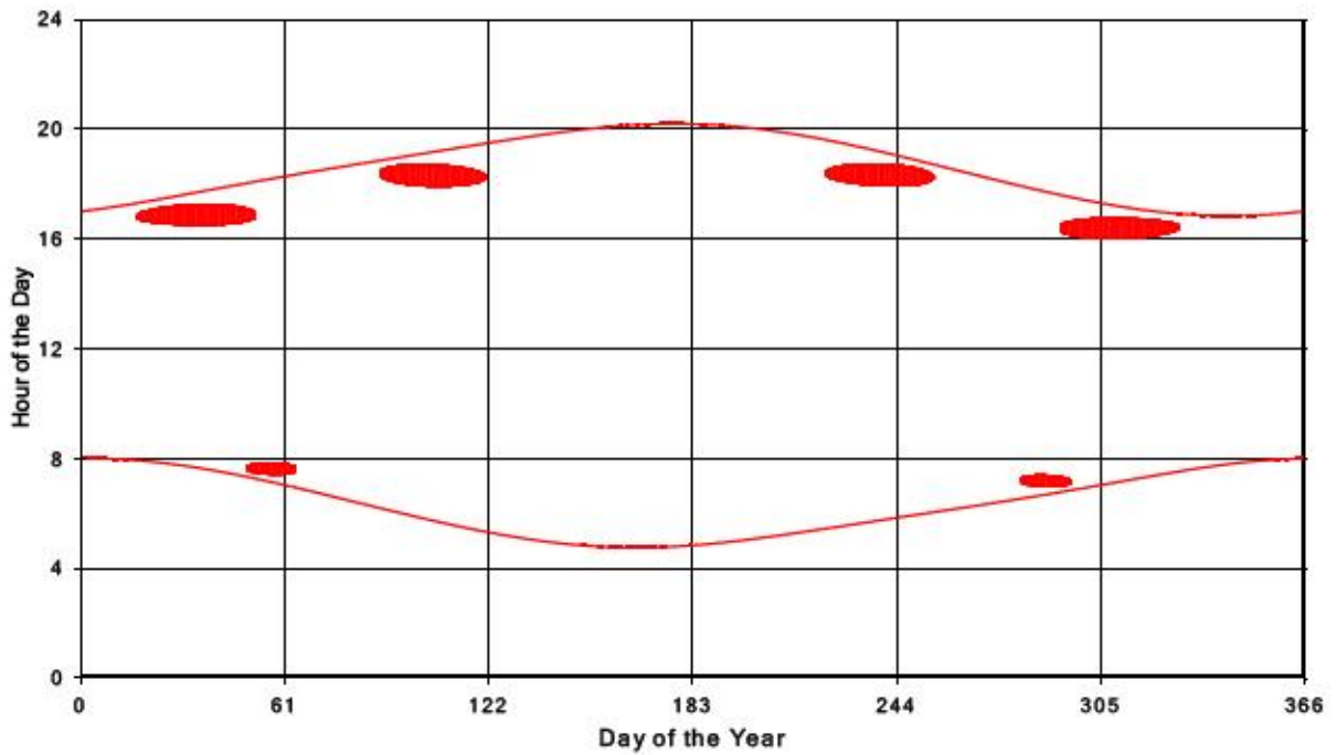
Bluewater Wind Energy Centre Shadow Times on Receptor 252, All Windows from All Turbine
