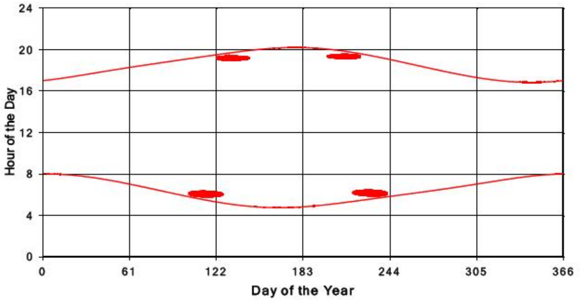
Bluewater Wind Energy Centre Shadow Times on Receptor 227, All Windows from All Turbine
