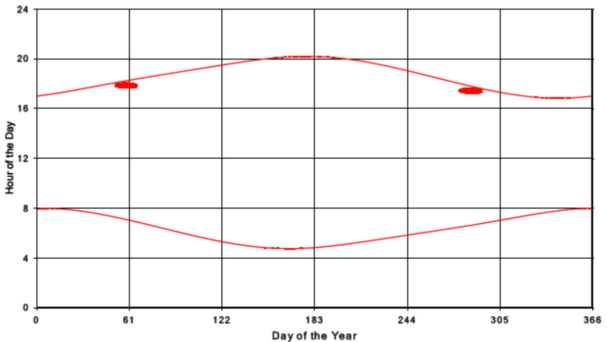
Bluewater Wind Energy Centre Shadow Times on Receptor 266, All Windows from All Turbine
