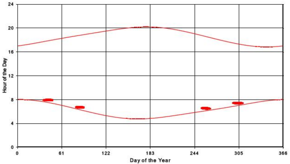
Bluewater Wind Energy Centre Shadow Times on Receptor 213, All Windows from All Turbine
