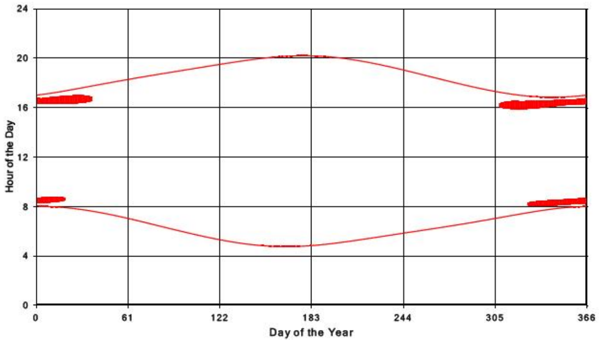
Bluewater Wind Energy Centre Shadow Times on Receptor 171, All Windows from All Turbine
