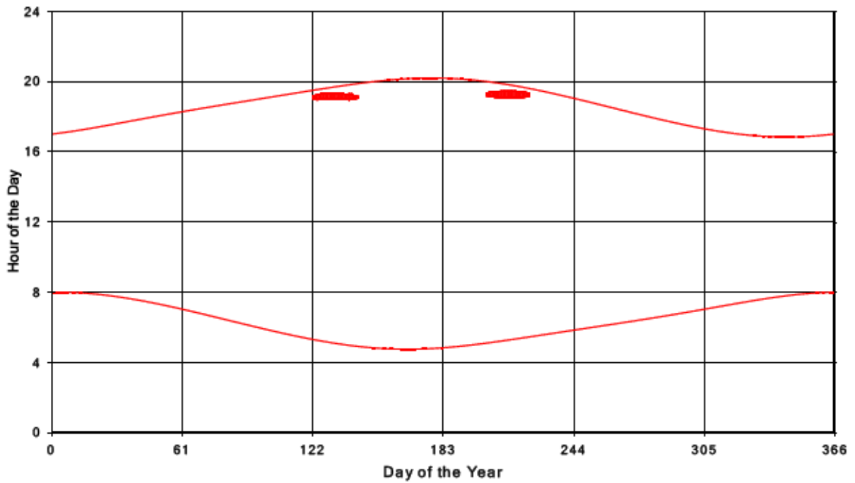
Bluewater Wind Energy Centre Shadow Times on Receptor 320, All Windows from All Turbine
