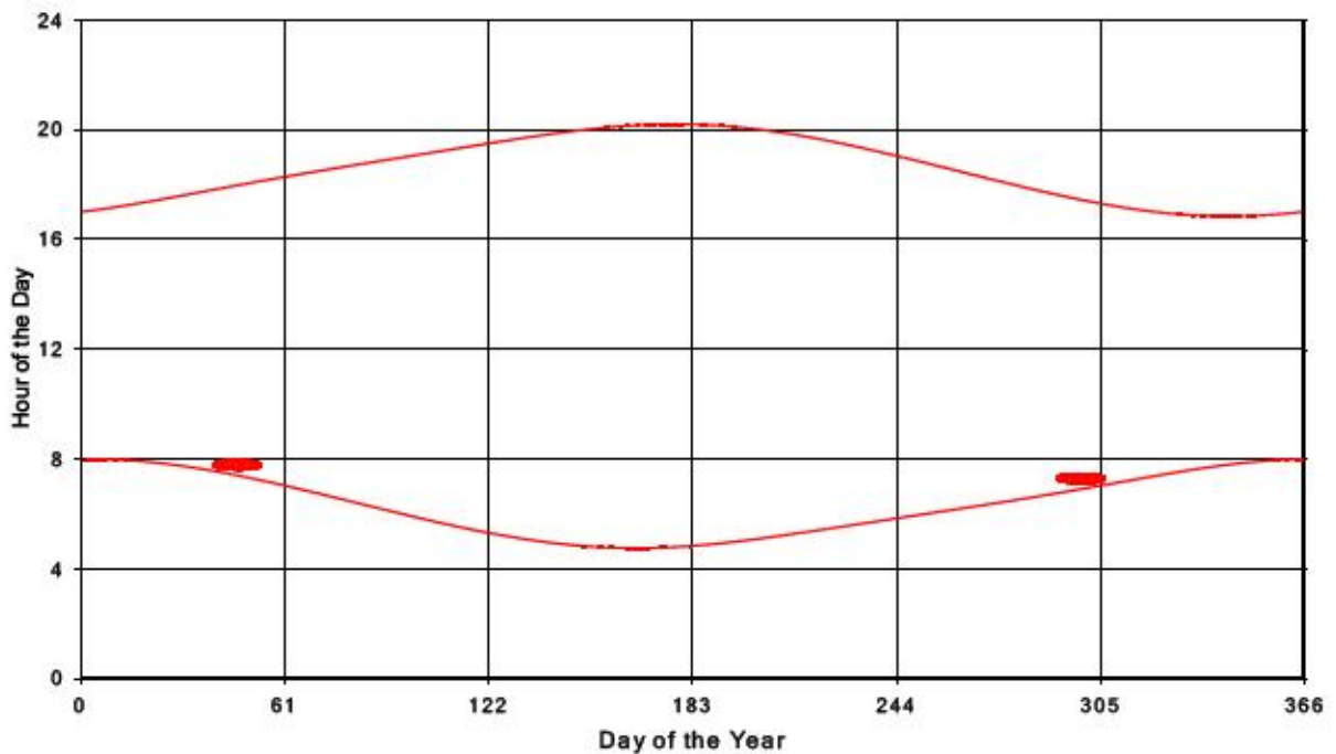
Bluewater Wind Energy Centre Shadow Times on Receptor 217, All Windows from All Turbine
