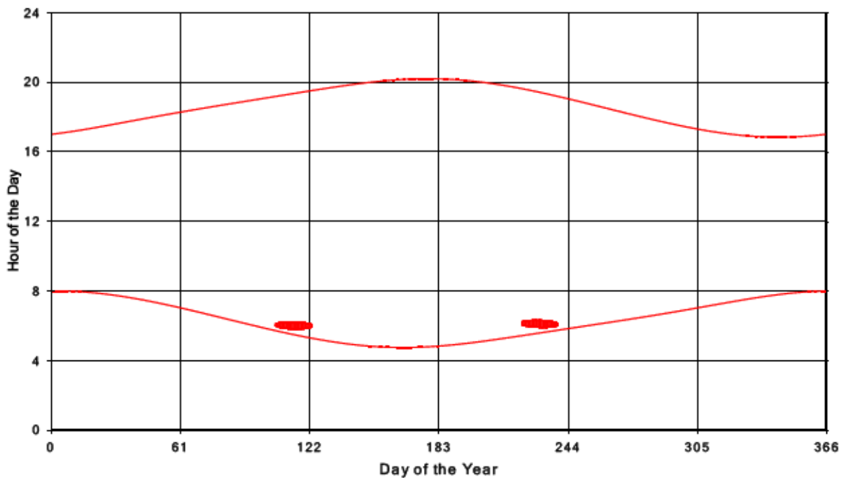
Bluewater Wind Energy Centre Shadow Times on Receptor 333, All Windows from All Turbine
