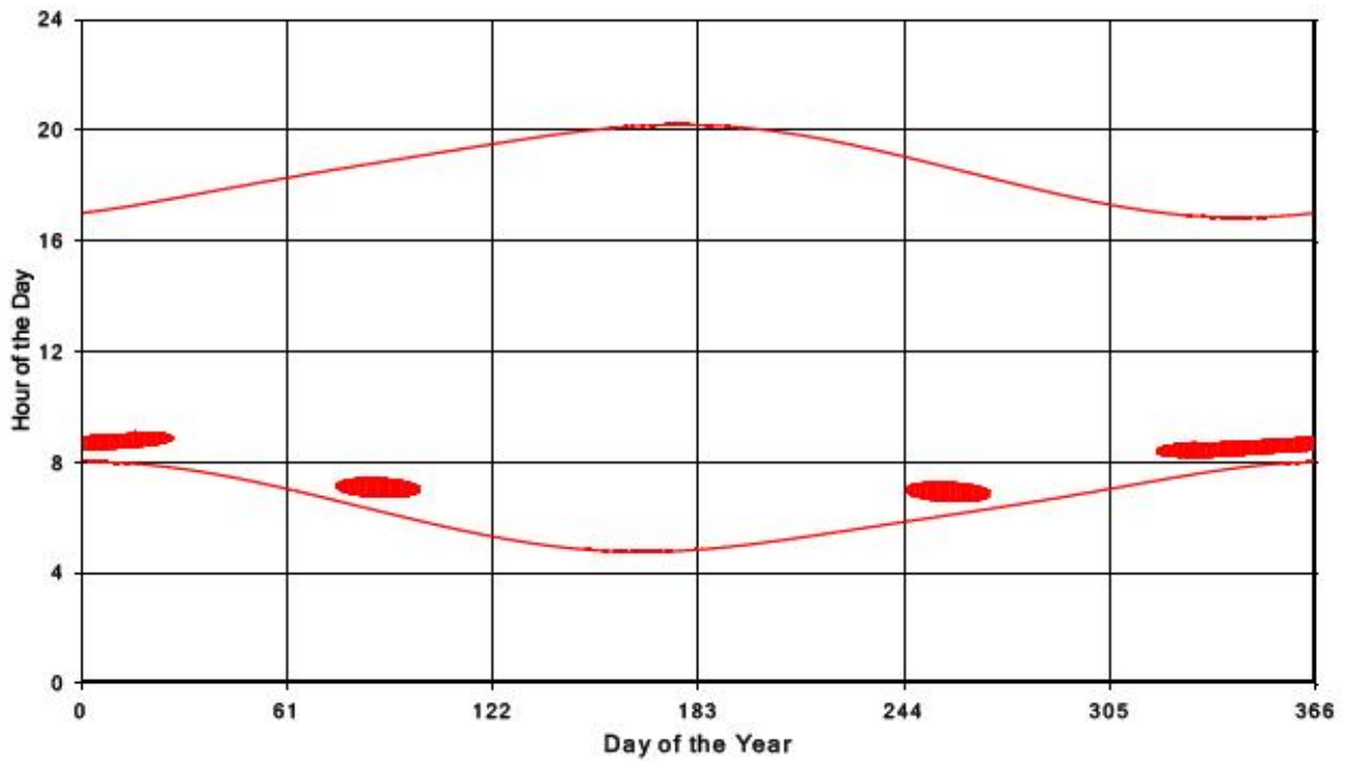
Bluewater Wind Energy Centre Shadow Times on Receptor 250, All Windows from All Turbine
