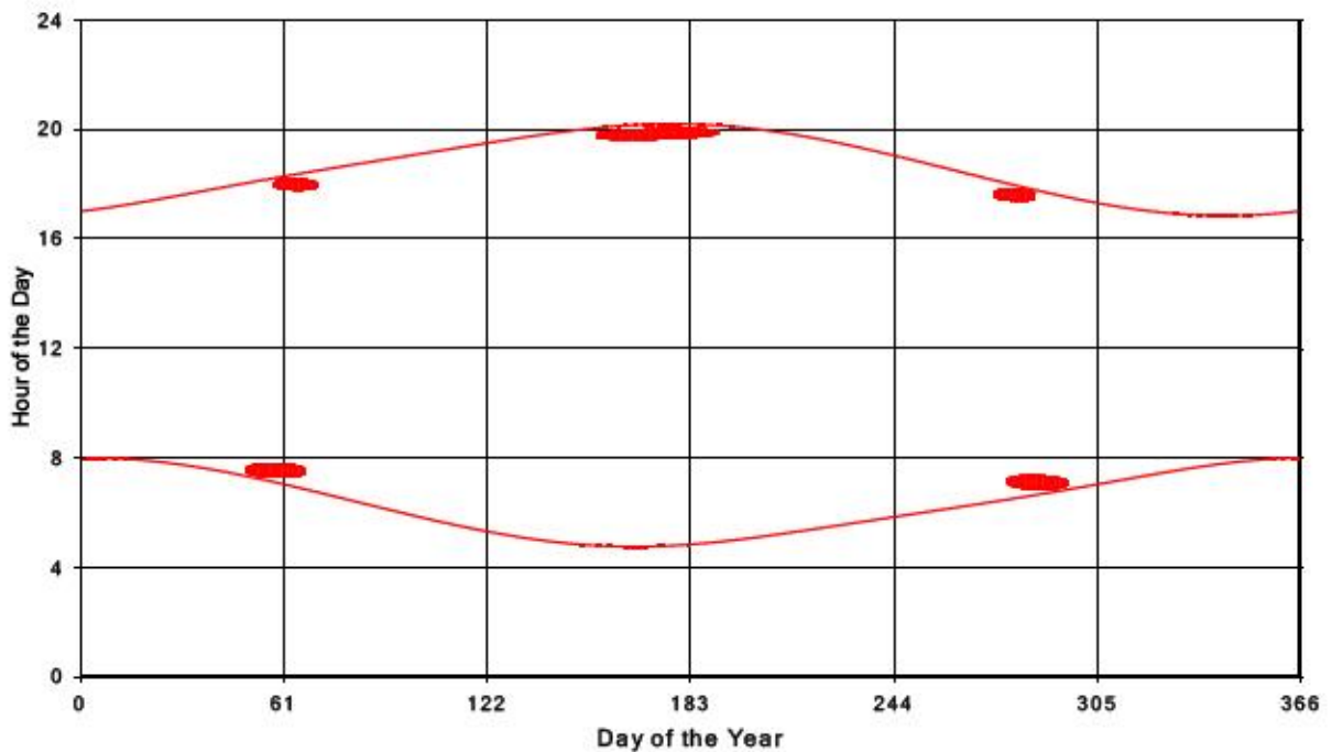
Bluewater Wind Energy Centre Shadow Times on Receptor 105, All Windows from All Turbine
