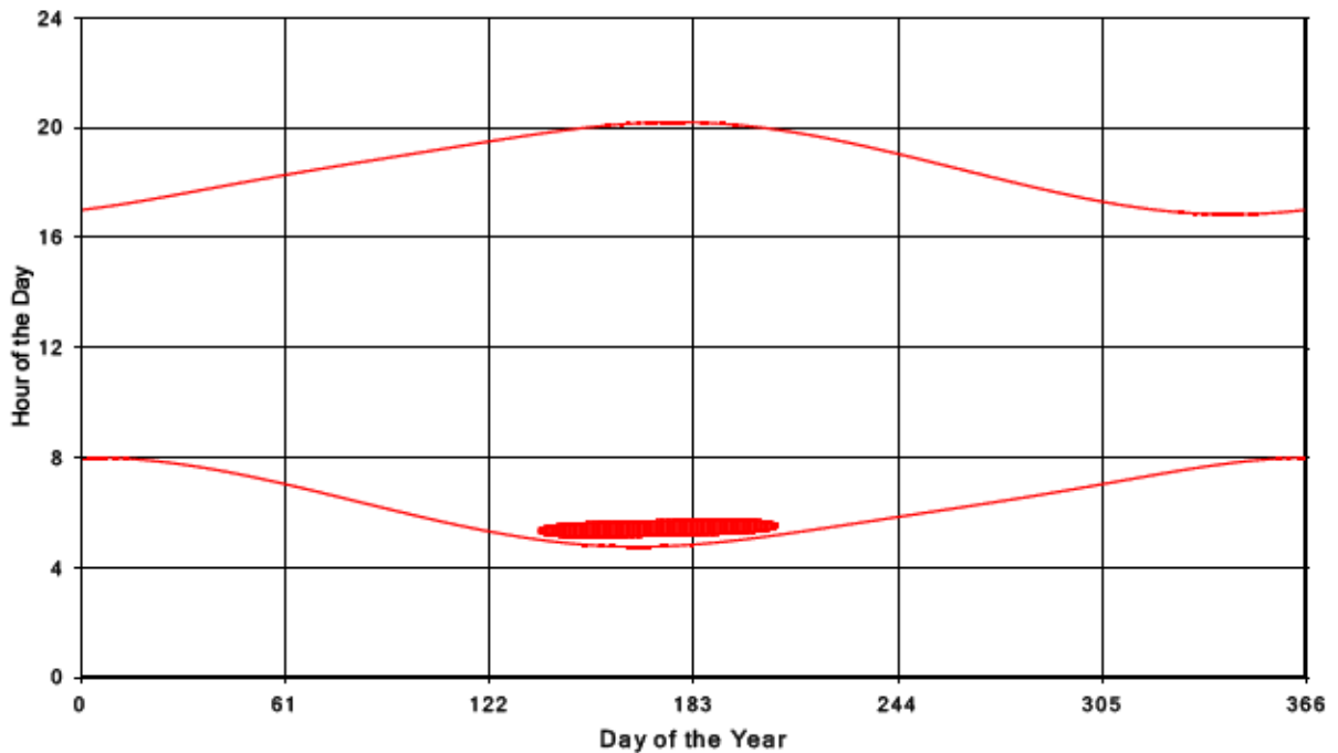
Bluewater Wind Energy Centre Shadow Times on Receptor 126, All Windows from All Turbine
