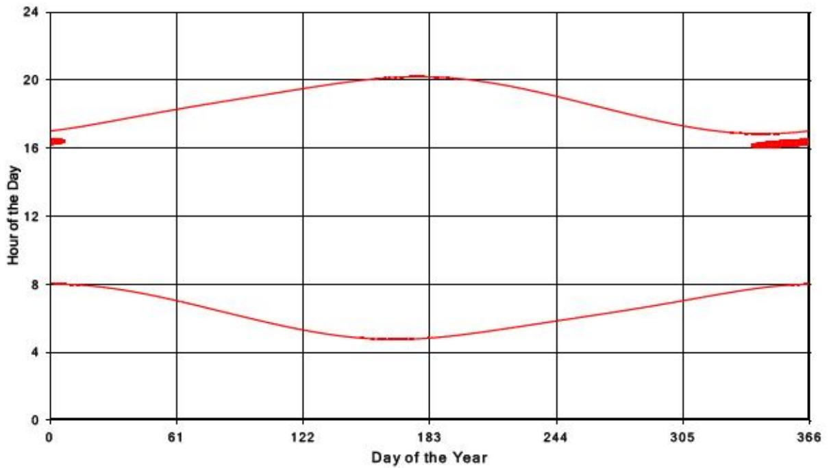
Bluewater Wind Energy Centre Shadow Times on Receptor 177, All Windows from All Turbine
