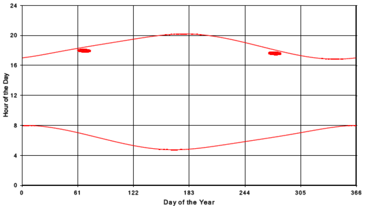
Bluewater Wind Energy Centre Shadow Times on Receptor 318, All Windows from All Turbine
