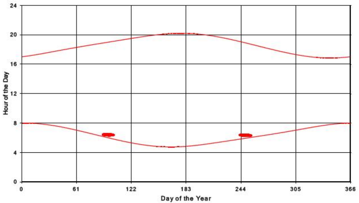
Bluewater Wind Energy Centre Shadow Times on Receptor 102, All Windows from All Turbine:
