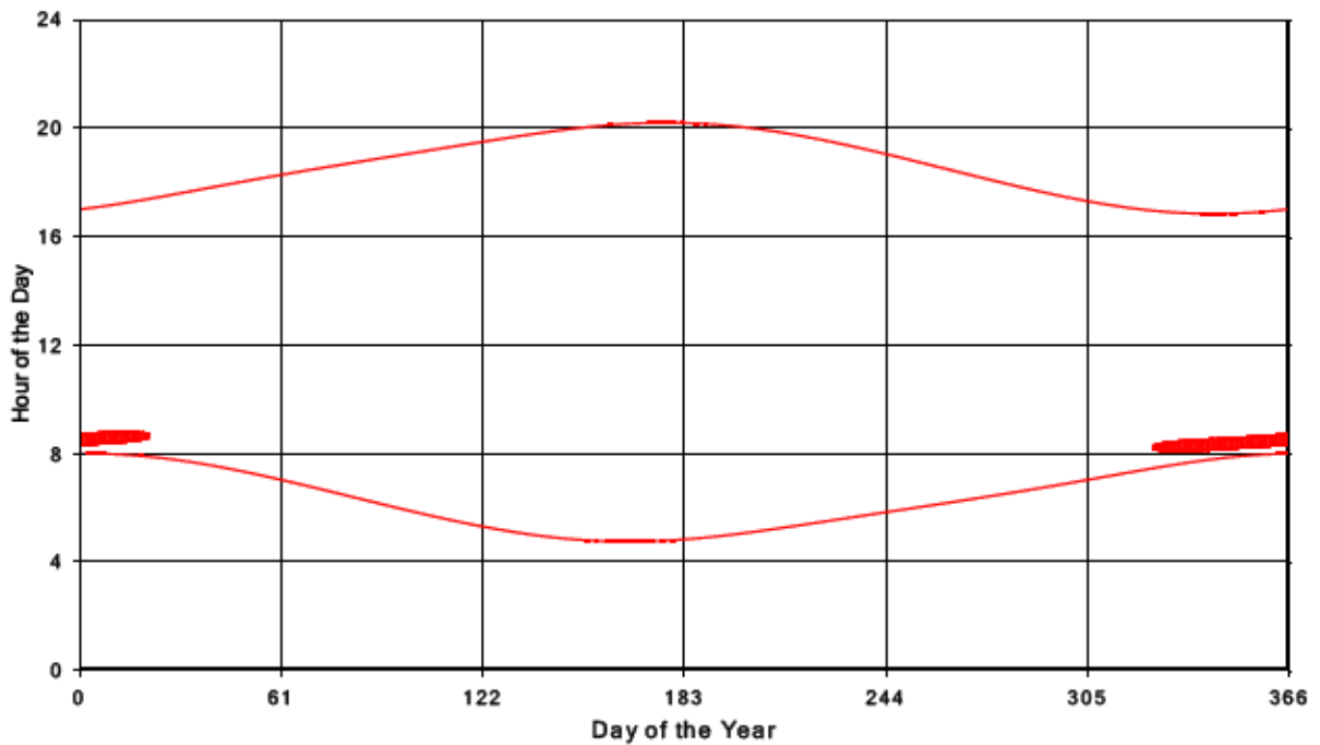
Bluewater Wind Energy Centre Shadow Times on Receptor 4, All Windows from All Turbine:
