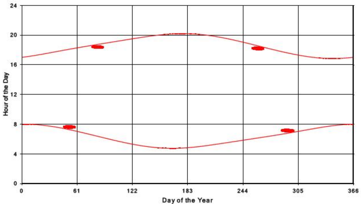
Bluewater Wind Energy Centre Shadow Times on Receptor 366, All Windows from All Turbine
