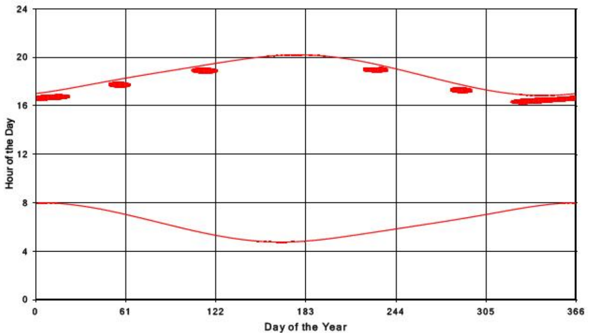
Bluewater Wind Energy Centre Shadow Times on Receptor 142, All Windows from All Turbine
