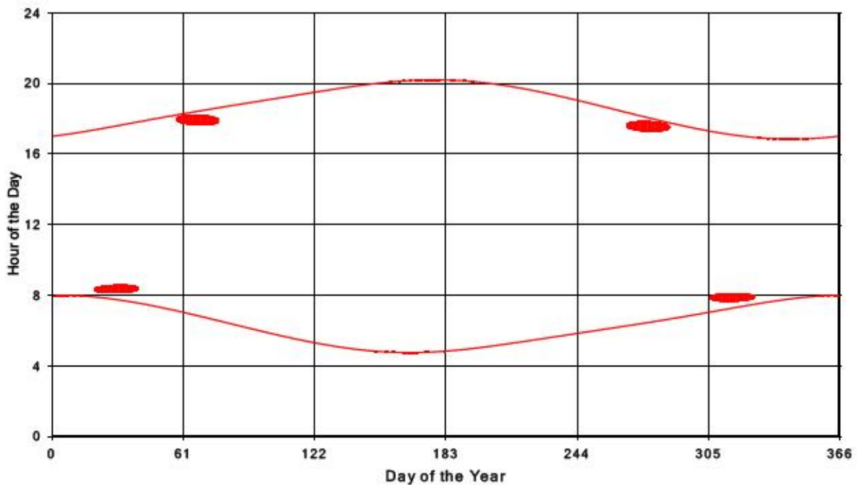
Bluewater Wind Energy Centre Shadow Times on Receptor 194, All Windows from All Turbine
