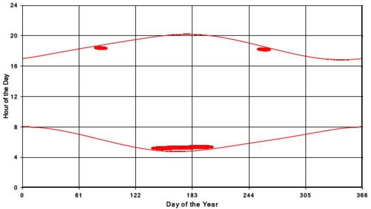
Bluewater Wind Energy Centre Shadow Times on Receptor 223, All Windows from All Turbine
