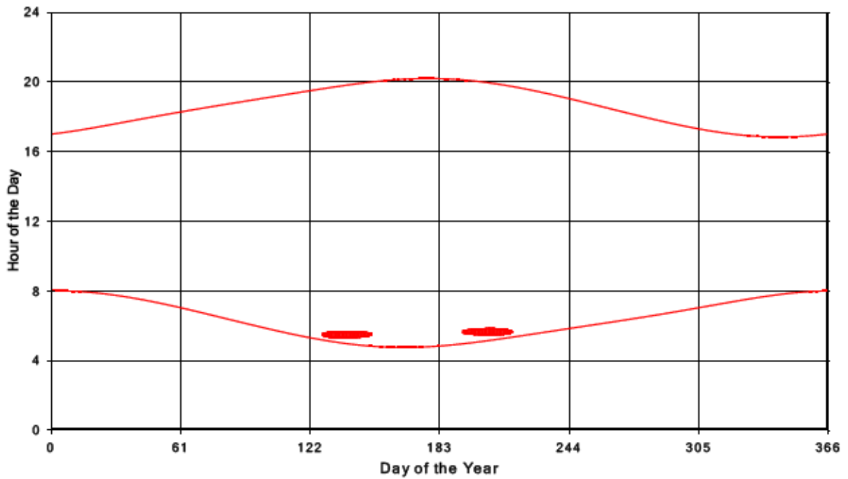
Bluewater Wind Energy Centre Shadow Times on Receptor 328, All Windows from All Turbine
