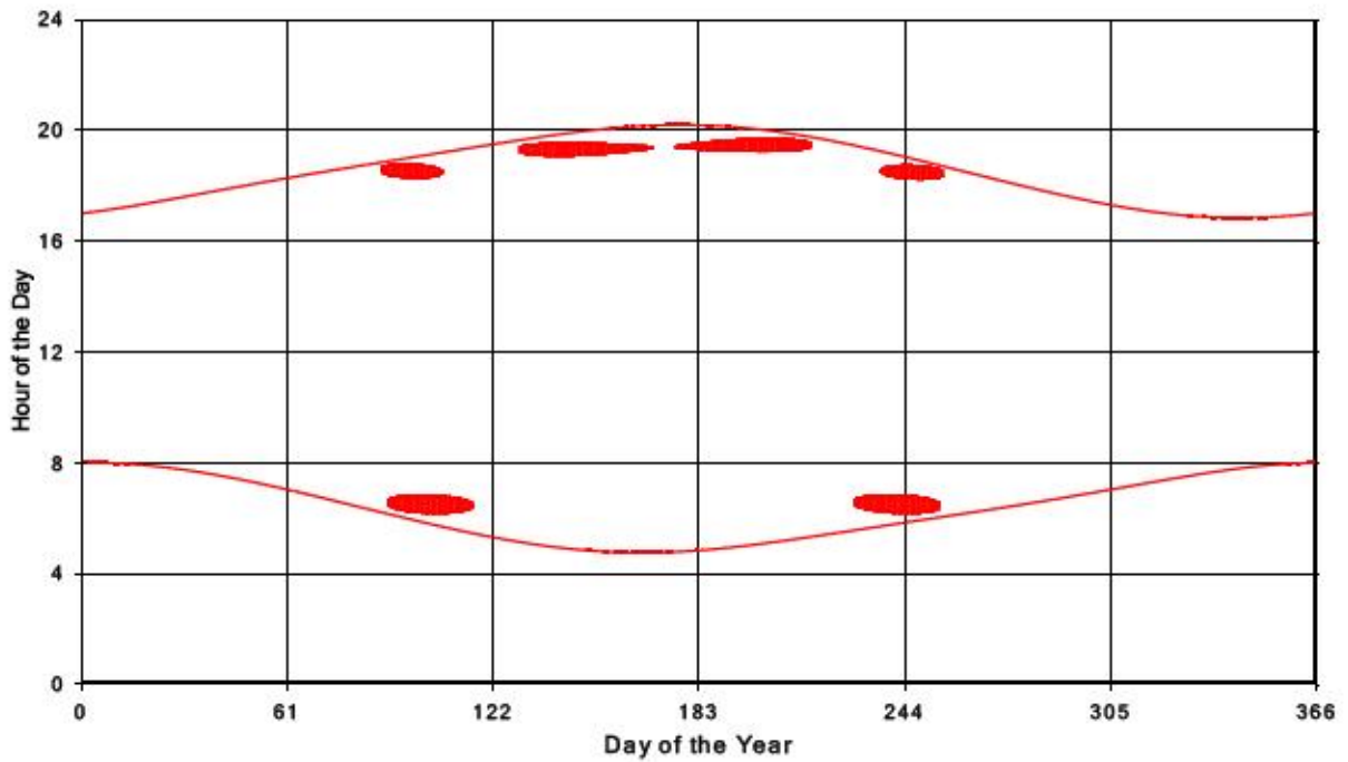
Bluewater Wind Energy Centre Shadow Times on Receptor 254, All Windows from All Turbine
