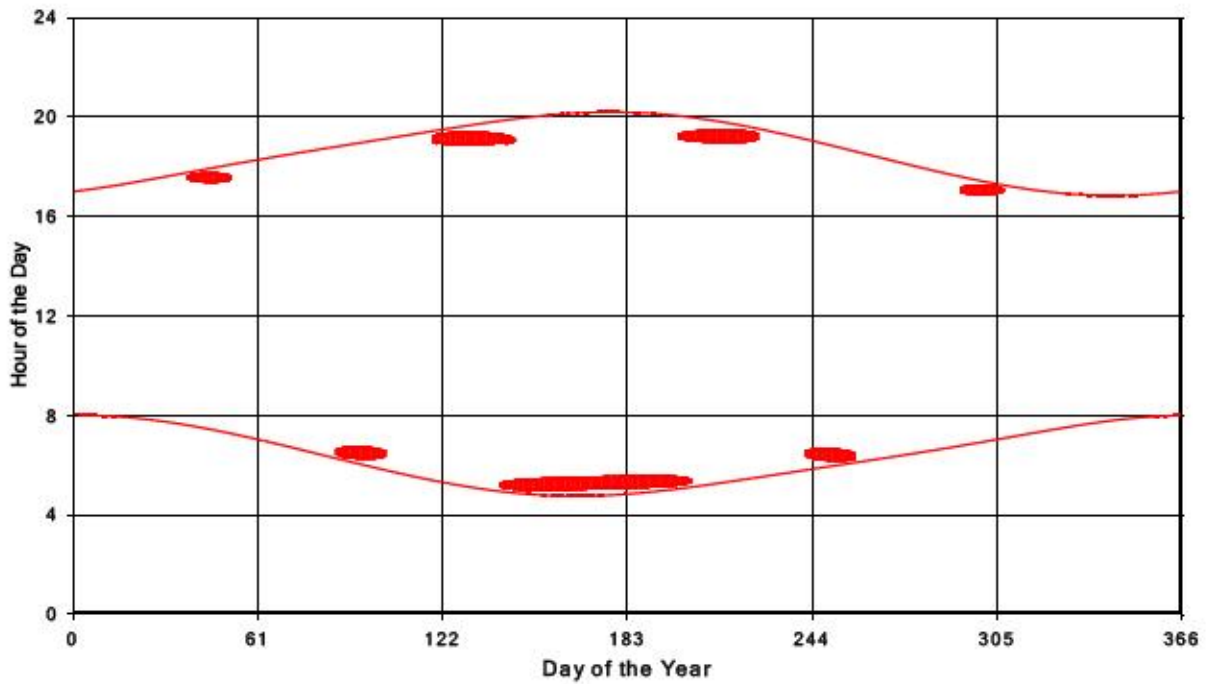
Bluewater Wind Energy Centre Shadow Times on Receptor 115, All Windows from All Turbine
