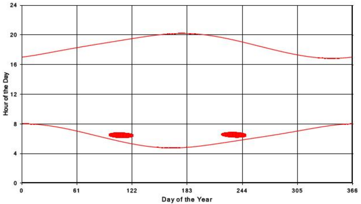
Bluewater Wind Energy Centre Shadow Times on Receptor 208, All Windows from All Turbine
