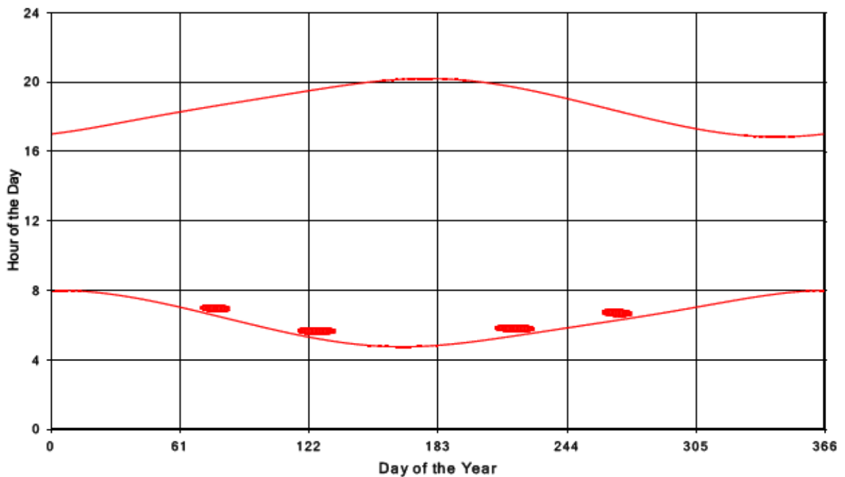
Bluewater Wind Energy Centre Shadow Times on Receptor 92, All Windows from All Turbine:
