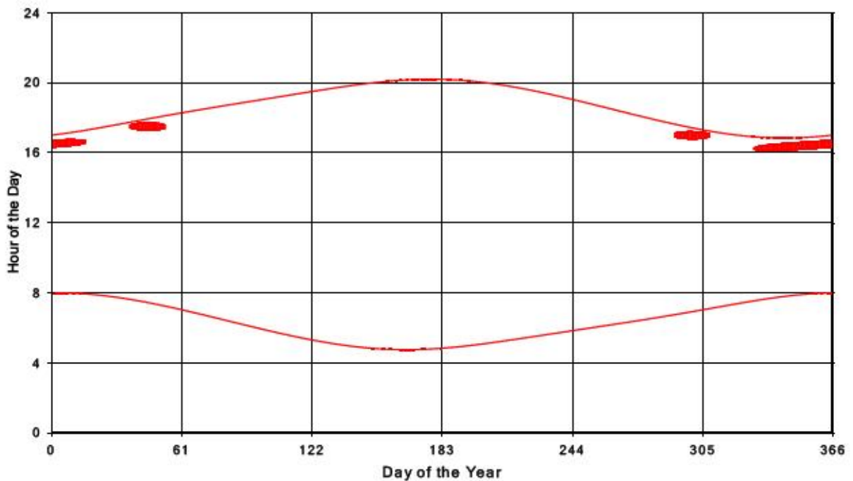
Bluewater Wind Energy Centre Shadow Times on Receptor 181, All Windows from All Turbine
