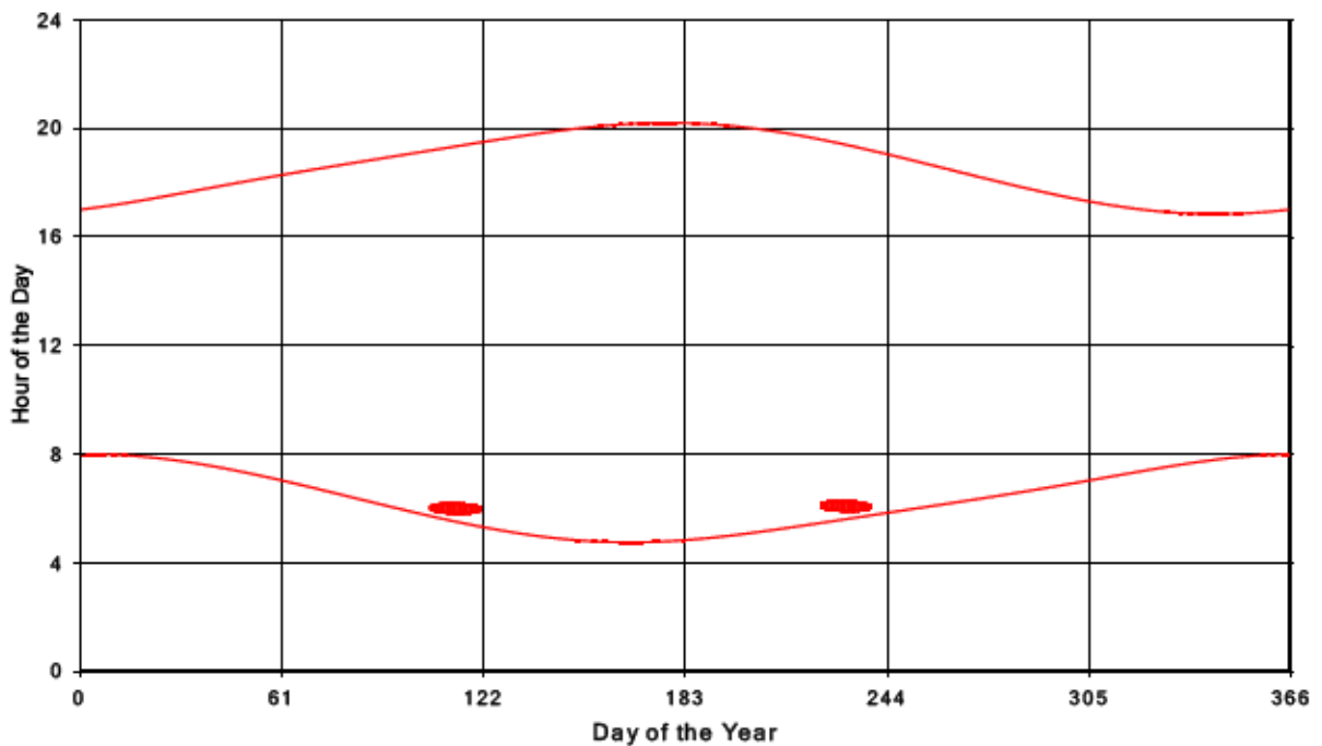
Bluewater Wind Energy Centre Shadow Times on Receptor 327, All Windows from All Turbine
