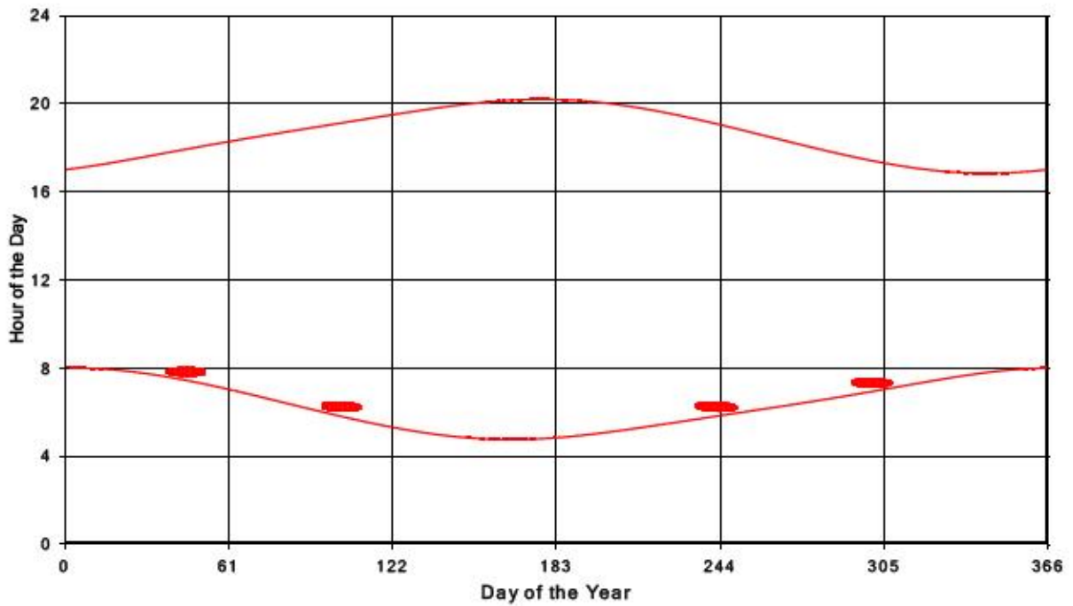
Bluewater Wind Energy Centre Shadow Times on Receptor 276, All Windows from All Turbine
