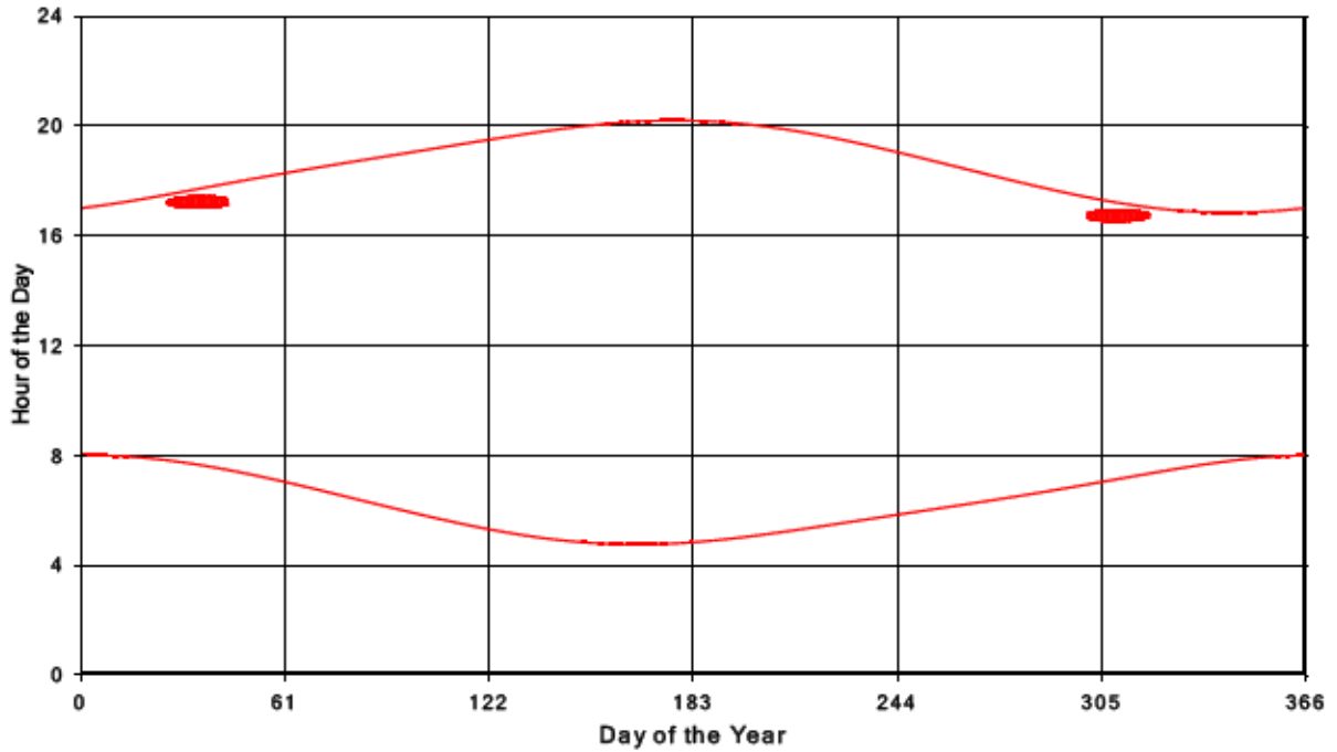
Bluewater Wind Energy Centre Shadow Times on Receptor 130, All Windows from All Turbine
