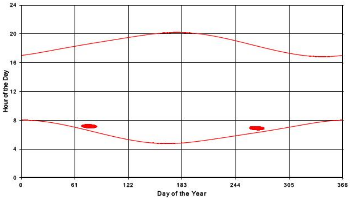
Bluewater Wind Energy Centre Shadow Times on Receptor 193, All Windows from All Turbine
