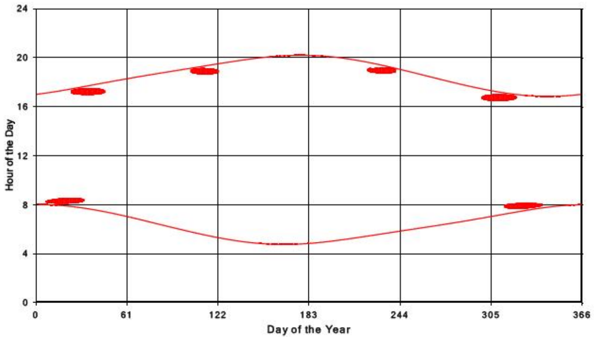
Bluewater Wind Energy Centre Shadow Times on Receptor 211, All Windows from All Turbine
