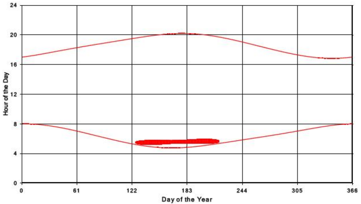
Bluewater Wind Energy Centre Shadow Times on Receptor 108, All Windows from All Turbine
