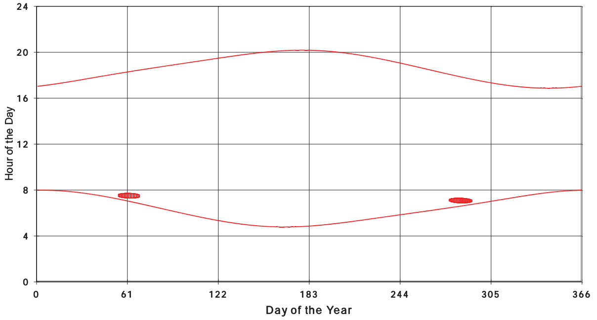
January 31 2013 Flicker with no barns shadow Times on House 3497, All Windows from All Turbine:
