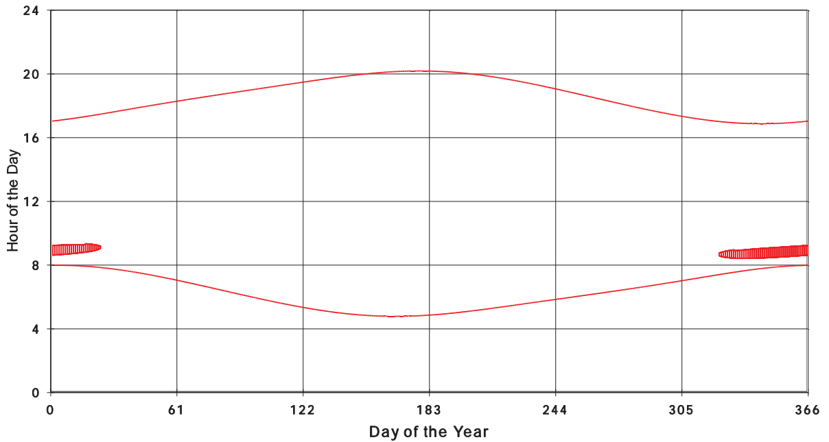
January 31 2013 Flicker with no barns shadow Times on House 3541, All Windows from All Turbine:
