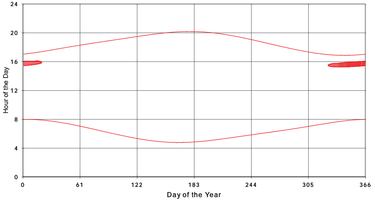
January 31 2013 Flicker with no barns Shadow Times on House 3306, All Windows from All Turbine:
