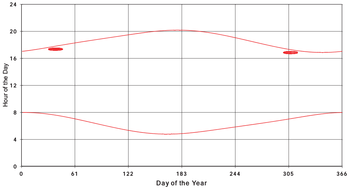
January 31 2013 Flicker with no barns Shadow Times on House 3524, All Windows from All Turbine:
