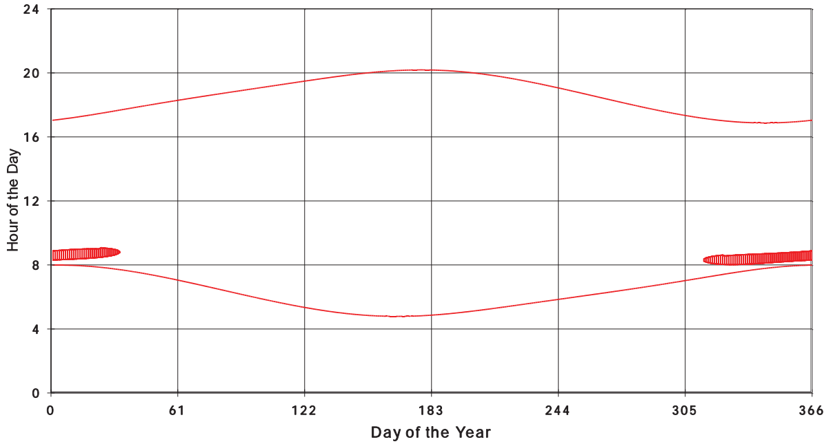
January 31 2013 Flicker with no barns Shadow Times on House 3302, All Windows from All Turbine:
