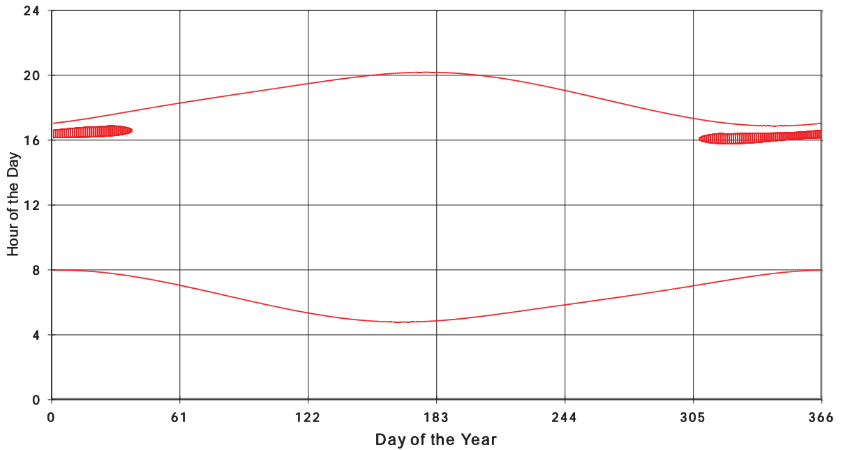
January 31 2013 Flicker with no barns Shadow Times on House 3303, All Windows from All Turbine:
