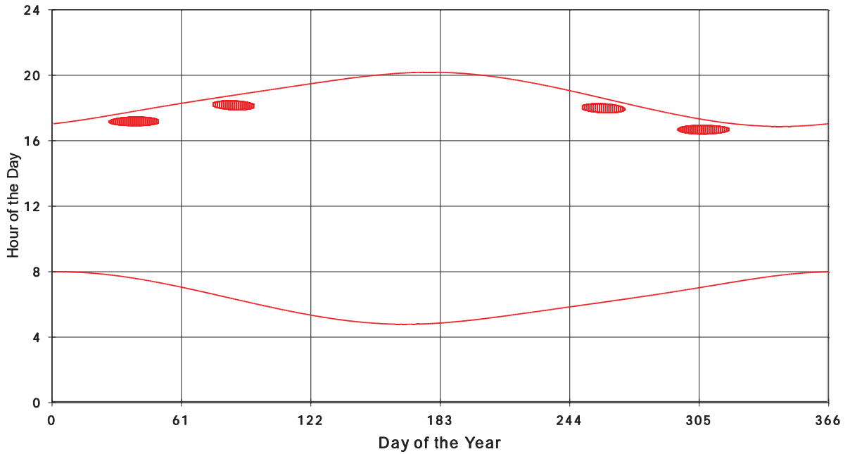
January 31 2013 Flicker with no barns Shadow Times on House 2631, All Windows from All Turbine:
