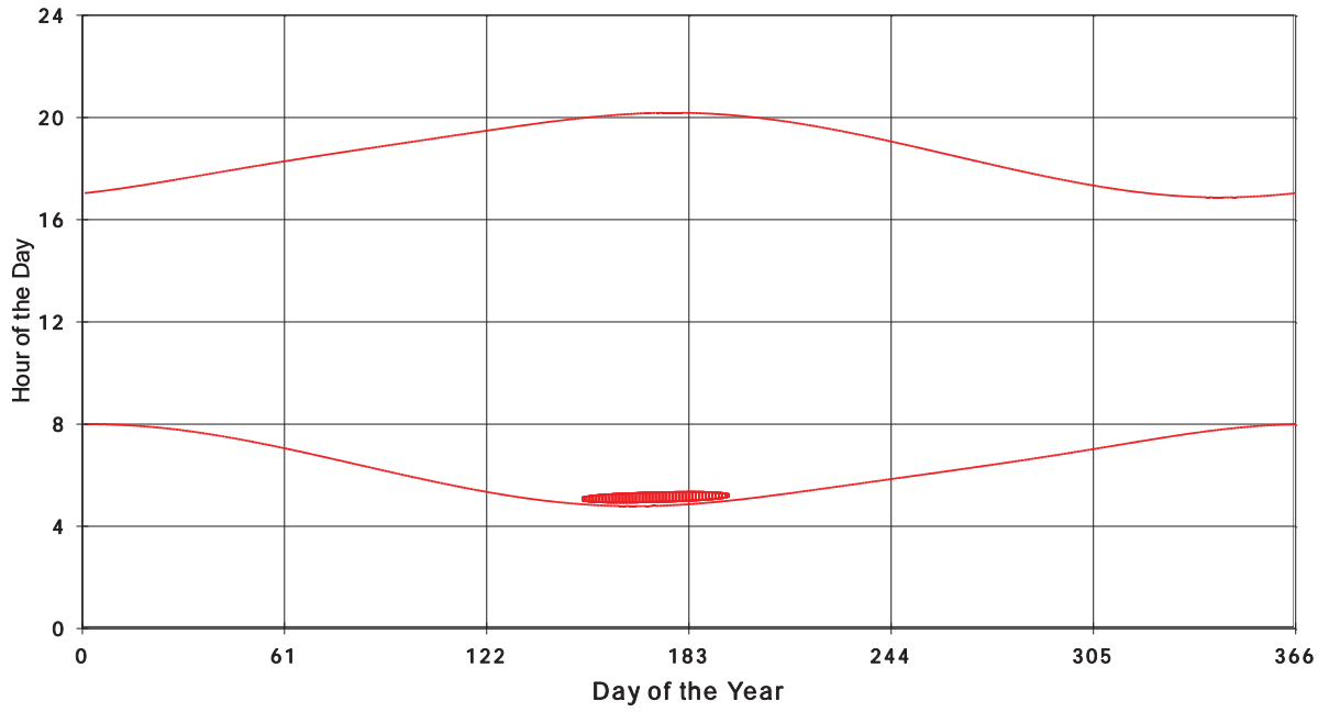
January 31 2013 Flicker with no barns Shadow Times on House 2636, All Windows from All Turbine:
