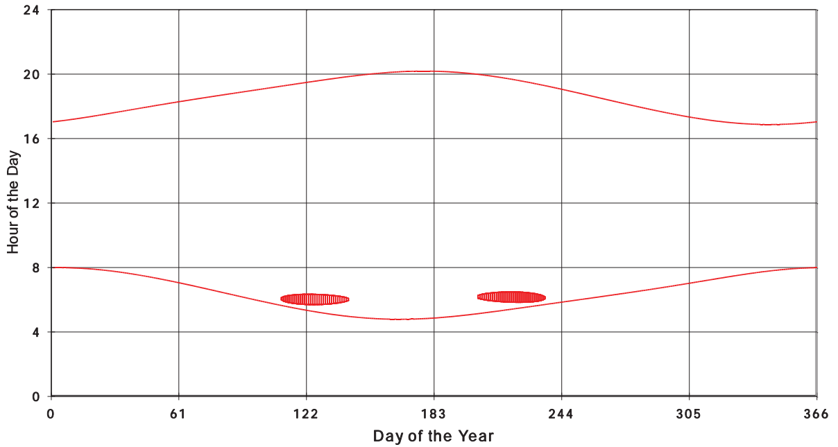
January 31 2013 Flicker with no barns shadow Times on House 2663, All Windows from All Turbine:
