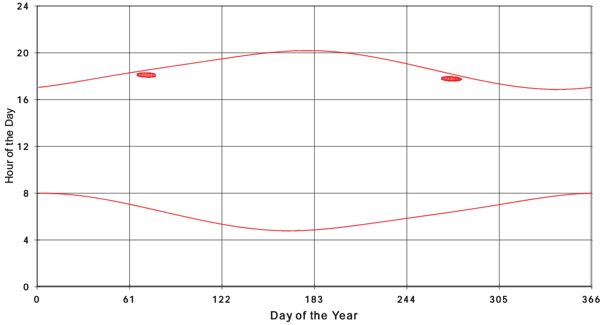
January 31 2013 Flicker with no barns shadow Times on House 2582, All Windows from All Turbine:
