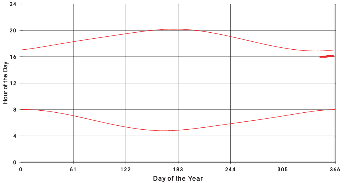
January 31 2013 Flicker with no barns shadow Times on House 2856, All Windows from All Turbine:
