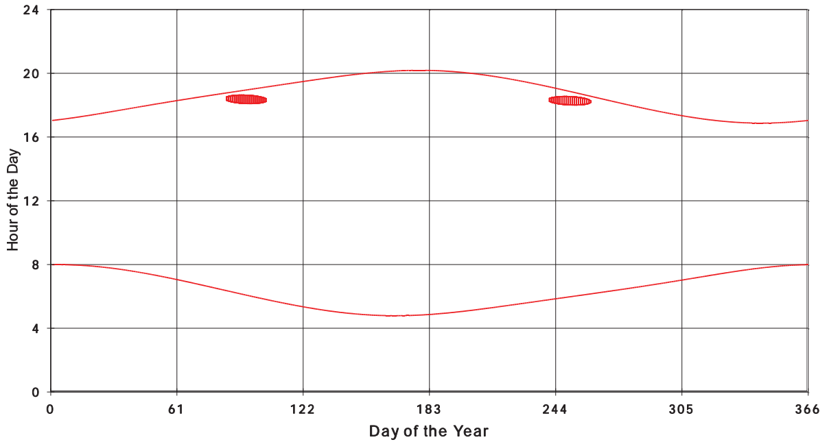
January 31 2013 Flicker with no barns Shadow Times on House 2591, All Windows from All Turbine:
