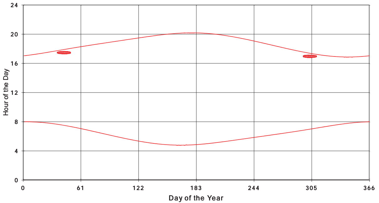
January 31 2013 Flicker with no barns shadow Times on House 2849, All Windows from All Turbine:
