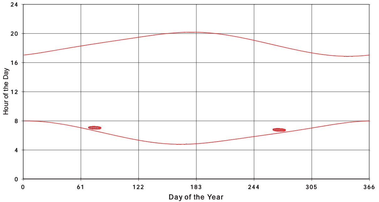
January 31 2013 Flicker with no barns shadow Times on House 2760, All Windows from All Turbine:
