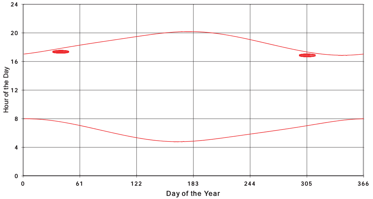
January 31 2013 Flicker with no barns shadow Times on House 2887, All Windows from All Turbine:
