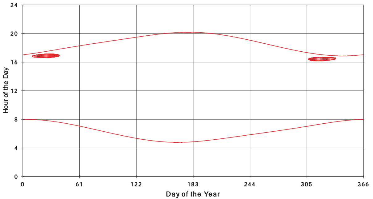
January 31 2013 Flicker with no barns Shadow Times on House 2816, All Windows from All Turbine:
