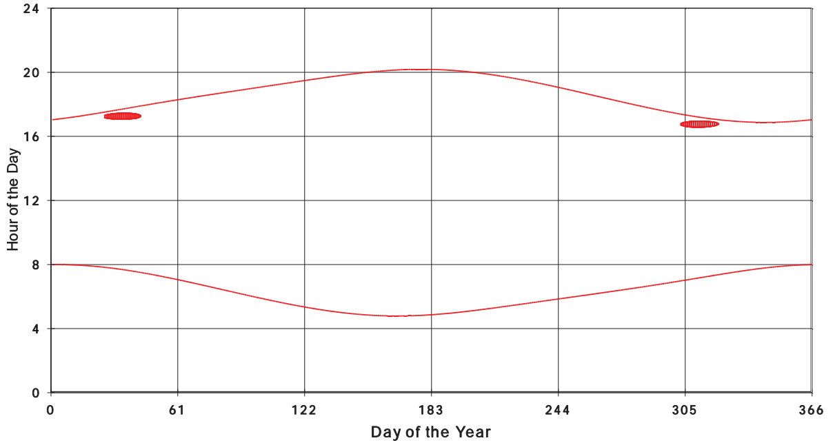
January 31 2013 Flicker with no barns shadow Times on House 2852, All Windows from All Turbine:
