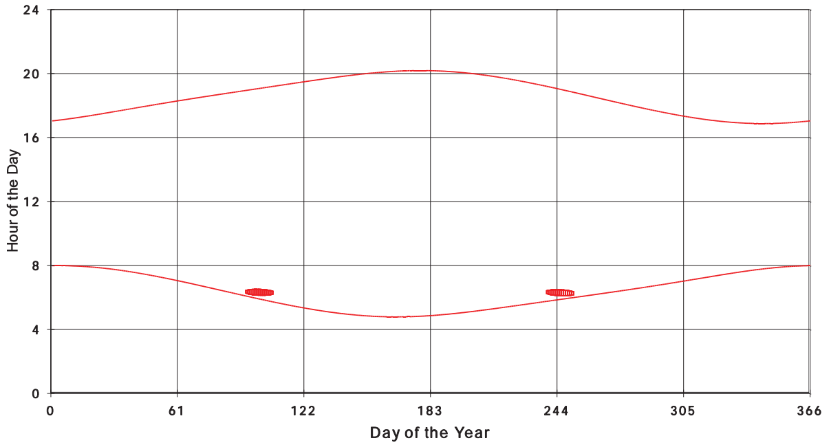
January 31 2013 Flicker with no barns hadow Times on House 2725, All Windows from All Turbine:
