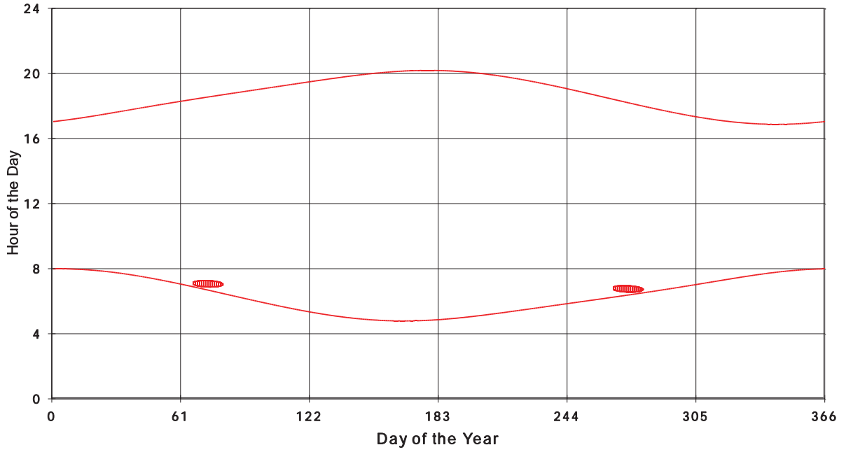
January 31 2013 Flicker with no barns shadow Times on House 2661, All Windows from All Turbine:
