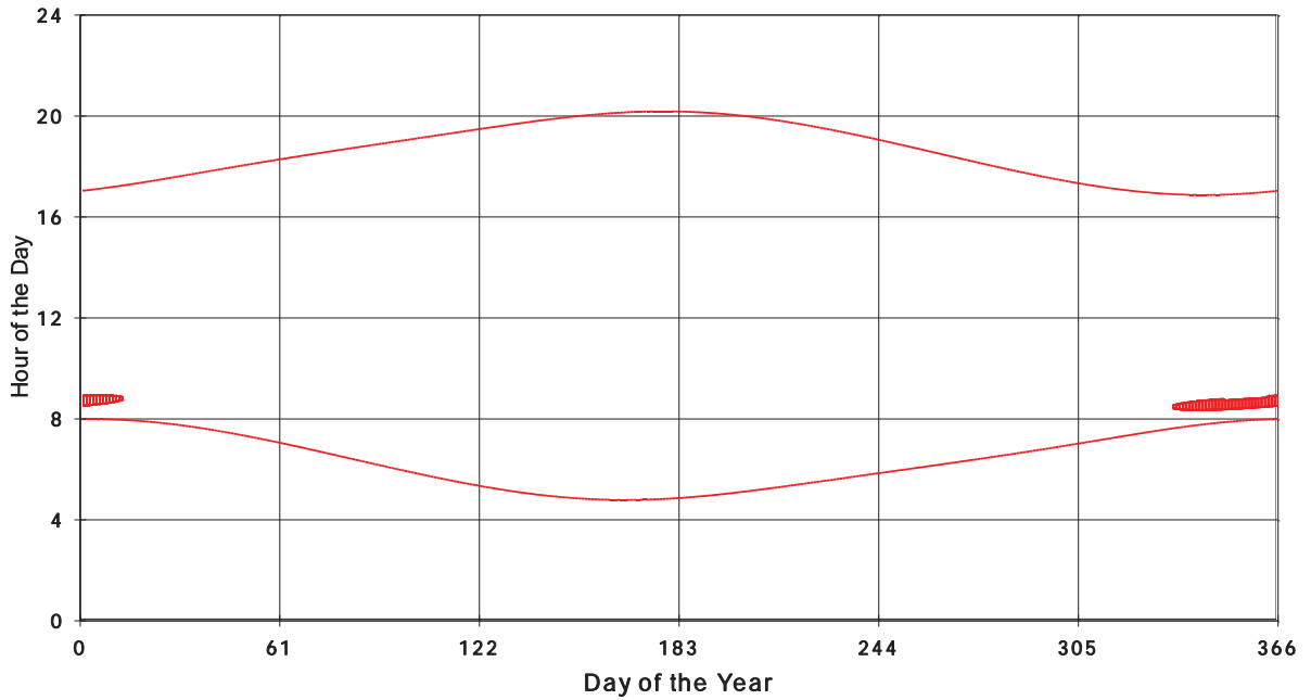
January 31 2013 Flicker with no barns shadow Times on House 2652, All Windows from All Turbine:
