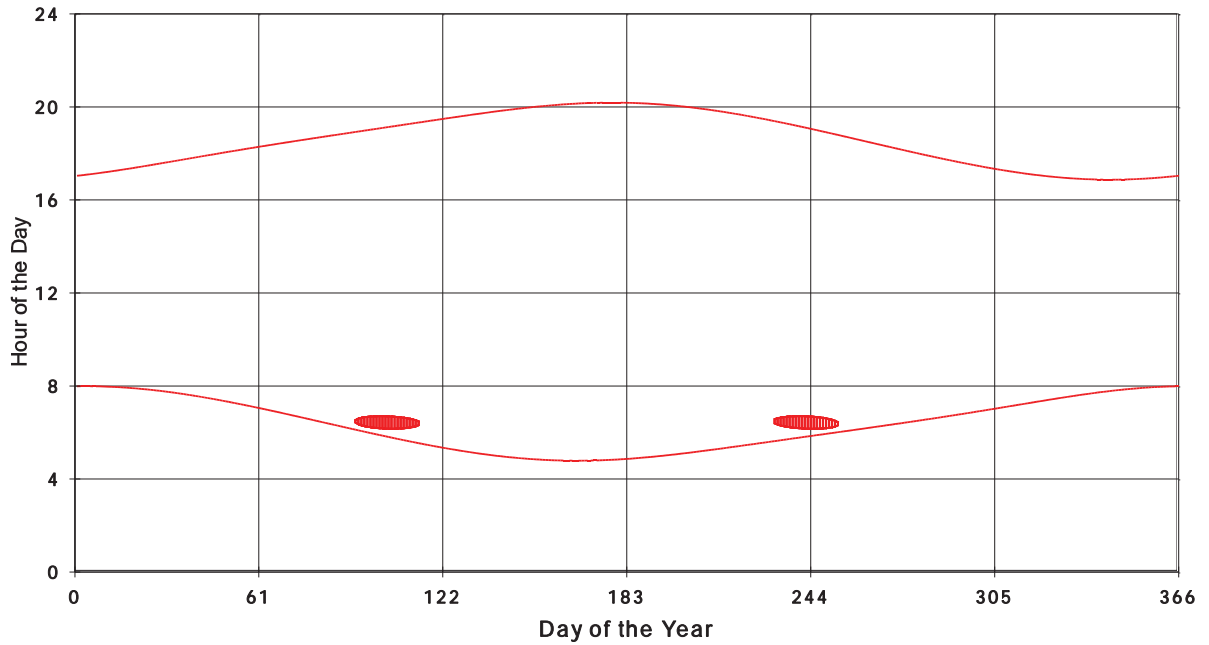
January 31 2013 Flicker with no barns shadow Times on House 2371, All Windows from All Turbine:
