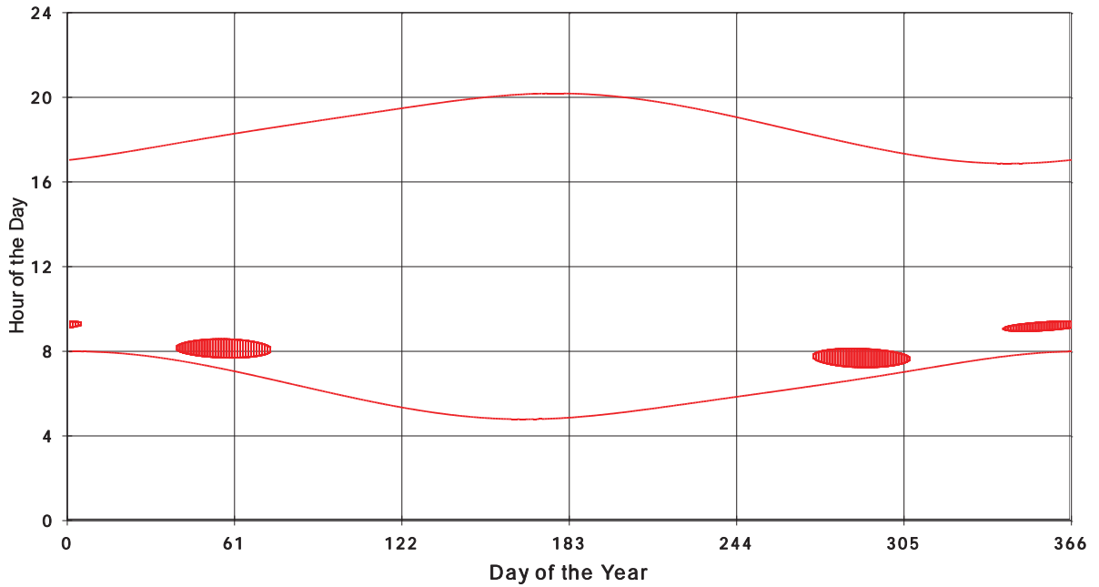
January 31 2013 Flicker with no barns shadow Times on House 2495, All Windows from All Turbine:
