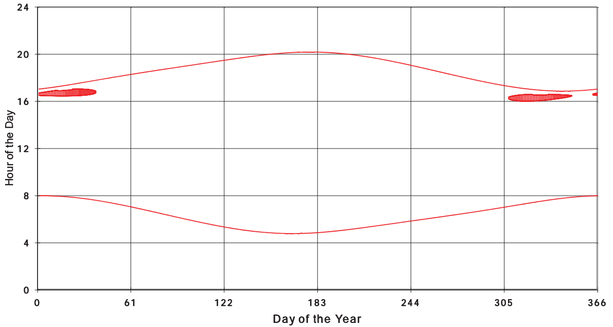
January 31 2013 Flicker with no barns Shadow Times on House 2525, All Windows from All Turbine:
