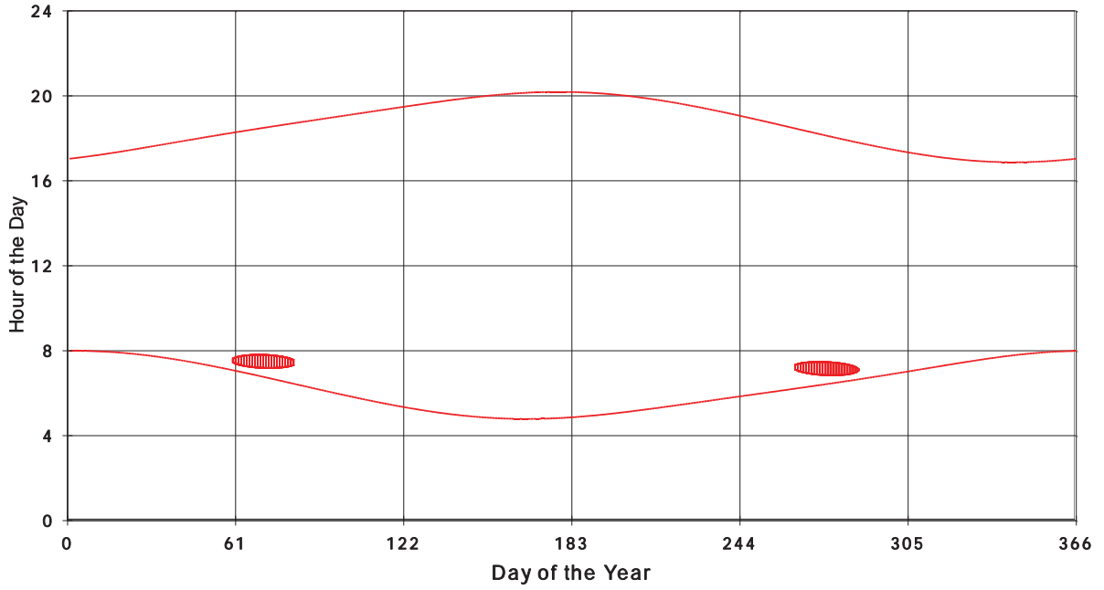
January 31 2013 Flicker with no barns shadow Times on House 2494, All Windows from All Turbine:
