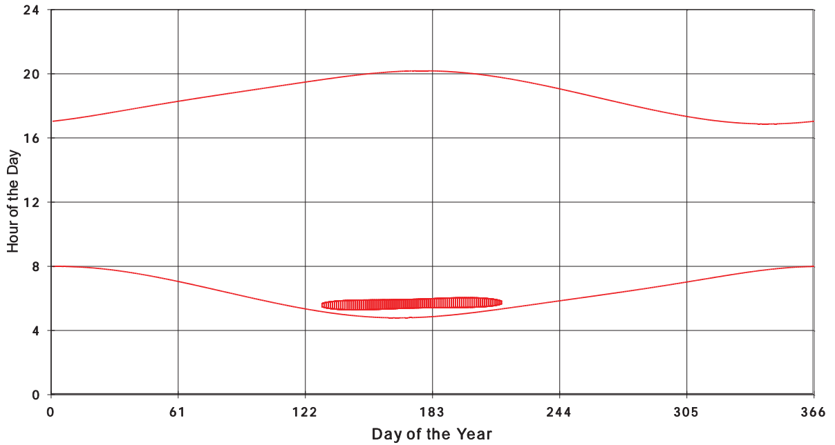
January 31 2013 Flicker with no barns Shadow Times on House 2532, All Windows from All Turbine:
