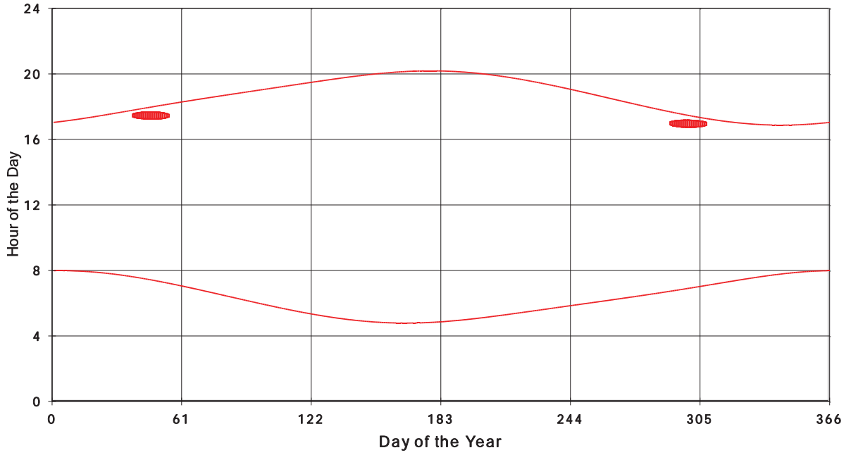
January 31 2013 Flicker with no barns Shadow Times on House 2513, All Windows from All Turbine:
