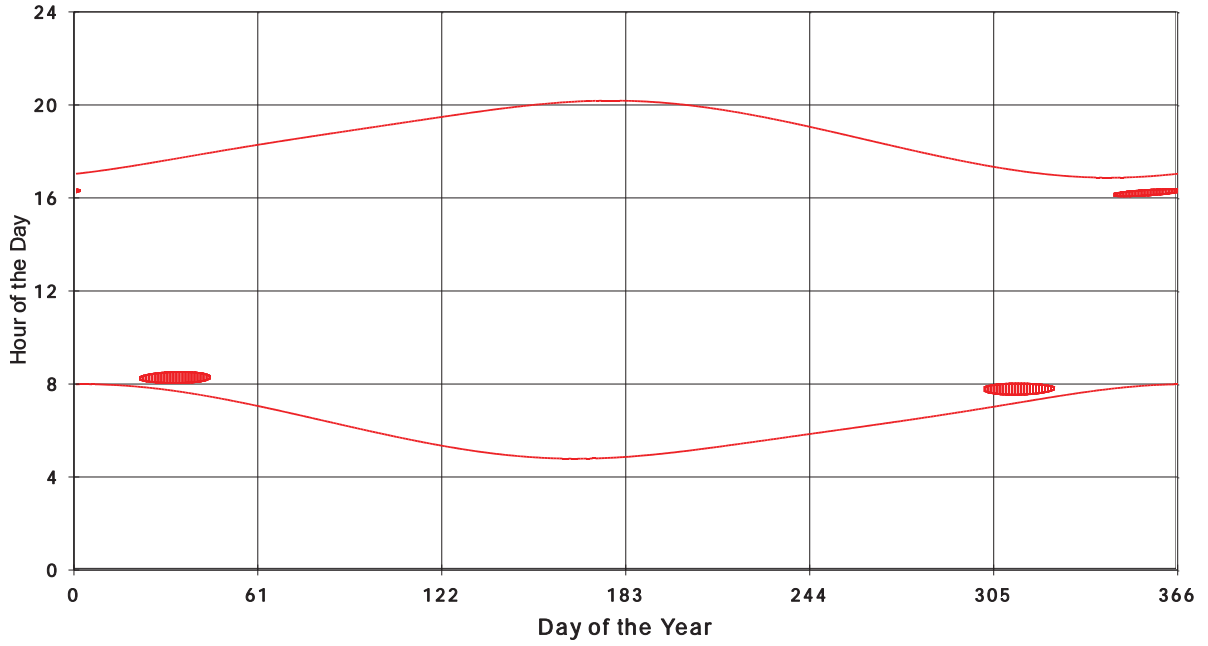
January 31 2013 Flicker with no barns shadow Times on House 2372, All Windows from All Turbine:
