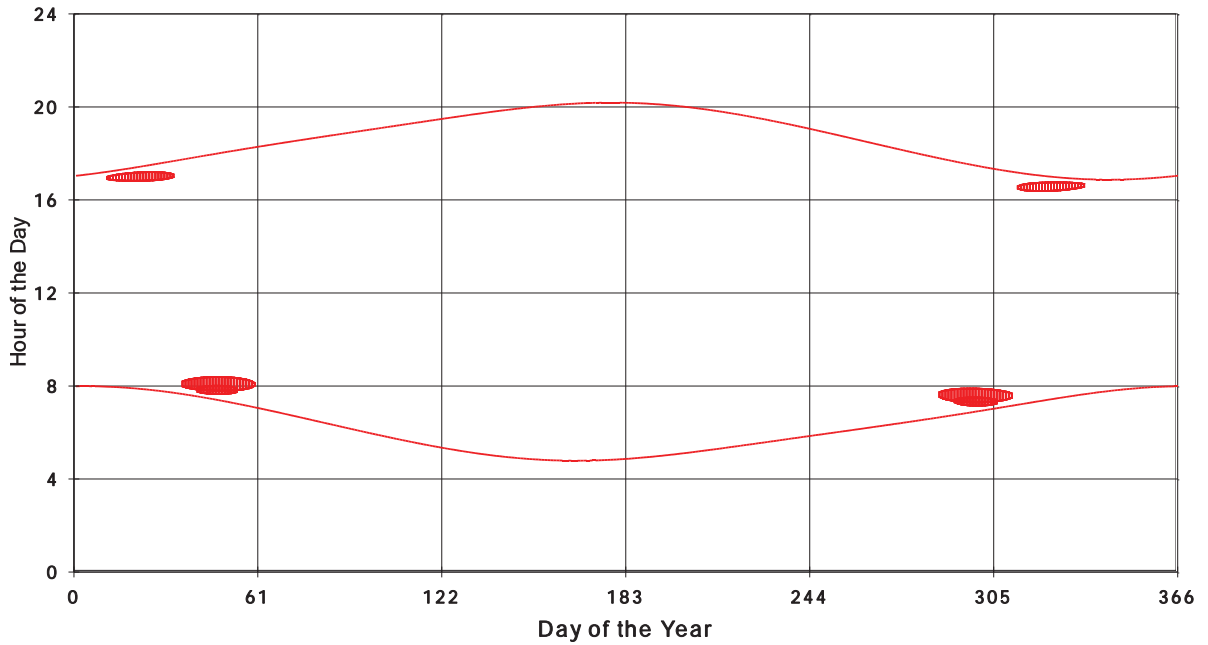
January 31 2013 Flicker with no barns shadow Times on House 2373, All Windows from All Turbine:
