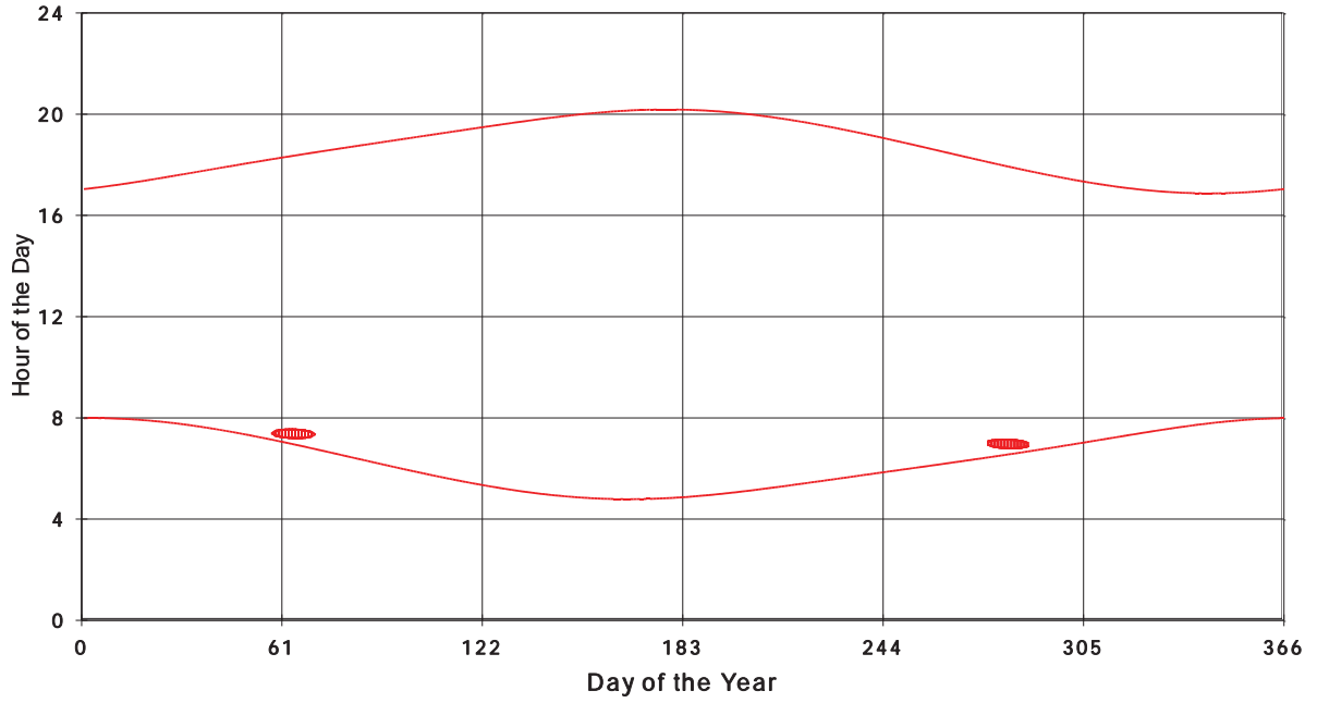
January 31 2013 Flicker with no barns shadow Times on House 2367, All Windows from All Turbine:
