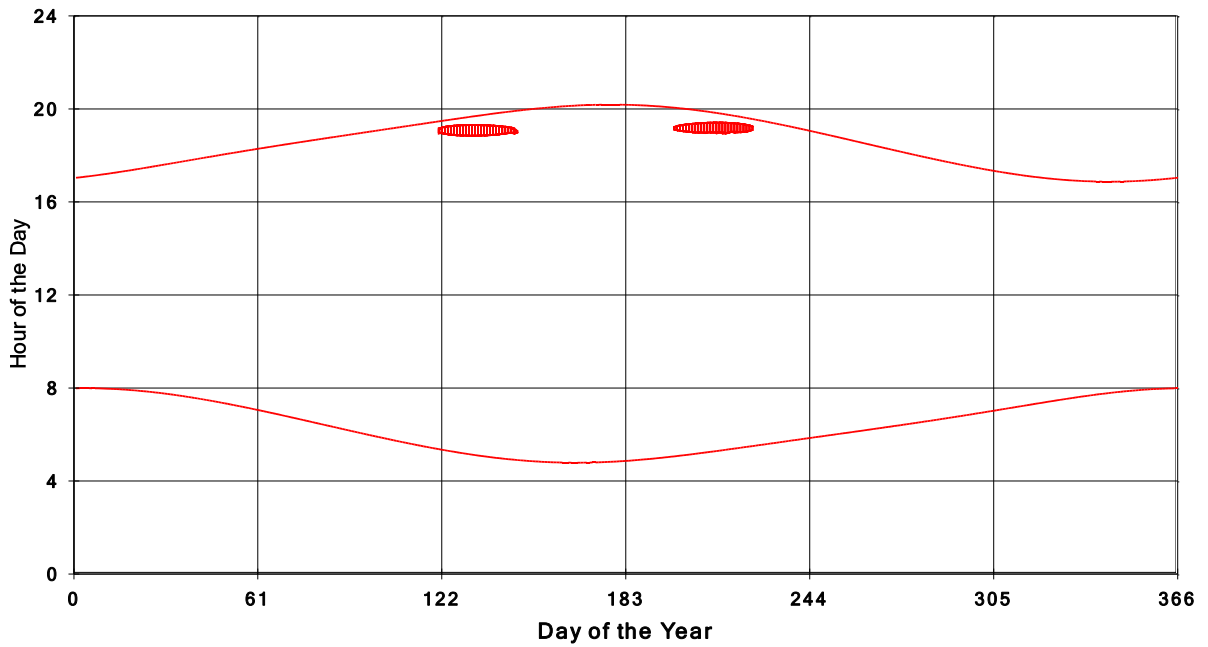
January 31 2013 Flicker with no barns shadow Times on House 2626, All Windows from All Turbine:
