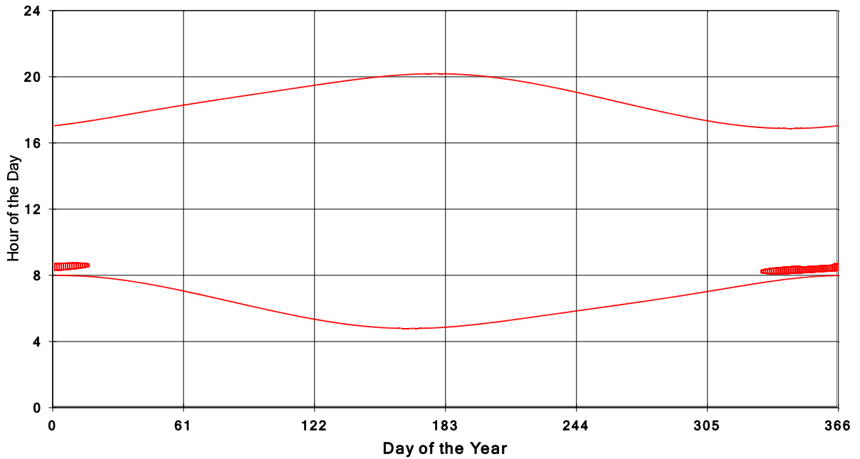
January 31 2013 Flicker with no barns shadow Times on House 3257, All Windows from All Turbine:
