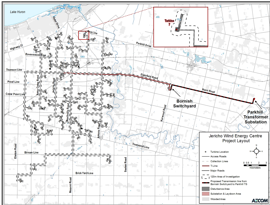
Project Layout
