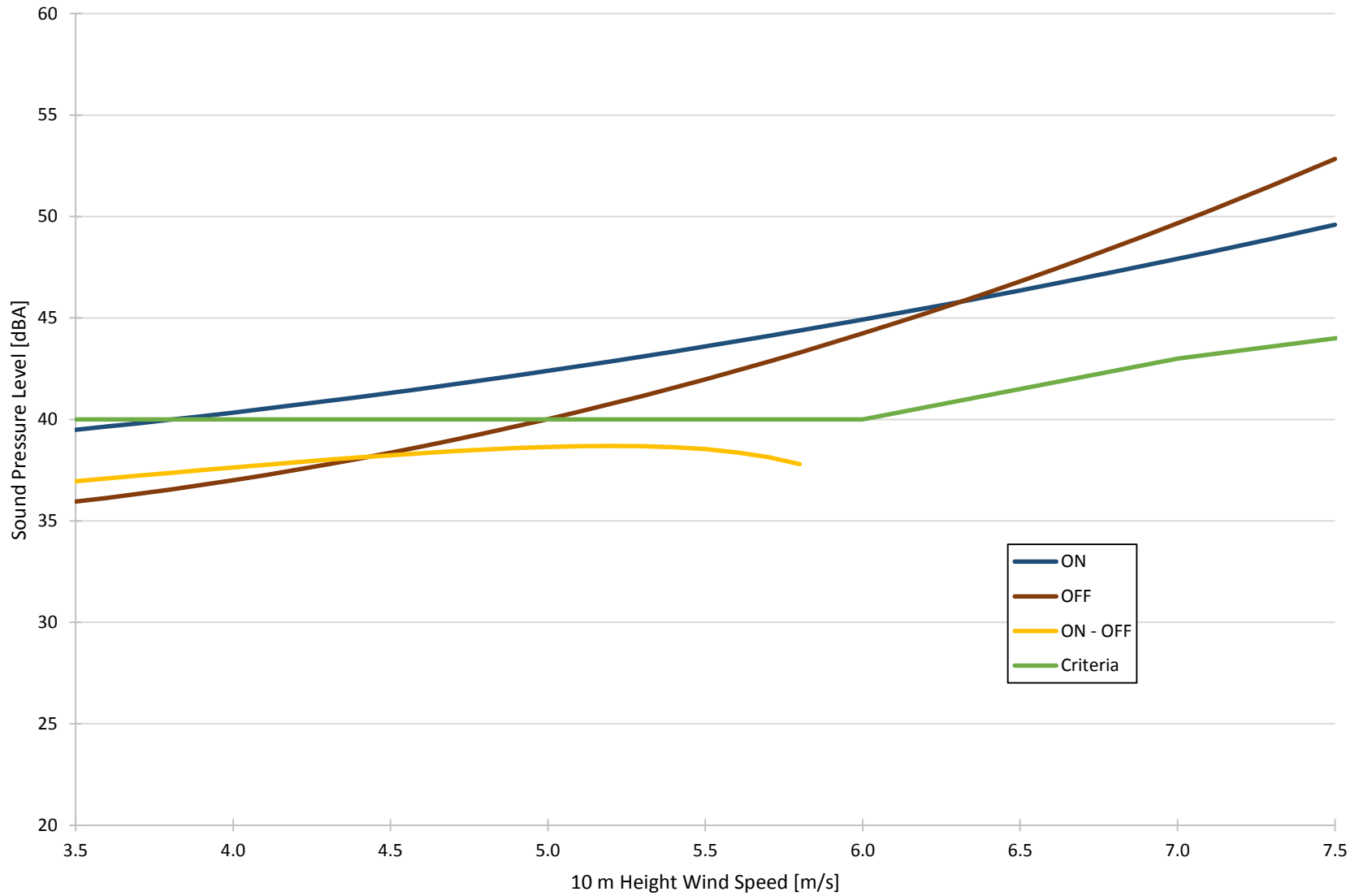
Figure 5b: Bluewater Wind Energy Centre Acoustic Audit Results Bronson Line, Receptor BLW517, September 4 to December 15, 2014
