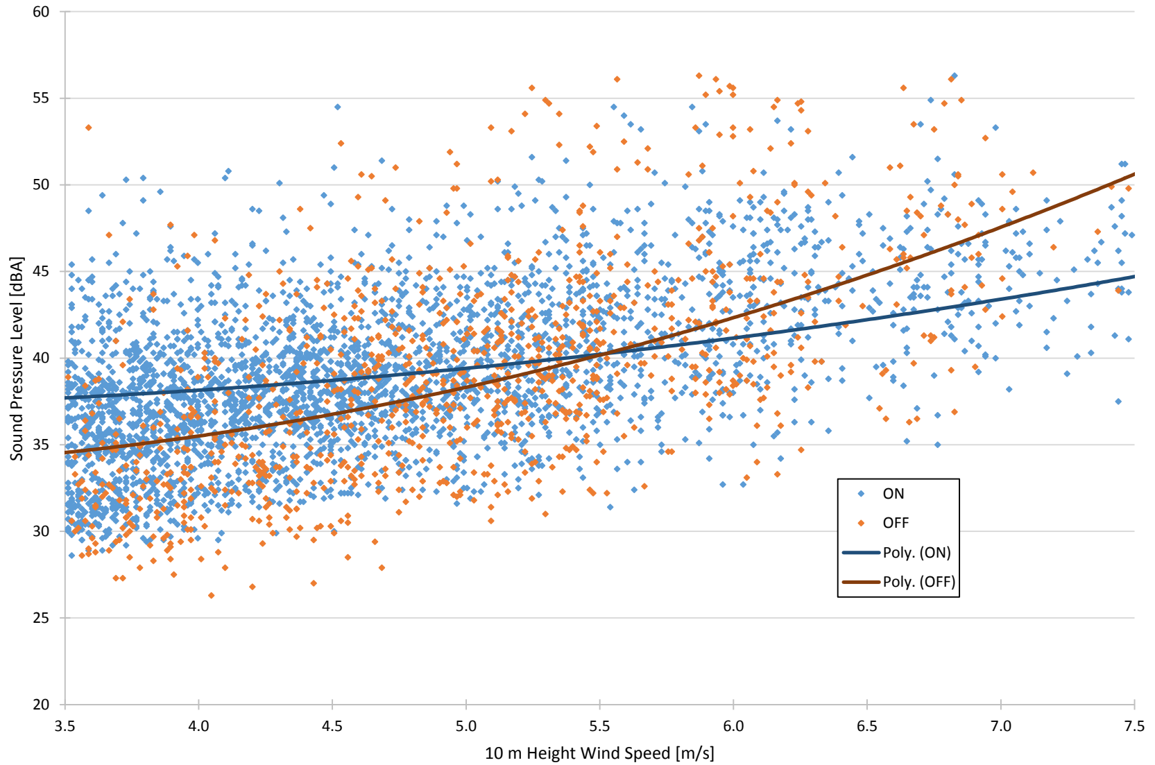
Figure 6a: Bluewater Wind Energy Centre Acoustic Audit Results Babylon Line, Receptor BLW906, September 4 to November 18, 2014
