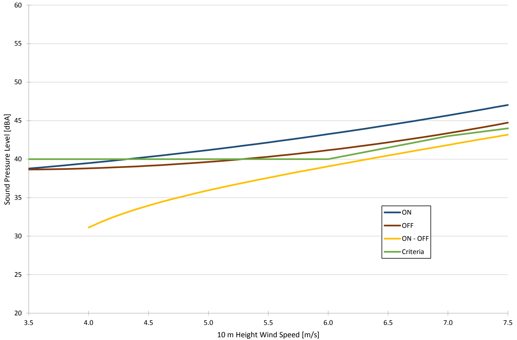
Figure 7b: Bluewater Wind Energy Centre Acoustic Audit Results Goshen Line, Receptor BLW780, September 23 to November 18, 2014
