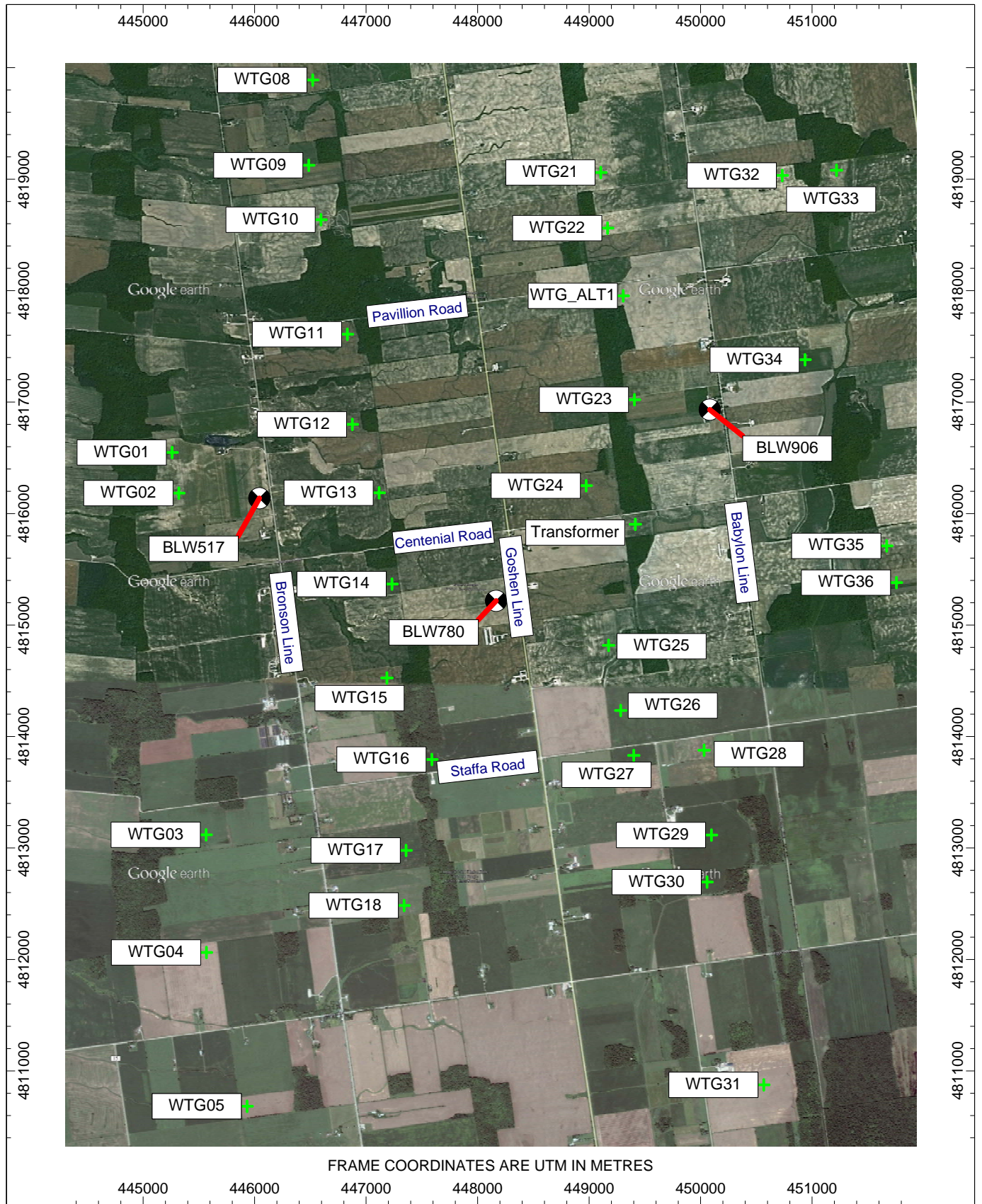
Figure 1: Wind Turbine and Sound Level Monitor Locations Bluewater Wind Energy Project, Bluewater, Ontario
