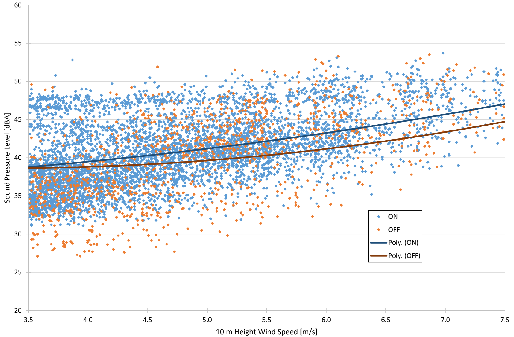
Figure 7a: Bluewater Wind Energy Centre Acoustic Audit Results Goshen Line, Receptor BLW780, September 23 to November 18, 2014
