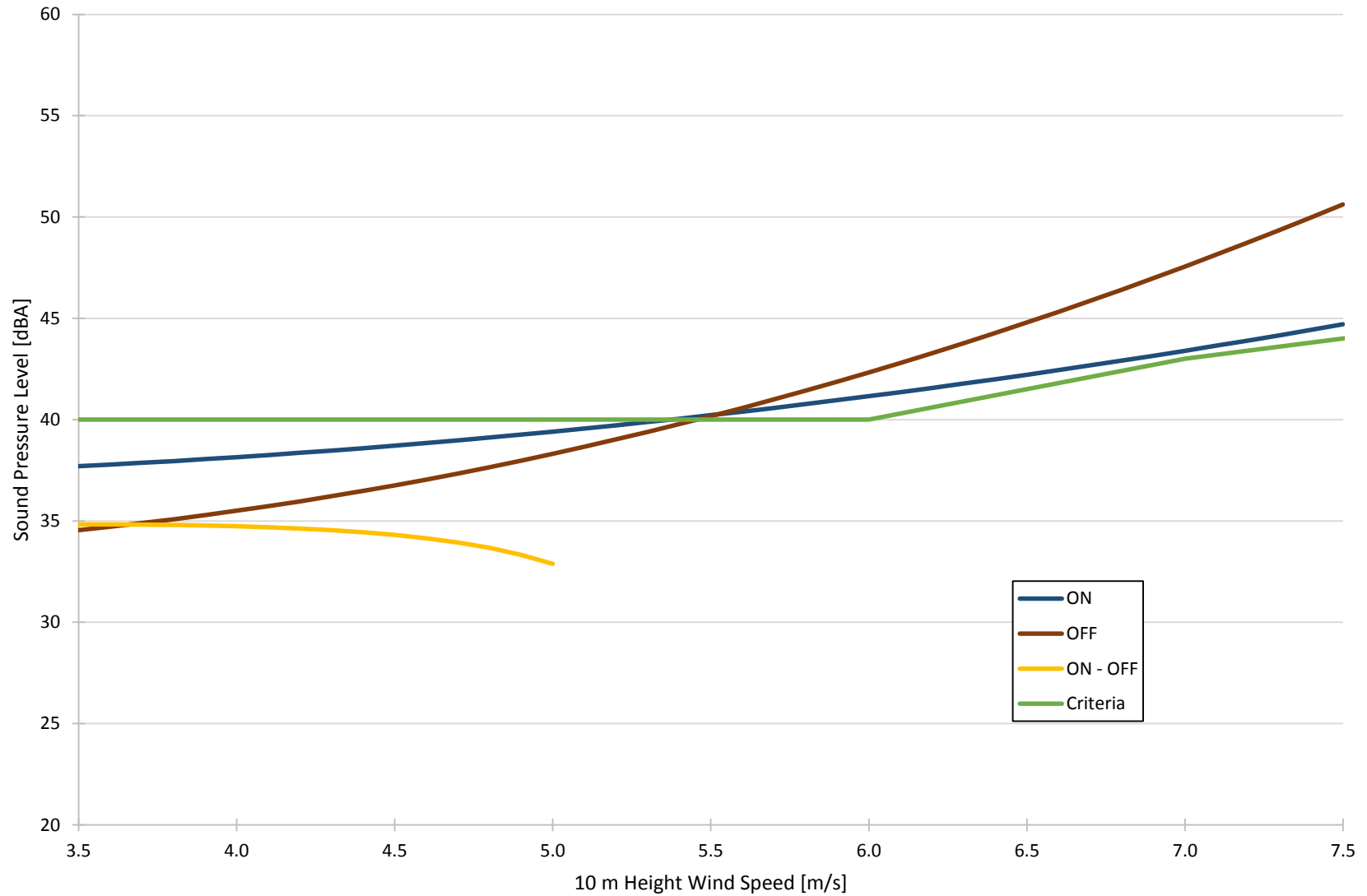
Figure 6b: Bluewater Wind Energy Centre Acoustic Audit Results Babylon Line, Receptor BLW906, September 4 to November 18, 2014
