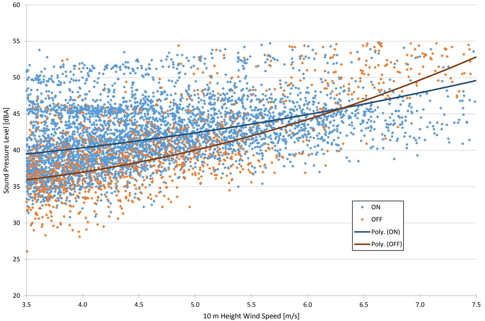
Figure 5a: Bluewater Wind Energy Centre Acoustic Audit Results Bronson Line, Receptor BLW517, September 4 to December 15, 2014
