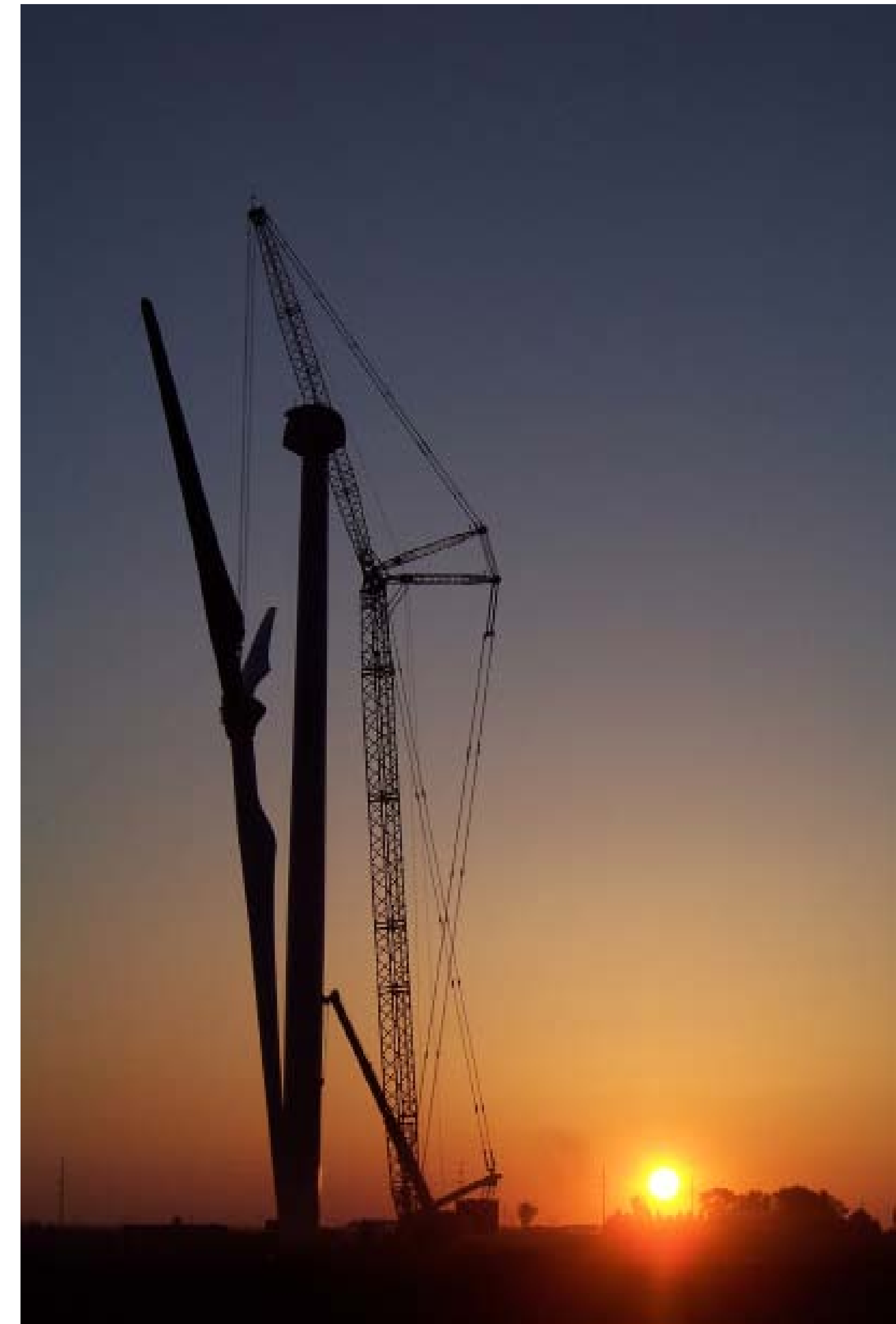
Cranes lift a rotor to be installed on the nacelle at the top of the tower.
