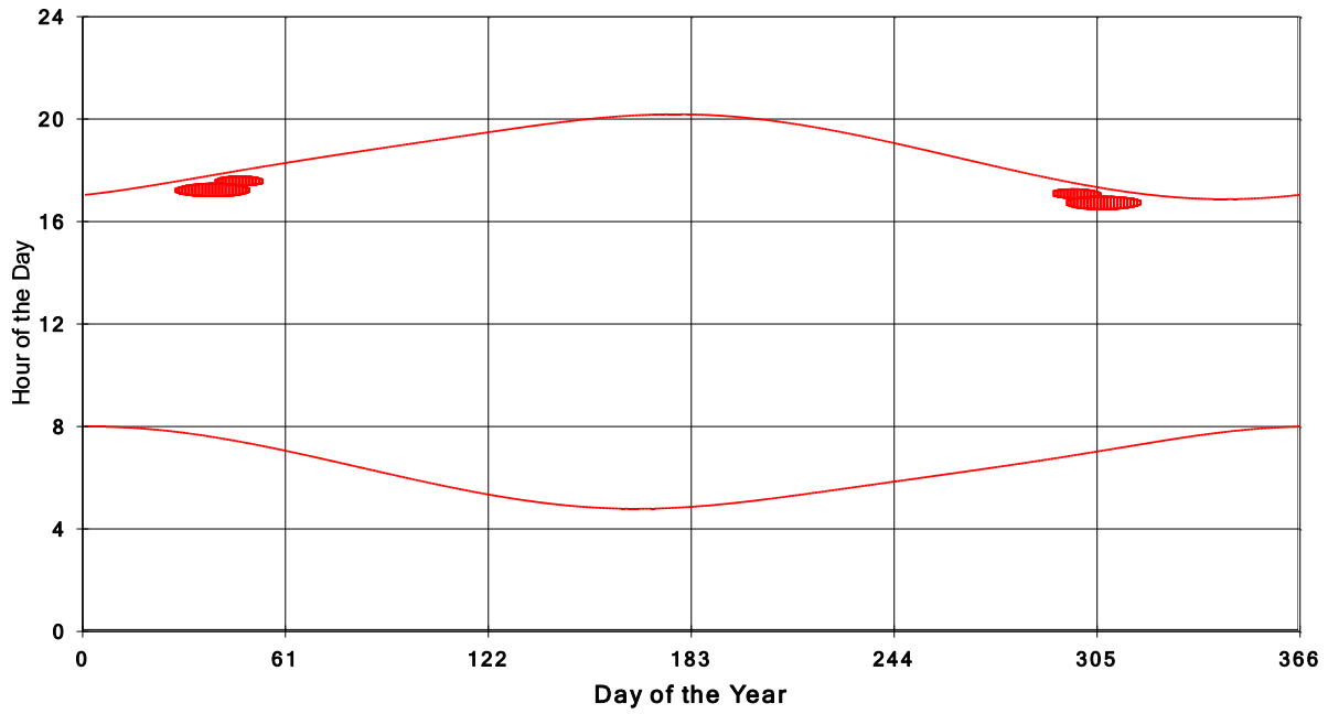
January 31 2013 Flicker with no barns Shadow Times on House 3895, All Windows from All Turbine:
