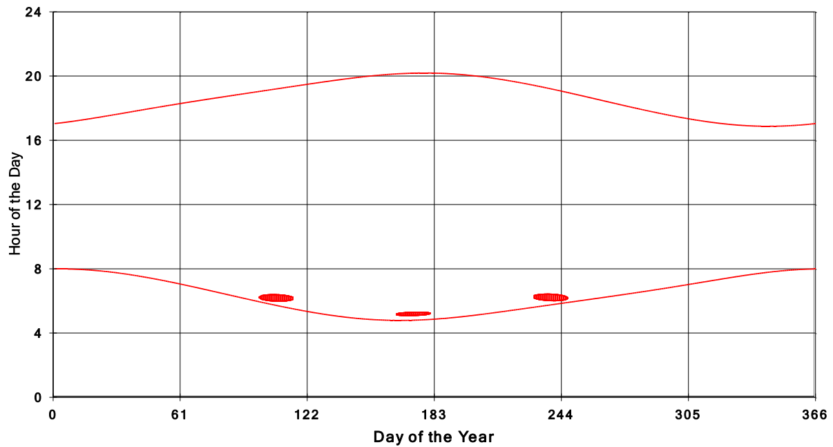
January 31 2013 Flicker with no barns shadow Times on House 3881, All Windows from All Turbine:
