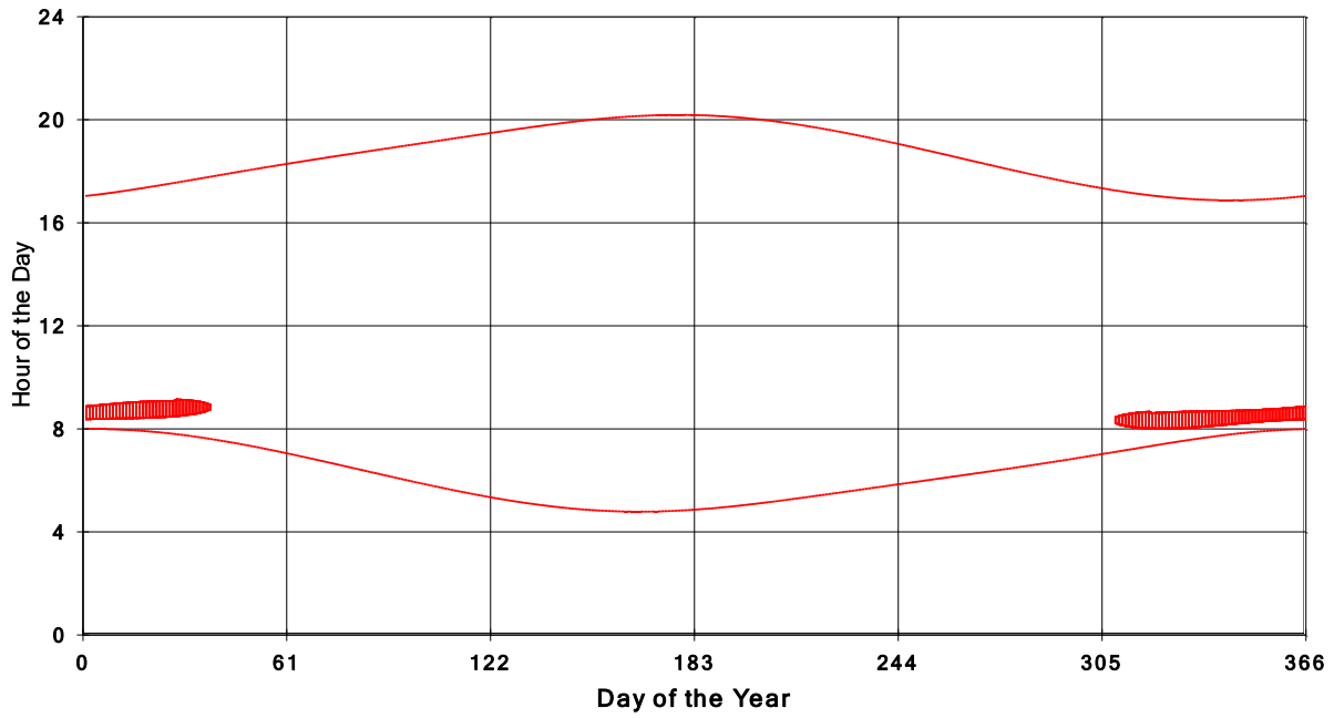
January 31 2013 Flicker with no barns shadow Times on House 3898, All Windows from All Turbine:
