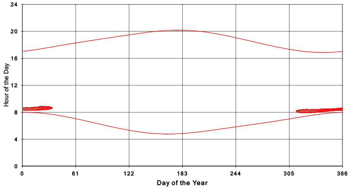
January 31 2013 Flicker with no barns shadow Times on House 3799, All Windows from All Turbine:
