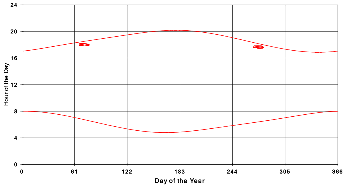
January 31 2013 Flicker with no barns shadow Times on House 3753, All Windows from All Turbine:
