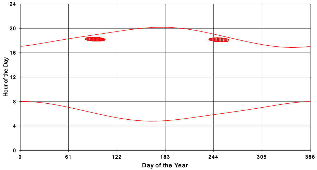
January 31 2013 Flicker with no barns shadow Times on House 3761, All Windows from All Turbine:
