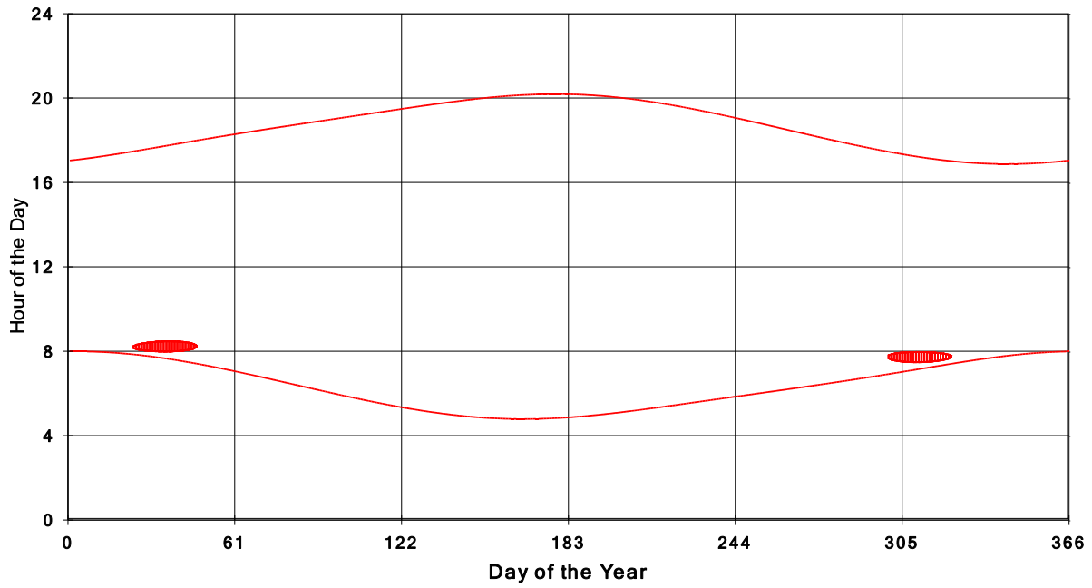
January 31 2013 Flicker with no barns Shadow Times on House 3973, All Windows from All Turbine:
