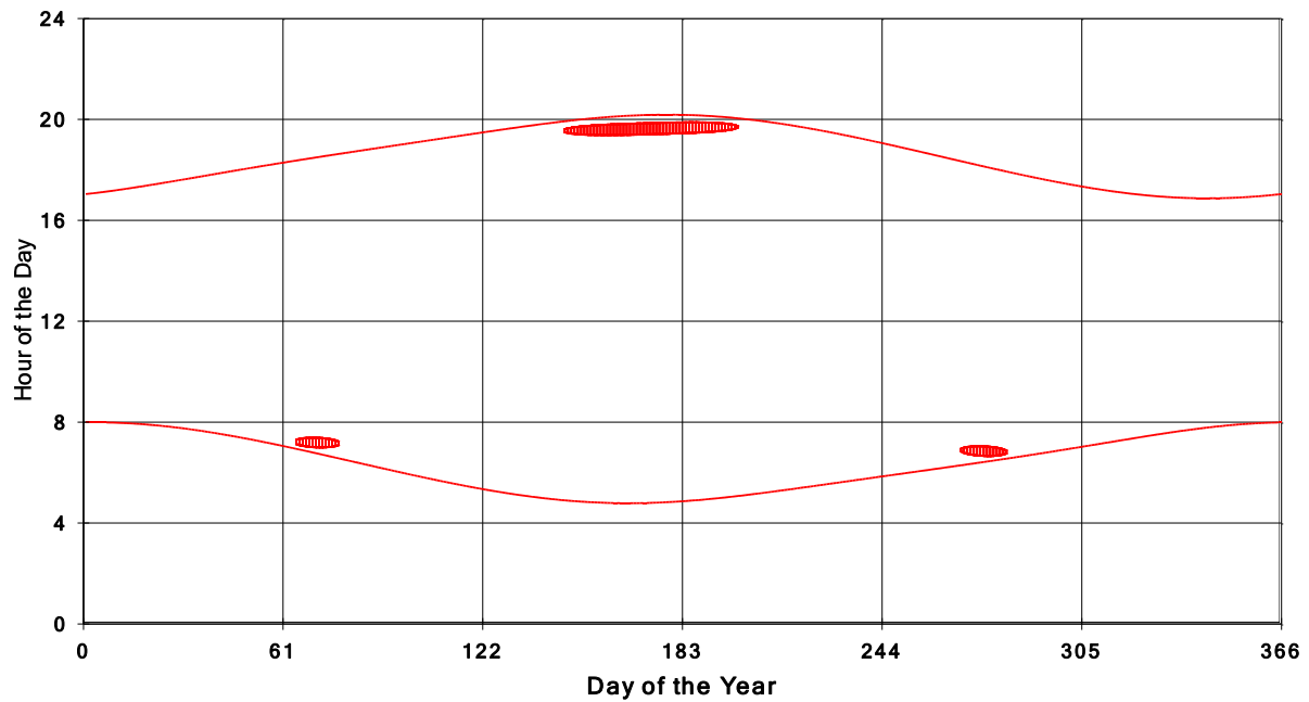
January 31 2013 Flicker with no barns shadow Times on House 3781, All Windows from All Turbine:
