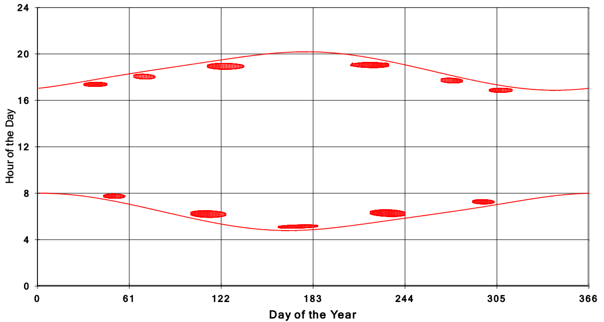
January 31 2013 Flicker with no barns shadow Times on House 3758, All Windows from All Turbine:
