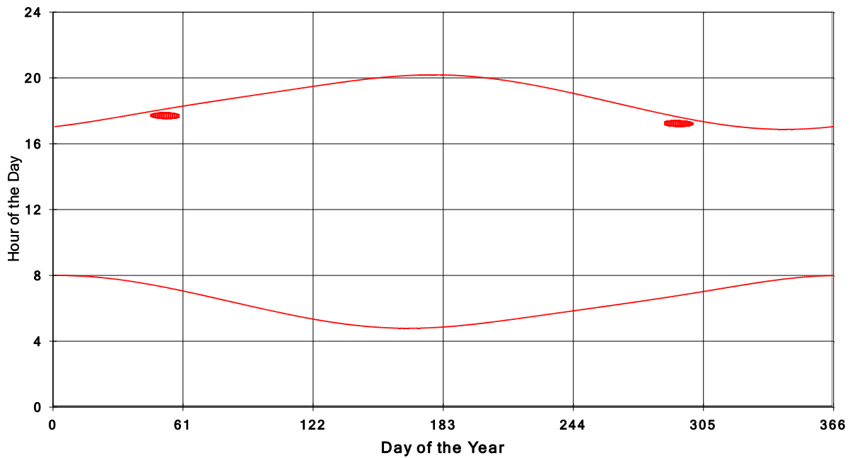
January 31 2013 Flicker with no barns shadow Times on House 3846, All Windows from All Turbine:
