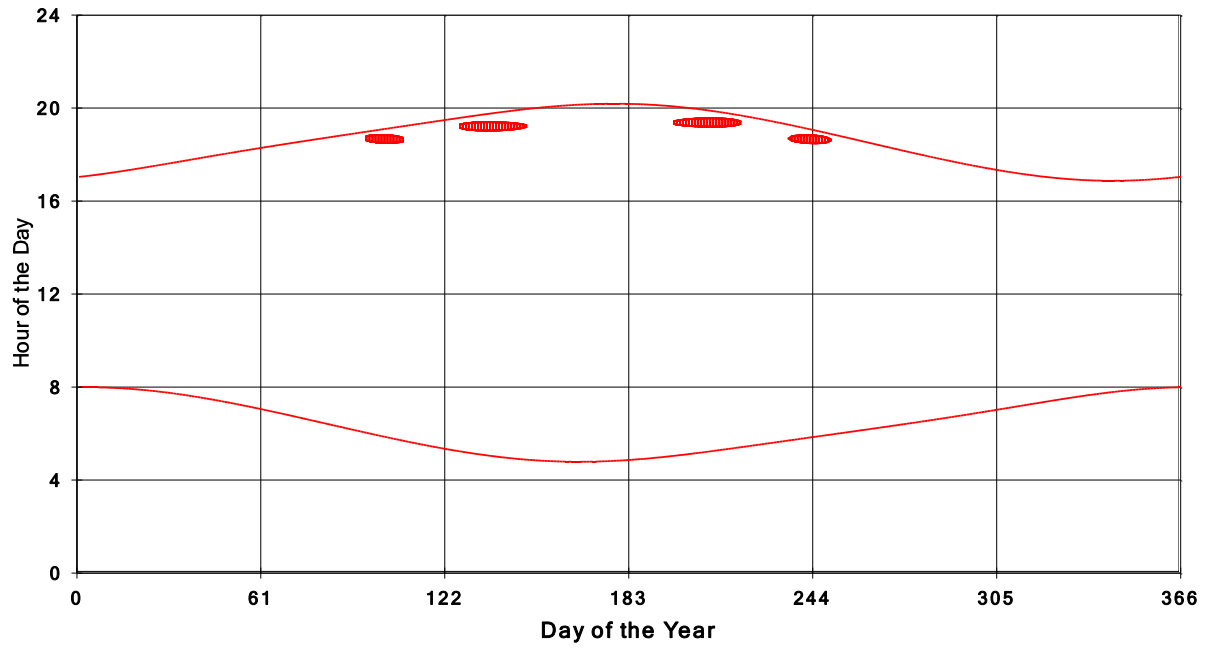
January 31 2013 Flicker with no barns shadow Times on House 3994, All Windows from All Turbine:
