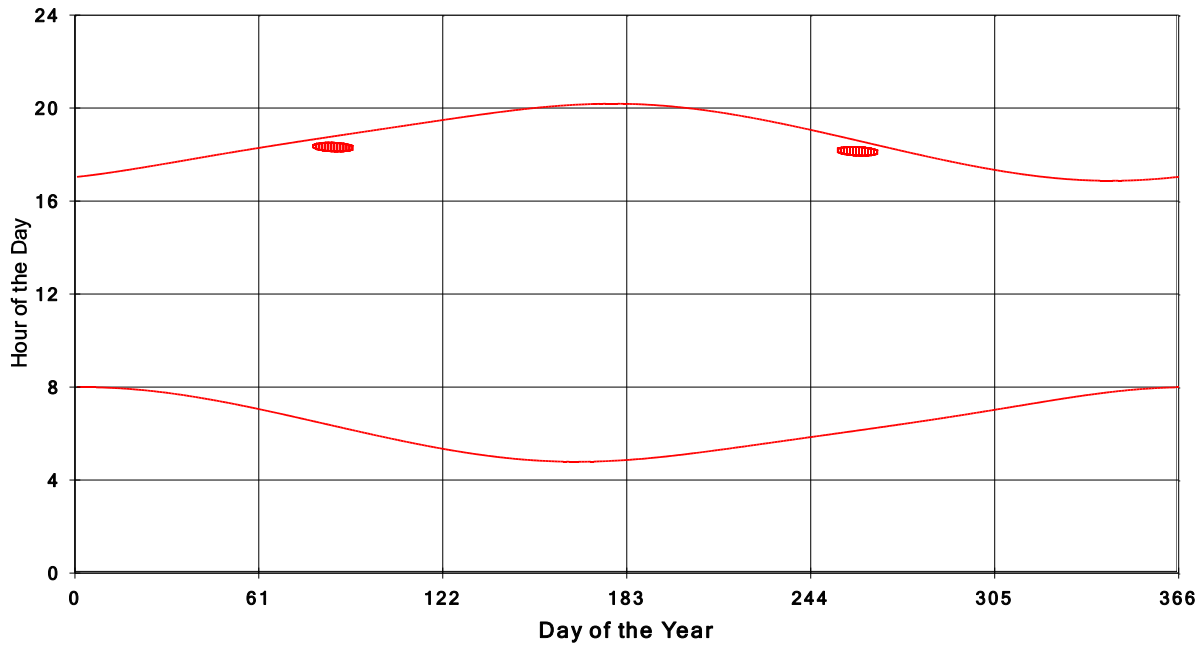
January 31 2013 Flicker with no barns shadow Times on House 3987, All Windows from All Turbine:
