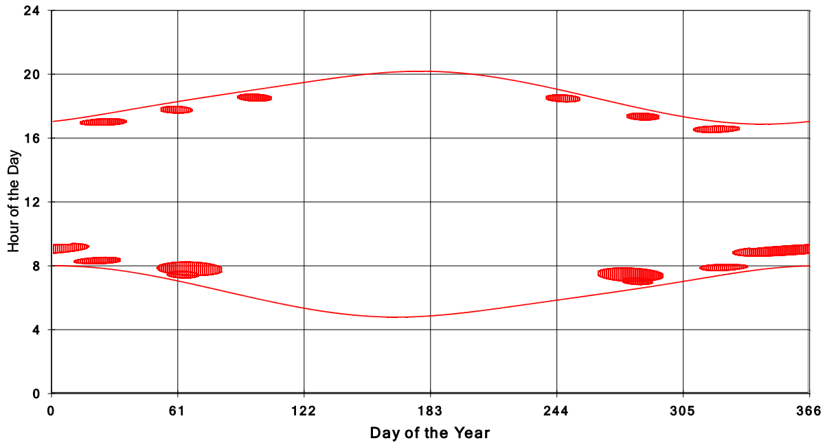
January 31 2013 Flicker with no barns shadow Times on House 3872, All Windows from All Turbine:
