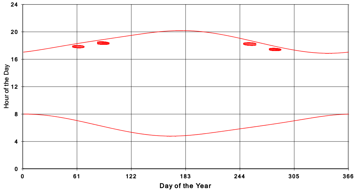
January 31 2013 Flicker with no barns shadow Times on House 3910, All Windows from All Turbine:
