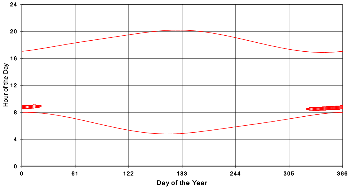
January 31 2013 Flicker with no barns Shadow Times on House 3801, All Windows from All Turbine:
