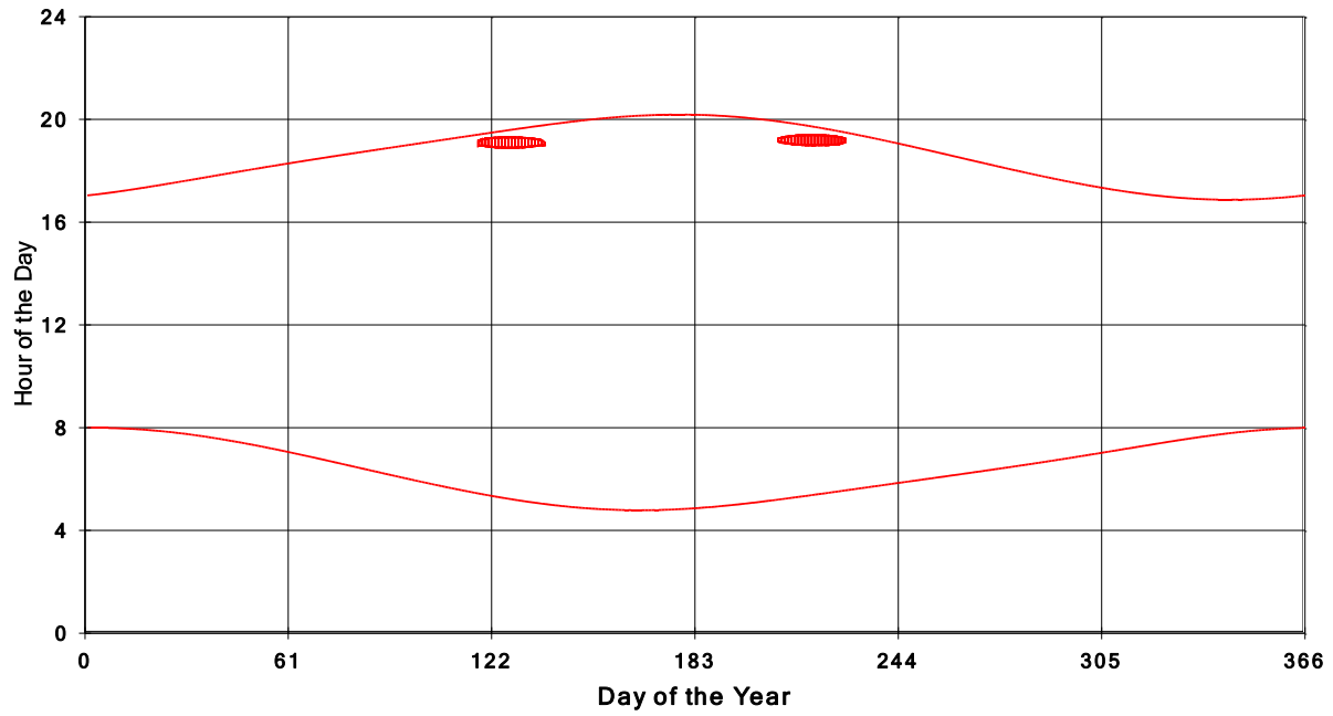
January 31 2013 Flicker with no barns shadow Times on House 3782, All Windows from All Turbine:
