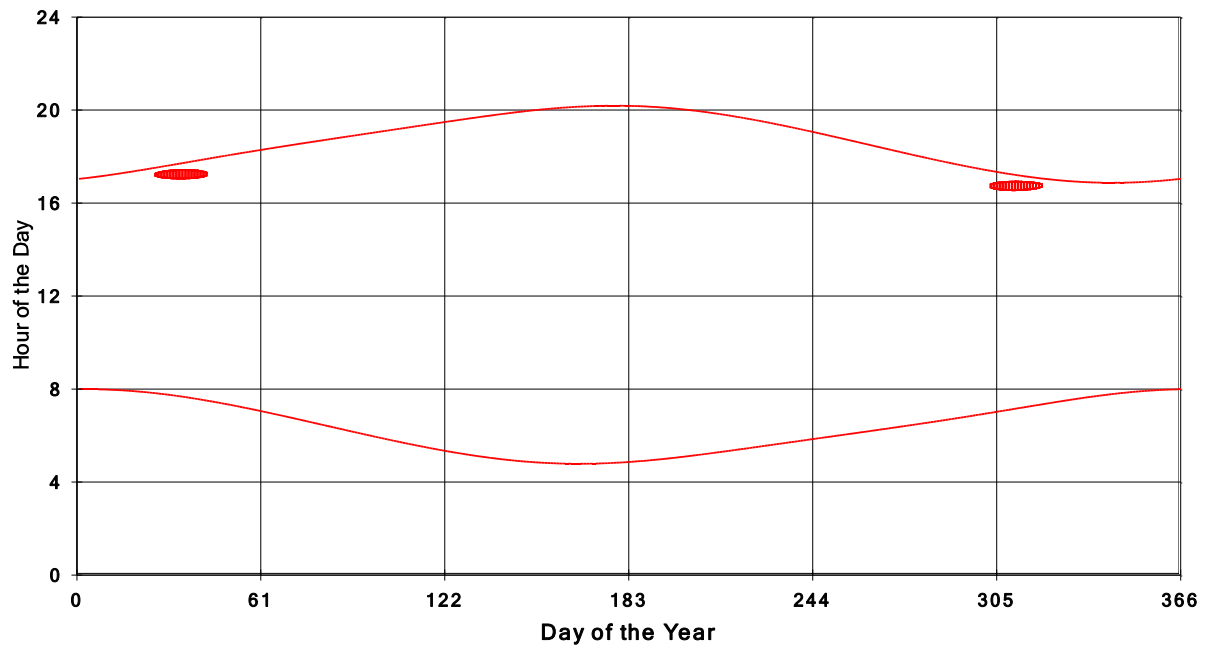
January 31 2013 Flicker with no barns shadow Times on House 3849, All Windows from All Turbine:
