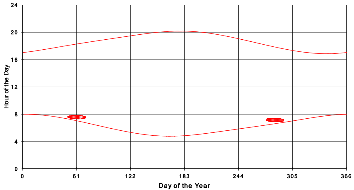
January 31 2013 Flicker with no barns shadow Times on House 3867, All Windows from All Turbine:
