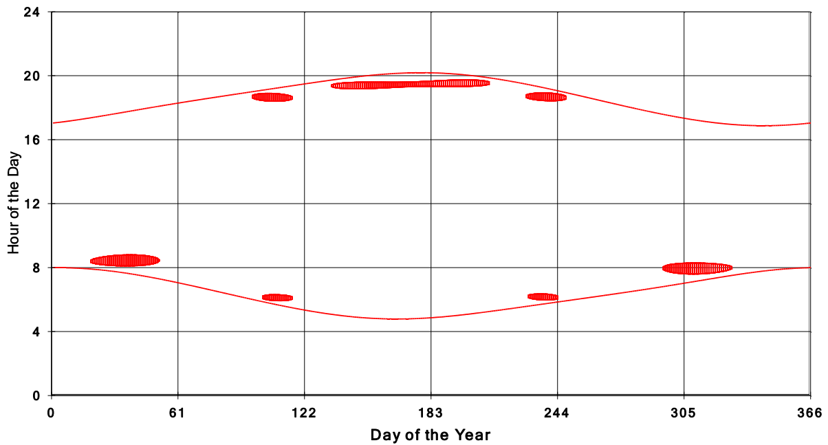
January 31 2013 Flicker with no barns Shadow Times on House 3897, All Windows from All Turbine:
