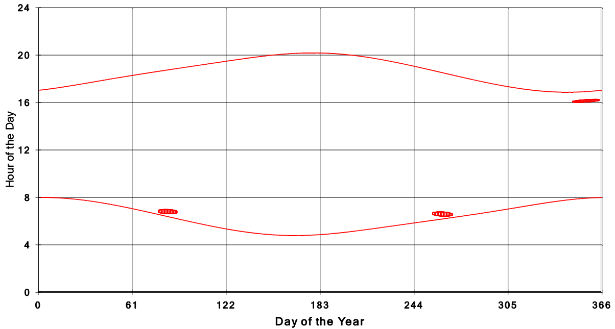
January 31 2013 Flicker with no barns shadow Times on House 3875, All Windows from All Turbine:
