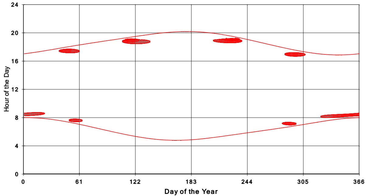
January 31 2013 Flicker with no barns shadow Times on House 3877, All Windows from All Turbine:
