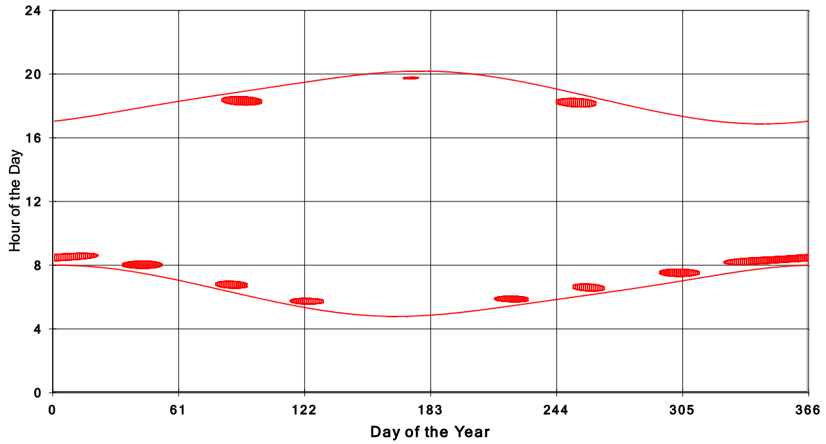
January 31 2013 Flicker with no barns Shadow Times on House 3878, All Windows from All Turbine:
