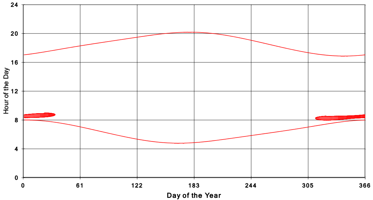
January 31 2013 Flicker with no barns Shadow Times on House 3802, All Windows from All Turbine:
