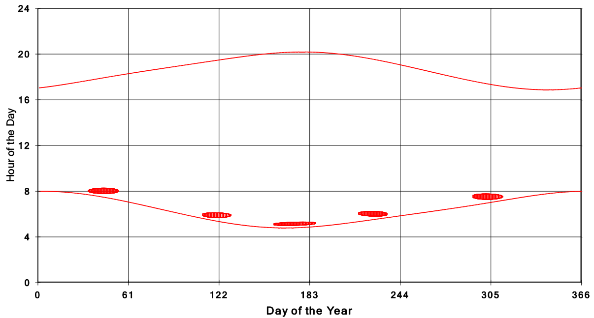
January 31 2013 Flicker with no barns Shadow Times on House 3879, All Windows from All Turbine:
