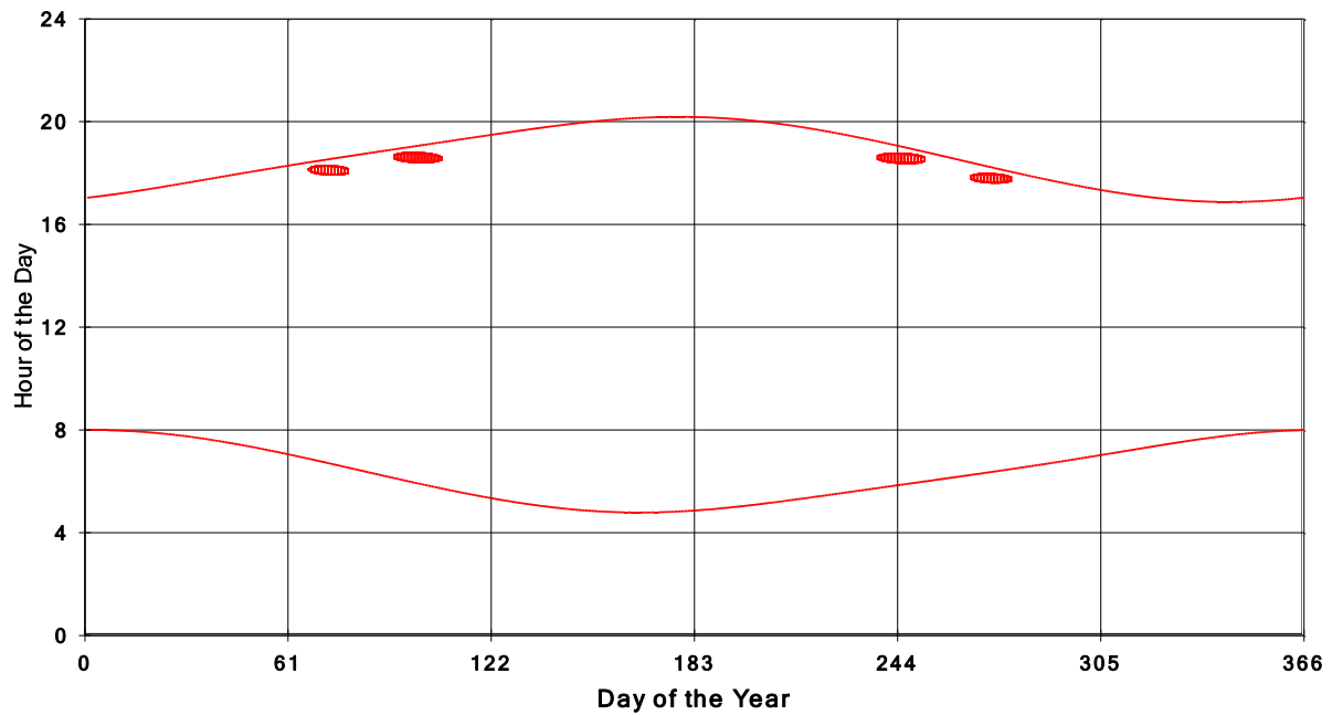
January 31 2013 Flicker with no barns shadow Times on House 3991, All Windows from All Turbine:
