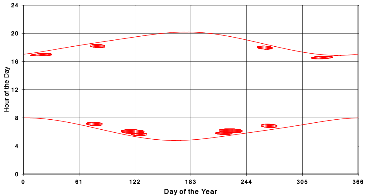
January 31 2013 Flicker with no barns Shadow Times on House 3737, All Windows from All Turbine:
