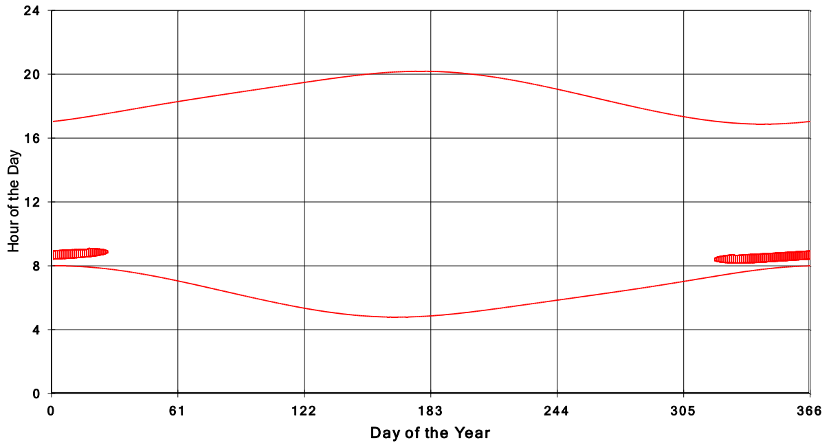
January 31 2013 Flicker with no barns shadow Times on House 3803, All Windows from All Turbine:
