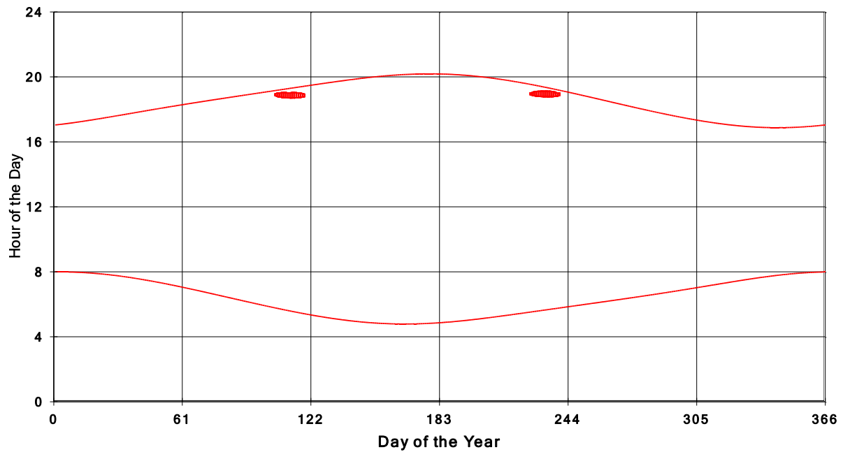
January 31 2013 Flicker with no barns Shadow Times on House 3993, All Windows from All Turbine:
