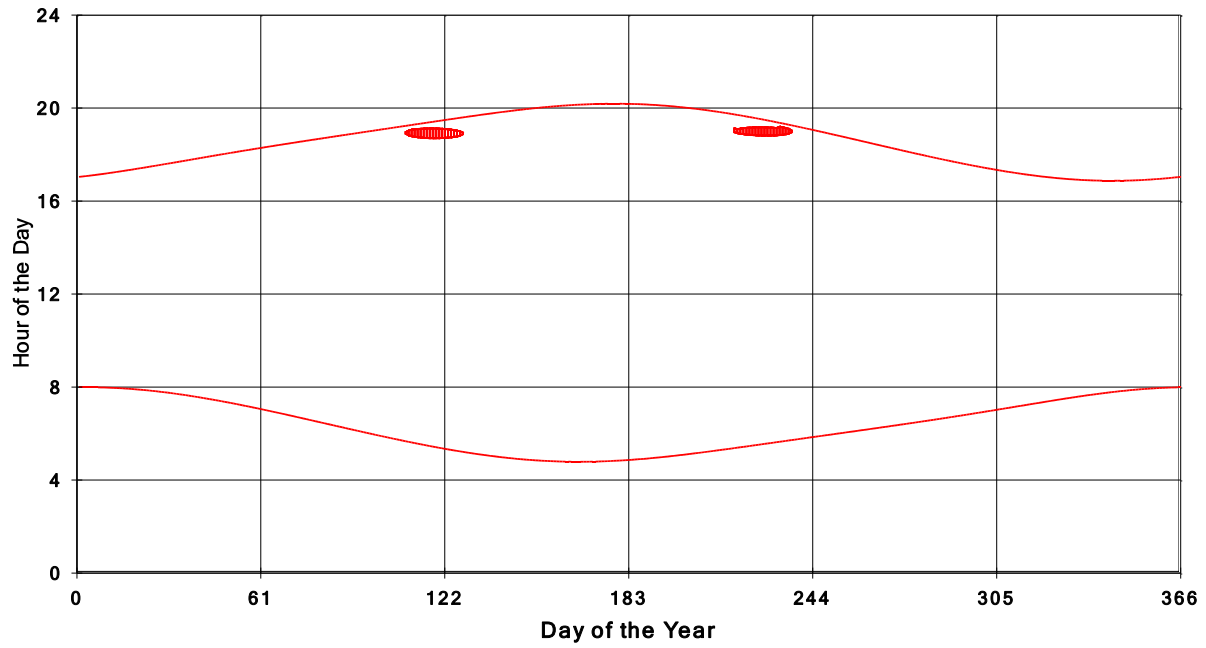
January 31 2013 Flicker with no barns Shadow Times on House 3784, All Windows from All Turbine:
