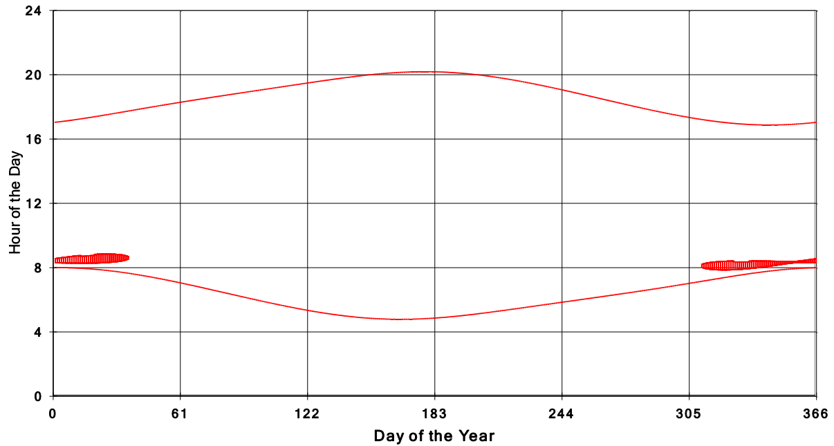
January 31 2013 Flicker with no barns shadow Times on House 3800, All Windows from All Turbine:
