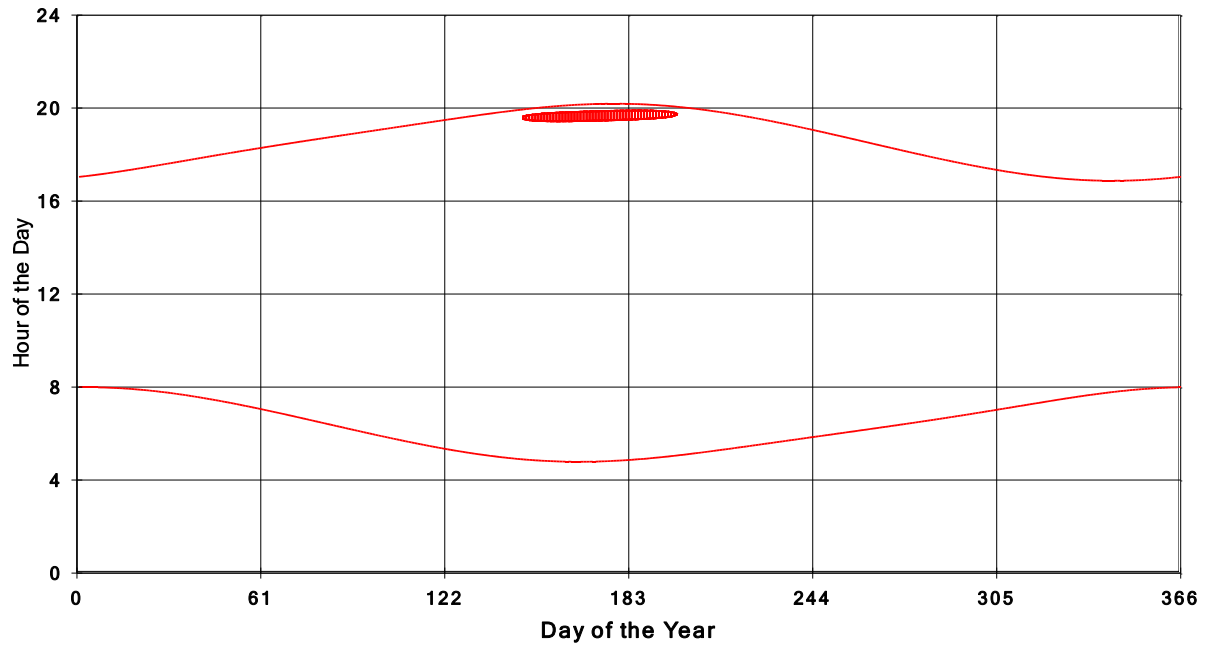
January 31 2013 Flicker with no barns Shadow Times on House 3864, All Windows from All Turbine:
