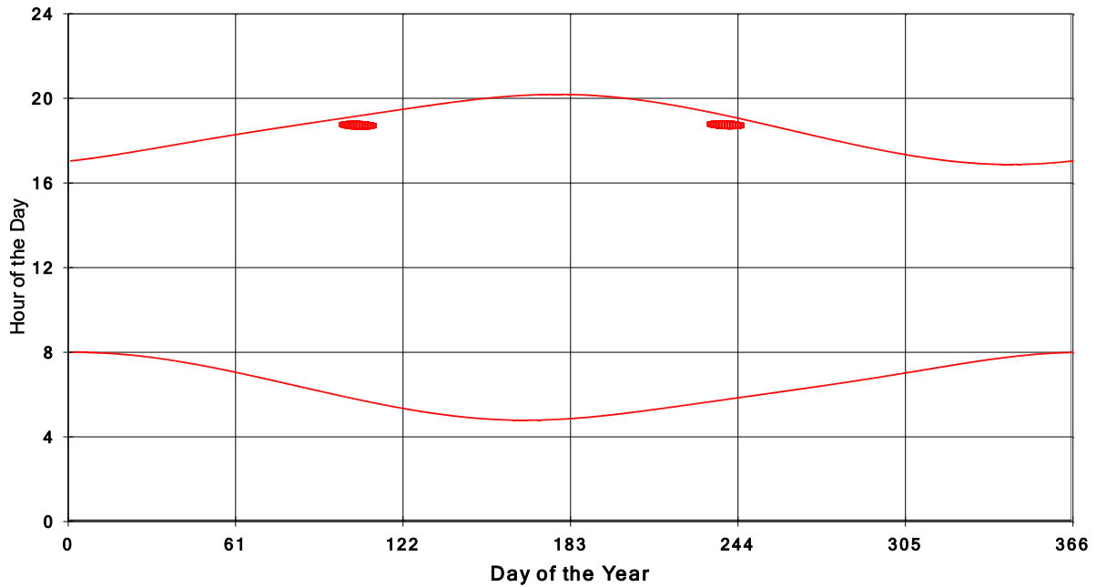
January 31 2013 Flicker with no barns shadow Times on House 3905, All Windows from All Turbine:
