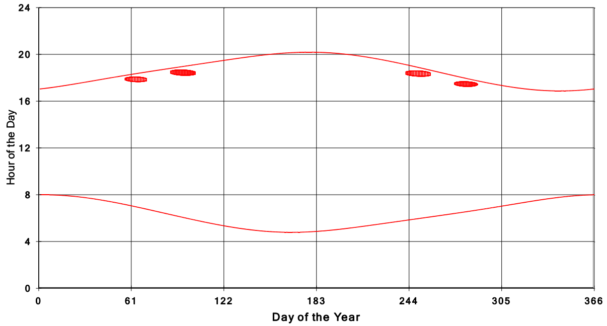
January 31 2013 Flicker with no barns shadow Times on House 3990, All Windows from All Turbine:
