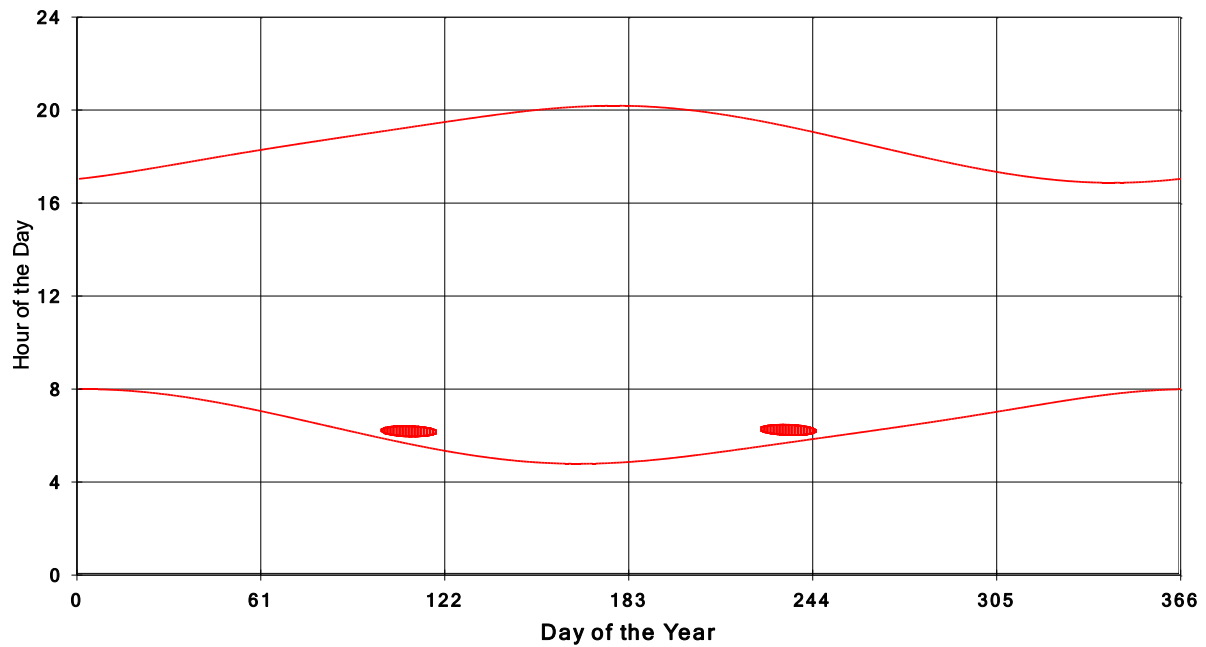
January 31 2013 Flicker with no barns shadow Times on House 3971, All Windows from All Turbine:
