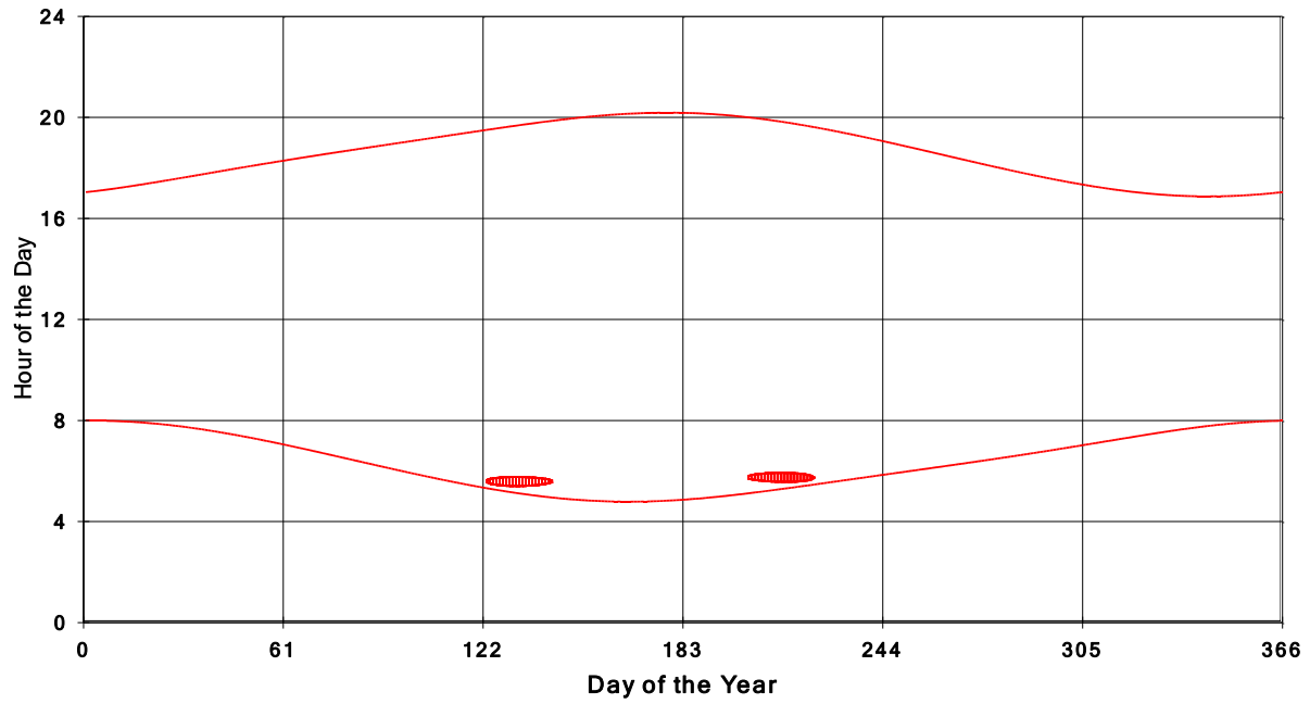
January 31 2013 Flicker with no barns shadow Times on House 3741, All Windows from All Turbine:
