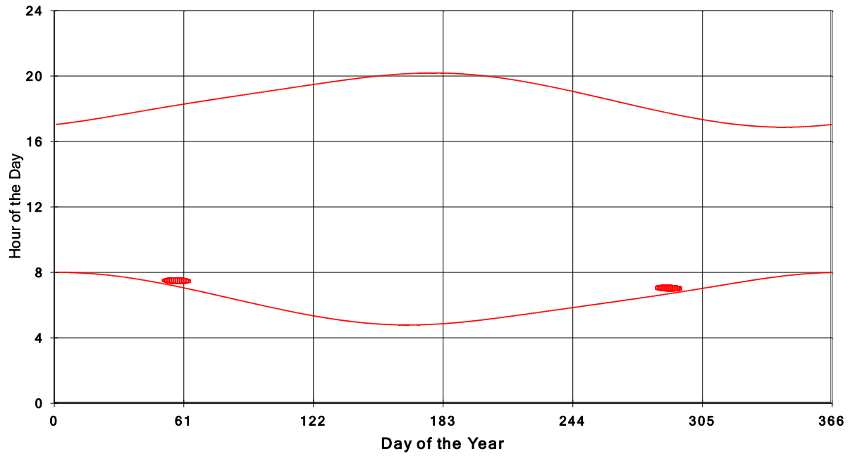
January 31 2013 Flicker with no barns Shadow Times on House 3736, All Windows from All Turbine:
