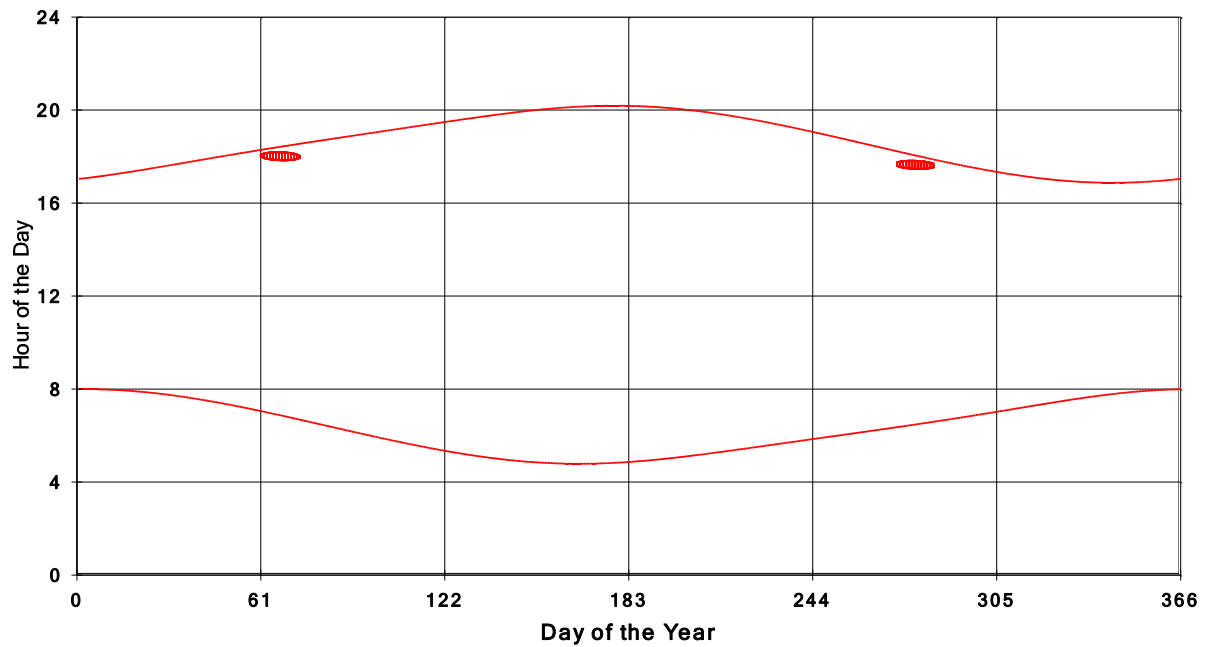
January 31 2013 Flicker with no barns shadow Times on House 3911, All Windows from All Turbine:
