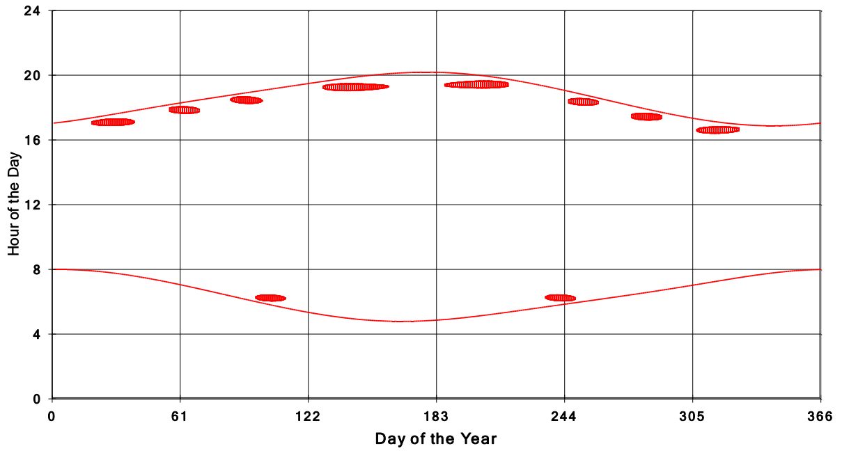
January 31 2013 Flicker with no barns shadow Times on House 3757, All Windows from All Turbine:
