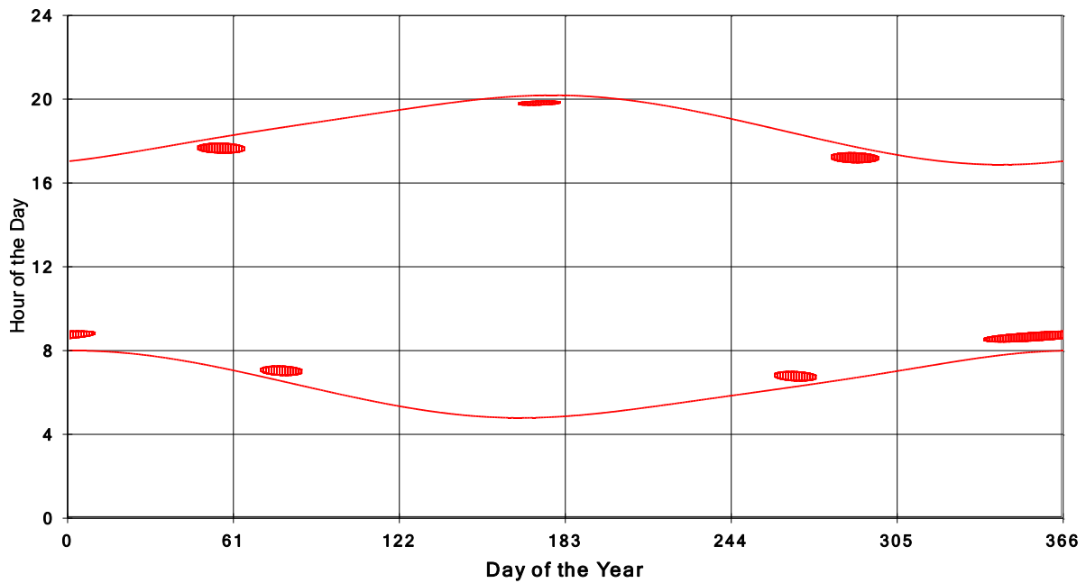
January 31 2013 Flicker with no barns Shadow Times on House 3984, All Windows from All Turbine:
