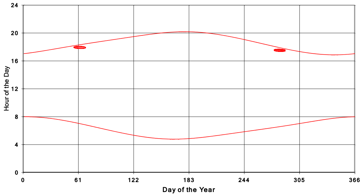
January 31 2013 Flicker with no barns shadow Times on House 4022, All Windows from All Turbine:
