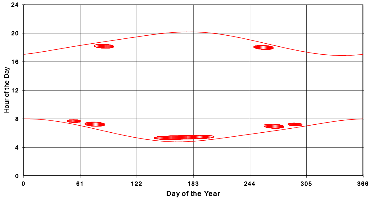
January 31 2013 Flicker with no barns shadow Times on House 3880, All Windows from All Turbine:
