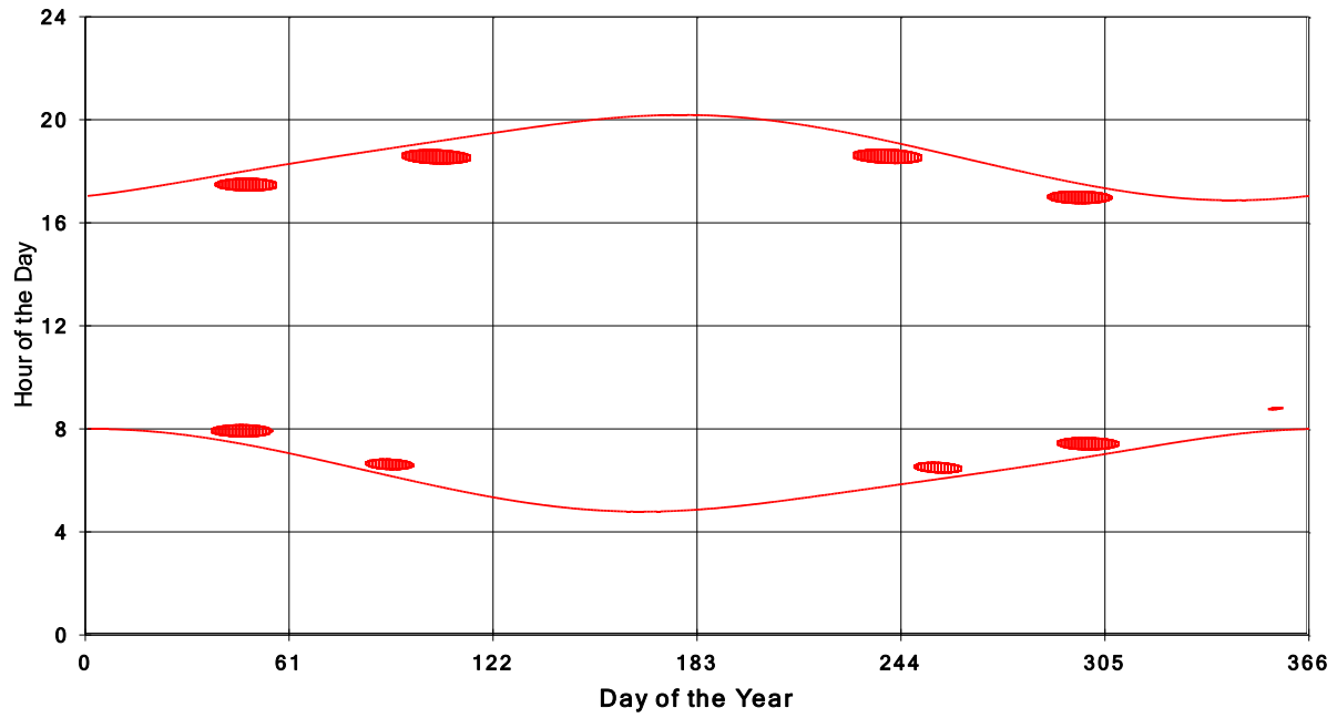
January 31 2013 Flicker with no barns shadow Times on House 3876, All Windows from All Turbine:
