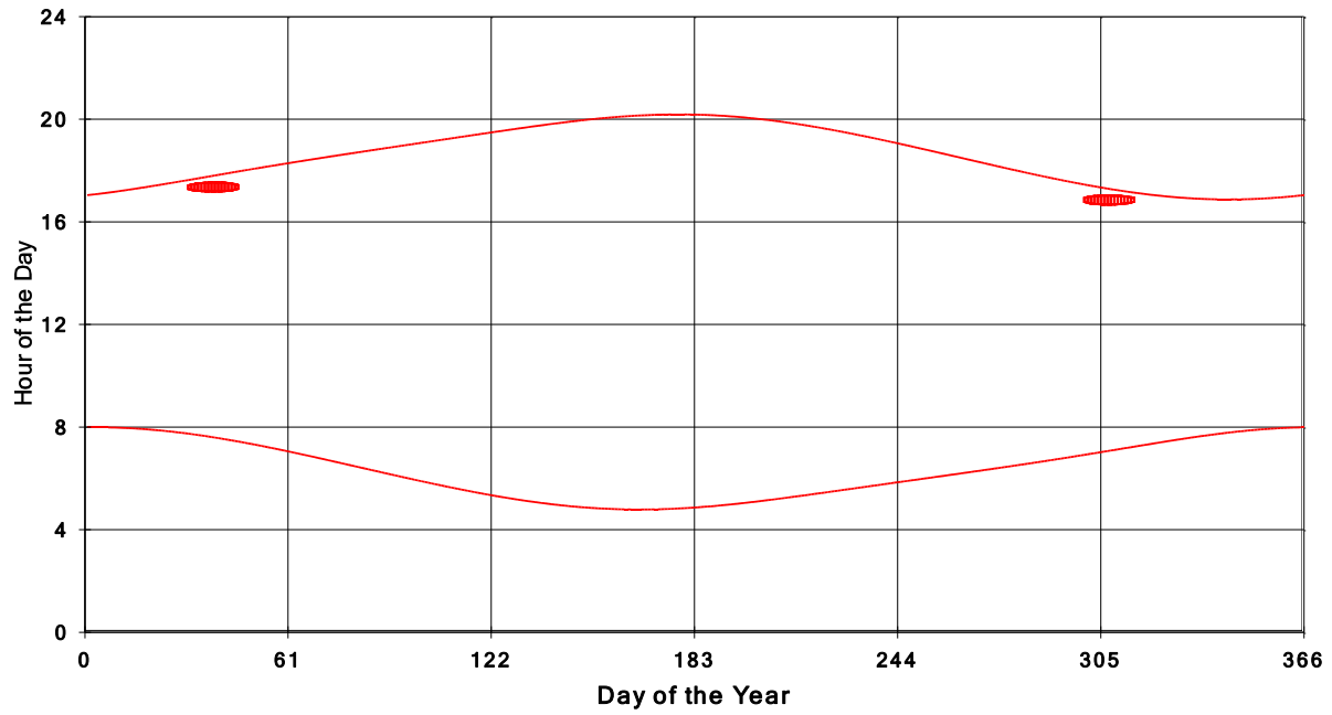
January 31 2013 Flicker with no barns shadow Times on House 3848, All Windows from All Turbine:
