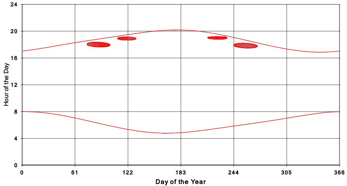
January 31 2013 Flicker with no barns shadow Times on House 4000, All Windows from All Turbine:
