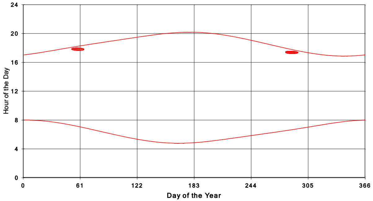
January 31 2013 Flicker with no barns shadow Times on House 3986, All Windows from All Turbine:
