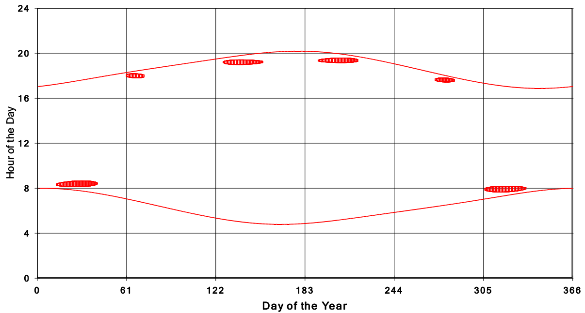
January 31 2013 Flicker with no barns shadow Times on House 4020, All Windows from All Turbine:
